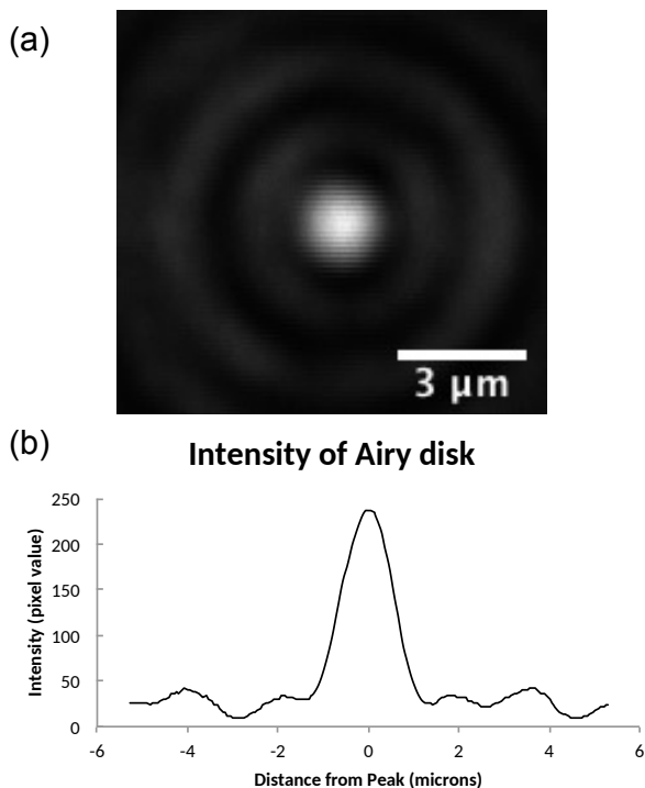
Fig. 3 (a) Airy disk produced by PDMS droplet lens, imaged with Mitutoyo 0.55 NA 100x long working distance objective. (b) Line profile through centre of Airy disk.
