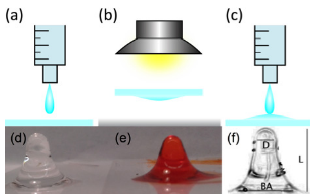
Fig. 1 Steps used to fabricate a droplet lens: (a) droplet of PDMS from syringe, deposited on microscope coverslip; (b) coverslip inverted and suspended above tin foil, 100W incandescent light bulb used to cure PDMS; (c) additional droplet of PDMS deposited on top of the cured drop. Steps (b) and (c) are repeated to increase droplet curvature. In our system, four invert and cure steps were performed. Fabricated lenses used for (d) trapping and (e) imaging are shown, along with (f) a schematic of how lenses were measured.
