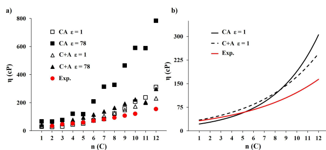
Fig. 9 a) Viscosity for C_n\text{mimNTf}_2 ( n = 1 to 12 ) series with \epsilon = 1 and 78 , and both models, including experimental data. b) CA and C+A models with \epsilon = 1 , and experimental data
