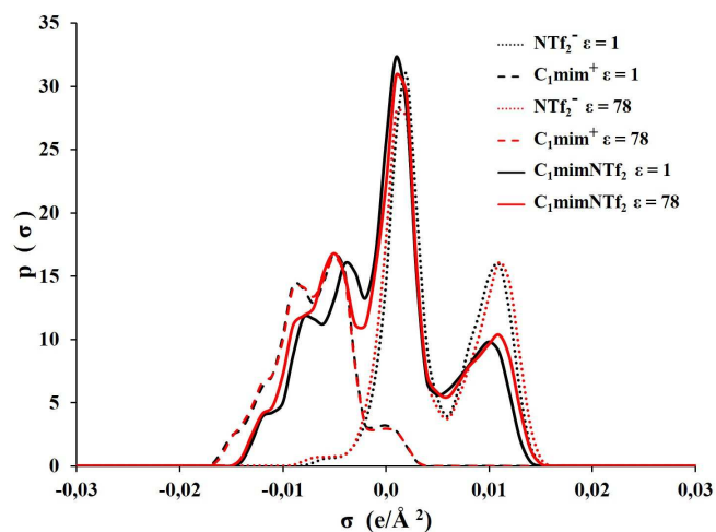
Fig. 3 \sigma -profiles of the C_1\text{mimNTf}_2 represented as both models with \epsilon = 1 (black line) and the highest value considered in this work for dielectric constant: \epsilon = 78 (red line)
