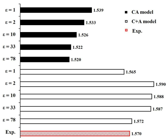
Fig. 8 Density for C_1\text{mimNTf}_2 modeled with different values of dielectric constant, including experimental data in \text{g.mL}^{-1}
