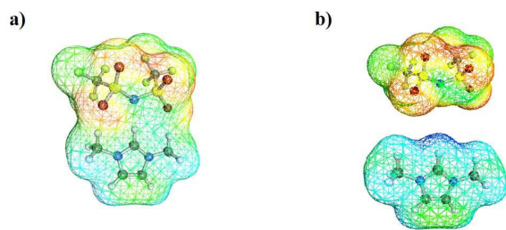
Fig. 2 a) lon-pair model and b) independent counterions model
