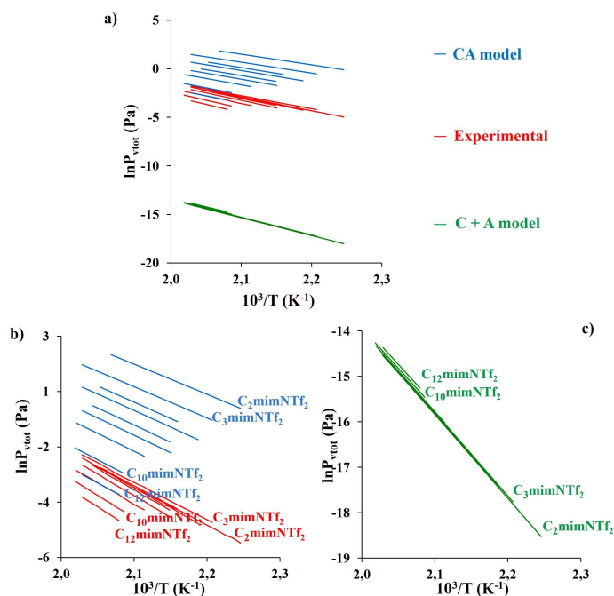
Fig. 6 a) \ln P_{vot} as function of the temperature for C n mimNTf 2 ( n = 2, 3, 4, 5, 6, 7, 8, 10 and 12 ) series with CA and C+A models, including experimental data. b) \ln P_{vot} as function of the temperature for C n mimNTf 2 ( n = 2, 3, 4, 5, 6, 7, 8, 10 and 12 ) series with CA model and experimental data. c) \ln P_{vot} as function of the temperature for C n mimNTf 2 ( n = 2, 3, 4, 5, 6, 7, 8, 10 and 12 ) series C+A model
