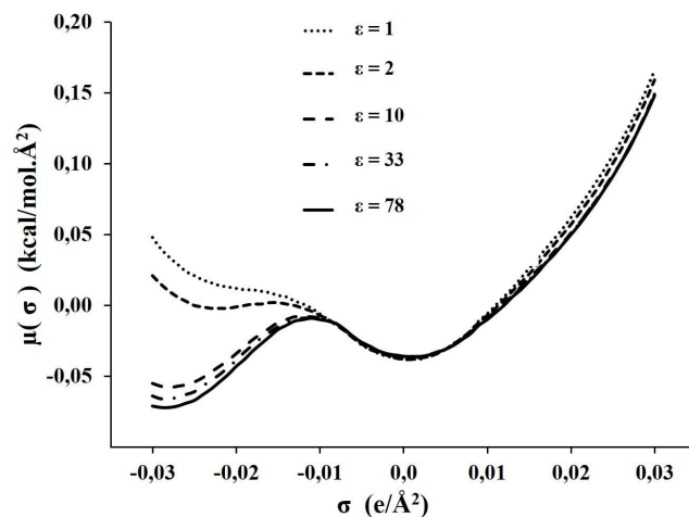
Fig. 4 \sigma -potentials of the C_1\text{mimNTf}_2 modeled as CA model with different values for dielectric constants: 1, 2, 10, 33, and 78
