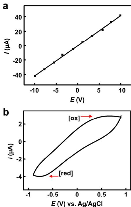
Figure 6. Electrical and electrochemical behavior of biocatalytically surface-grown polypyrrole films. a) I-V characteristic of a polypyrrole film obtained by two contact measurement. b) Redox wave for a polypyrrole film in PBS, at a scan rate of 100 \text{ mV s}^{-1} , showing oxidation and reduction reactions.
