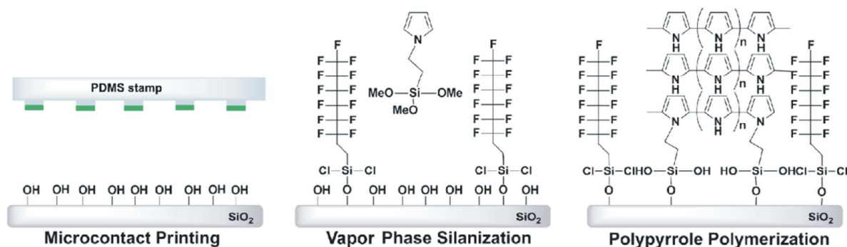
Figure 1. Site-selective deposition of biocatalytically produced polypyrrole microelectrodes on insulating SiO 2 surfaces. Schematics of the procedure that include from left to right: \mu CP of fluorosilane FDTES, backfilling with pyrrole-silane and polymerization of pyrrole.
