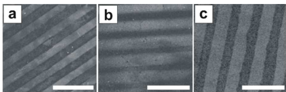
Figure 3. The versatility of the site-selective deposition of biocatalytically produced polypyrrole microelectrodes was validated using various pattern dimensions. Representative SEM images of a) 20- \mu\text{m} -width lines with 20- \mu\text{m} pitch (scale bar = 100 \mu\text{m} ), b) 5- \mu\text{m} -width lines with 1- \mu\text{m} pitch (scale bar = 15 \mu\text{m} ), and c) 5- \mu\text{m} -width lines with 5- \mu\text{m} pitch (scale bar = 20 \mu\text{m} ).
