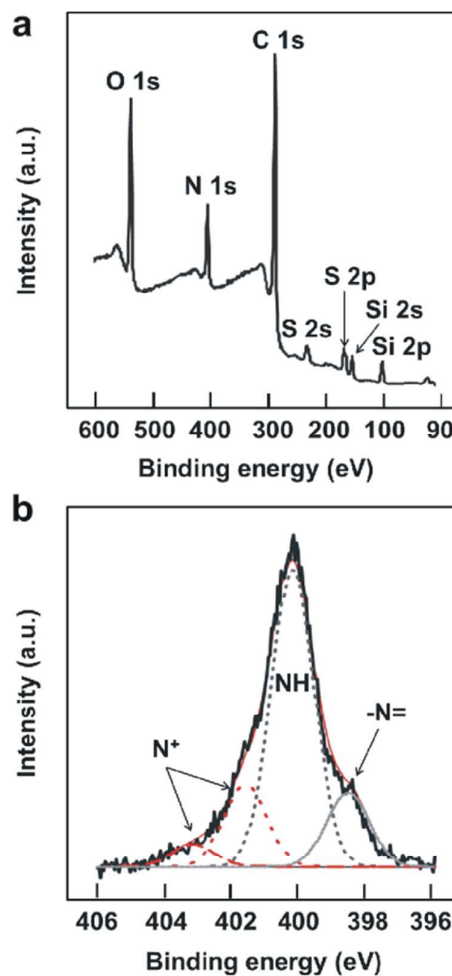
Figure 5. XPS analysis of biocatalytically synthesized polypyrrole thin films. a) Wide-scan spectrum, and b) N 1s core-level deconvolution showing the \text{N}^+ components of the doped polypyrrole structure.
