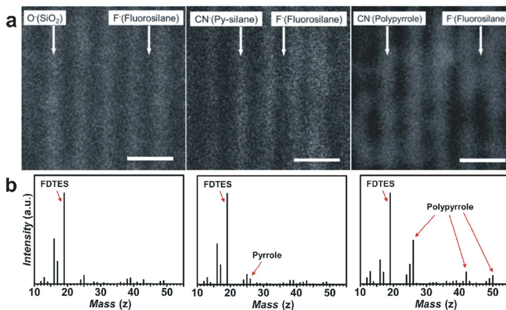
Figure 2. Site-selective deposition of biocatalytically produced polypyrrole microelectrodes on insulating SiO 2 surfaces. a) Representative ToF-SIMS images of the indicated ions, obtained after each fabrication step. Scale bar = 15 \mu m. b) Representative ToF-SIMS spectra obtained after each fabrication step and highlighting the material of which the samples comprised.
