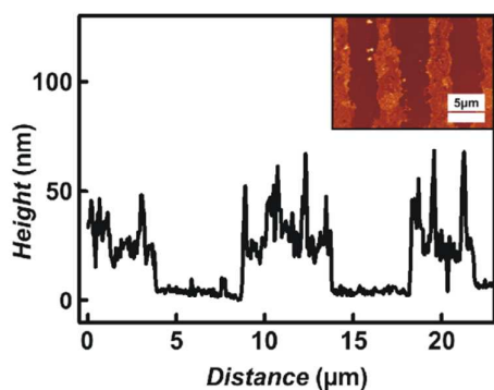
Figure 4. AFM profile of biocatalytically produced polypyrrole microelectrodes. Polypyrrole microelectrodes showed an average thickness of 31 nm. Inset shows corresponding AFM topographical image.
