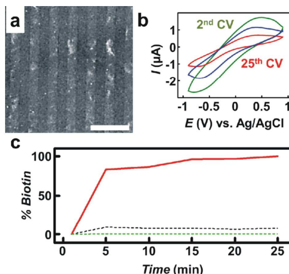
Figure 7. Electrically controlled release of biotin from biocatalytically produced polypyrrole microelectrodes. a) Representative SEM image of 20- \mu\text{m} -width lines of site-selective biocatalytically surface-grown polypyrrole in the presence of biotin (scale bar = 100 \mu\text{m} ). b) Series of CVs (at 2 scans in green, 8 scans in blue and 25 scans in red) performed on the biotin-modified polypyrrole electrodes, showing the reduction in the electro-activity caused by biotin release. c) Plot of the evolution of the characteristic peak area fragment at m/z = 245.09 of biotin, obtained from HPLC-MS analysis of the electrolyte solution at various time-points during the reduction step (solid red line), oxidation step (dashed green line), and without electrical stimulation (dashed black line). Results show that biotin release caused by passive ion exchange or during the oxidation step is minimal.
