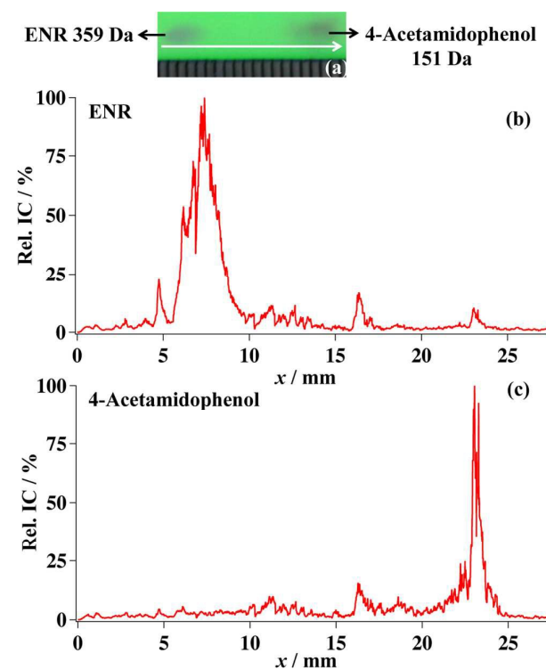
Figure 8. ESTASI-MS line-scan of a drug mixture on a silica gel TLC plate with silane modification. The mixture contains ENR ( 1.4 \text{ nmole} ) and 4-acetamidophenol ( 3.3 \text{ nmole} ) (a) an optical image of the dried sample spots on the TLC plate. (b) and (c) Rel. IC/% chromatography of ENR and 4-acetamidophenol, respectively.
