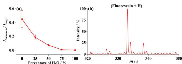
Figure 2. Extraction solvent optimization and detection limit of fluorescein on HPRP C18 plate. (a) Optimization of the extraction solvent (water and methanol mixture with 1% acetic acid). I_{\text{fluorescein}} : intensity of singly protonated fluorescein at m/z = 333.3 ; I_{\text{AngI}} : intensity of three-protonated angiotensin I at m/z = 432.9 . (b) Mass spectrum of fluorescein detected by ESTASI-MS from the HPRP C18 plate with 1% acetic acid, 75% methanol and 24% \text{H}_2\text{O} as the extraction solvent under a flow rate of 1 \mu\text{L min}^{-1} . Sample on TLC: fluorescein (1 \mu\text{L} , 30 \mu\text{M} aqueous solution) developed by the mobile solution of methanol and tetrahydrofuran (60: 40 v/v) with 100 mM ammonium acetate.
