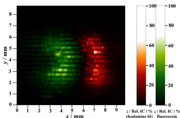
Figure 4. 2D TLC-ESTASI-MSI of rhodamine 6G and fluorescein spots in Figure 3(a). Rel. IC/% of each dye was plotted with respect to the position on the TLC plate and represented individually as the z -axis in a form of green (fluorescein) or red (rhodamine 6G) colour gradient.
