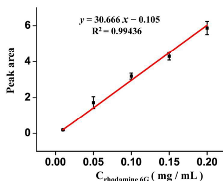
Figure 5. Calibration plot of integrated peak area of Rel. IC chromatography of rhodamine 6G from TLC-ESTASI-MS versus its concentration. Each sample spot was developed from 1 \mu\text{L} of rhodamine 6G solutions with different concentrations, ranging from 0.01 mg/mL to 0.2 mg/mL on a HPRP C18 plate. The ESTASI was performed with the extraction solvent of Ang I (3 \mu\text{M} ) in 1% acetic acid, 75% methanol and 24% water under the flow rate of 1 \mu\text{L min}^{-1} .
