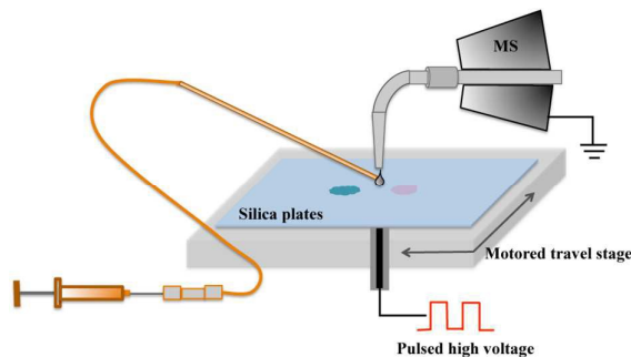
Figure 1. Schematic representation of the setup used for TLC-ESTASI-MS.
