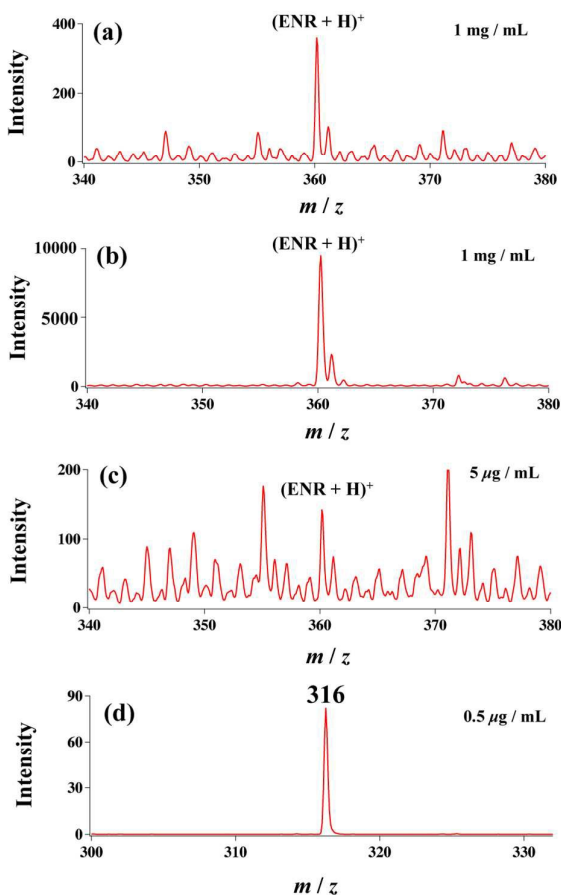
Figure 7. ESTASI-MS spectra of sample spots from: (a) 1 \mu\text{L} , 1 \text{ mg/mL} ENR aqueous solution developed on a silica gel TLC plate, (b) 1 \mu\text{L} , 1 \text{ mg/mL} ENR aqueous solution developed on a silica gel TLC plate with silane modification, and (c) 1 \mu\text{L} 5 \mu\text{g/mL} ENR solution developed on a silica gel TLC plate with silane modification. (d) ESTASI-MS SRM spectrum of a sample spot from 1 \mu\text{L} , 0.5 \mu\text{g/mL} ENR aqueous solution developed on a silica gel TLC plate followed with silane modification. ESTASI-MS was performed with the extraction solvent of 75% water, 24% methanol and 1% acetic acid. Normalized collision energy of CID: 25; isolation width of precursor ion: \pm 1 ; SRM range: m/z 316 \pm 16 .
