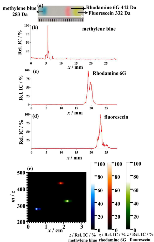
Figure 3. ESTASI-MS line scan of a dye mixture separated on a HPRP C18 plate. The dye mixture contains methylene blue (1.7 nmole), rhodamine 6G (1 nmole) and fluorescein (1.5 nmole). (a) Optical image of the dried samples. (b), (c) and (d) normalized relative ion current (Rel. IC/%) chromatography of methylene blue, rhodamine 6G and fluorescein, respectively. (e) 3D TLC-ESTASI MS map of the three dyes. Rel. IC of each dye was calculated by dividing the IC of singly protonated sample molecule by that of the triply protonated Ang I, and then normalized, respectively.
