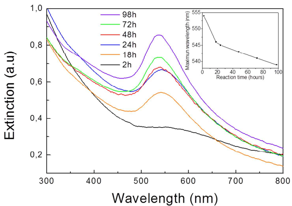
Figure 2. UV-Vis extinction spectra of a sample taken from the reaction between \text{HAuCl}_4 \cdot 3\text{H}_2\text{O} and preformed Pt cubeoctahedra at different reaction times. Inset: plot of maximum wavelength of the SPR band vs. reaction time 254x190mm (96 x 96 DPI)
