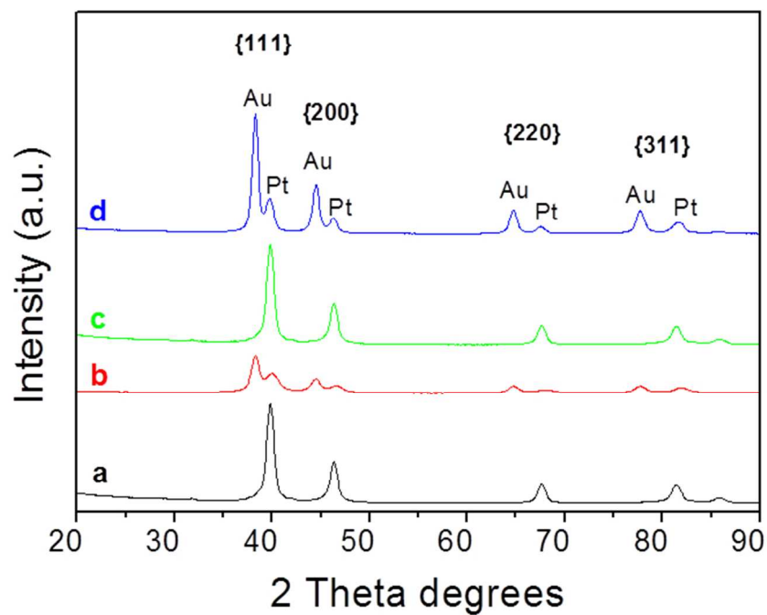
Figure 4. X-ray diffraction patterns of (a) Pt cubeoctahedra, (b) cubeoctahedrally-derived HDs, (c) Pt octahedra and (d) octahedrally-derived HDs.
