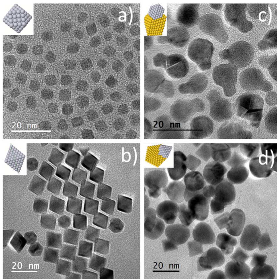
Figure 1. Representative TEM images of (a) Pt cubeoctahedra, (b) Pt octahedra, (c) cubeoctahedrally-derived HDs and (d) octahedrally-derived HDs 186x187mm (96 x 96 DPI)
