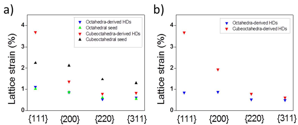
Figure 5. Estimated bulk lattice strain for different crystallographic planes of Pt nanocrystals and their corresponding HDs. (a) Pt phases and (b) Au phases. 254x113mm (96 x 96 DPI)
