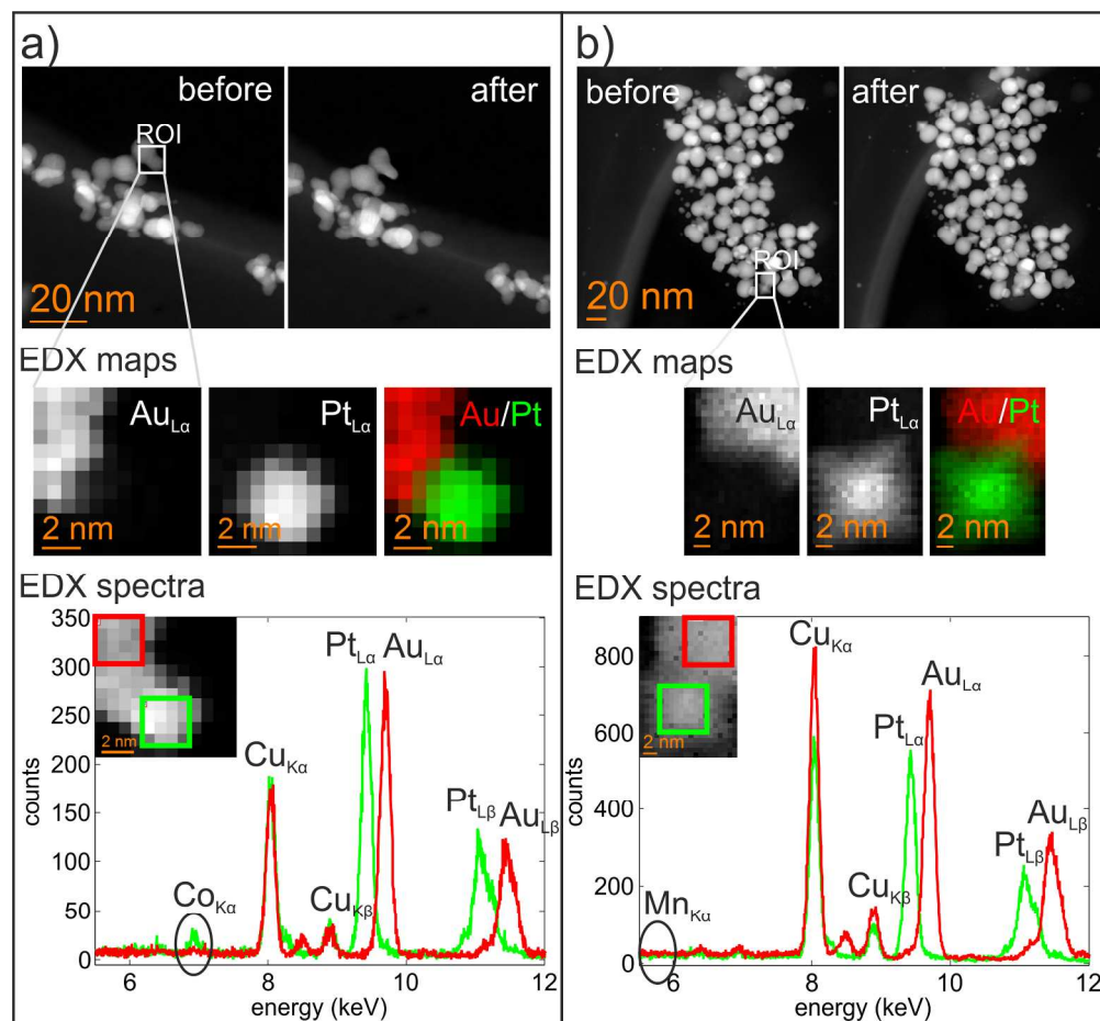
Figure 7. HAADF images before and after STEM-EDX analysis (top) combined with EDX elemental maps (middle) and EDX spectra (bottom) for cubeoctahedrally-derived HDs (a) and octahedrally-derived HDs (b). The elemental maps of Au and Pt are taken from the regions as marked in the HAADF images, while the spectra are extracted from the regions shown in the inset of the EDX spectra.
