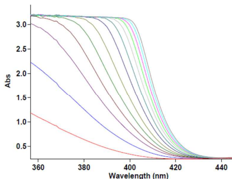
Fig. 2. Absorption changes versus wavelength for the reaction Between 1 ( 10^{-2} \text{ M} ), 2 ( 10^{-2} \text{ M} ) and 3 ( 10^{-2} \text{ M} ) in formic acid for generation of product 4
