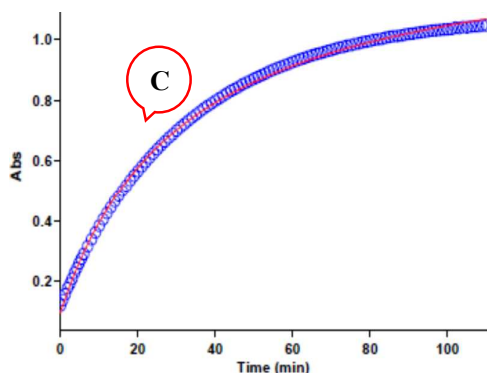
Fig. 4-C. Plot of absorbance versus time at 420 nm for the reaction between 1 ( 10^{-2} mol.L ^{-1} ), 2 ( 10^{-3} mol.L ^{-1} ) and 3 ( 10^{-2} mol.L ^{-1} ) in formic acid, dotted line is experimental values, and the solid line is fit curve
