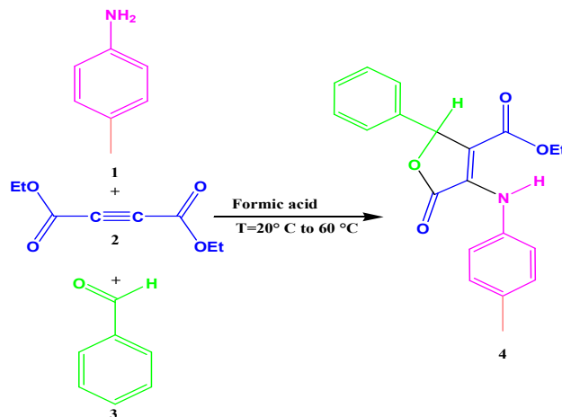
Fig. 1: The three-component synthesis of furan-2(5H)-ones [38]
