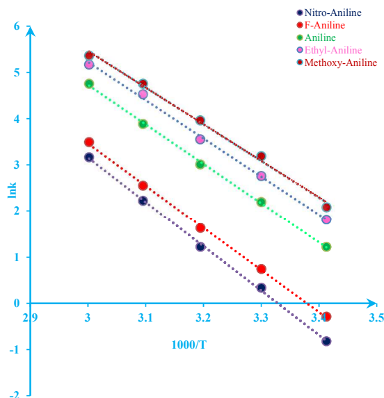
Fig. 5. Dependence of second order ( \ln k_{\text{ovr}} = \ln k_1 ) on reciprocal temperature for the reaction between reactants 1 , 2 and 3 in formic acid measured at wavelength 420 nm in accordance with Arrhenius equation
