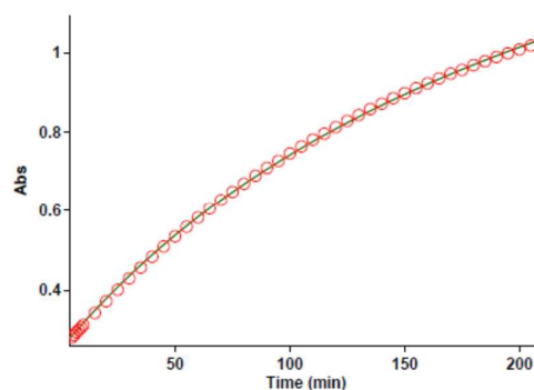
Fig. 3. The original experimental absorbance curve versus time at selected wavelength of 420 nm for the reaction between 1 ( 10^{-2} \text{ M} ) and 2 ( 10^{-2} \text{ M} ) with 3 ( 10^{-2} \text{ M} ) in formic acid. Dotted line is experimental values and the solid line is a fit curve
