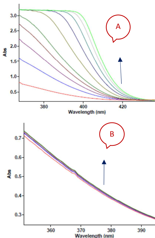
Fig. 7-A: Changes in absorption spectra vs. wavelength in 20°C for the reaction between aniline 1 and diethylacetylenedicarboxylate 2 in formic acid as reaction proceeds into a 10 mm light-path cell. The total acquisition time was 45 min; the time increment was set to 5 min. Herein, the upward of direction of the arrow indicate that the progress of reaction
