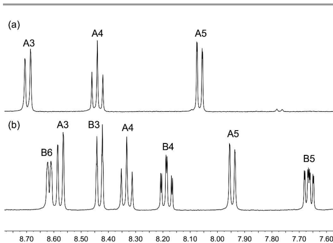
Fig. 2. 500 MHz ^1\text{H} NMR spectra of (a) [\text{Cu}(\mathbf{2})_2][\text{PF}_6] and (b) [\text{Cu}(\mathbf{3})_2][\text{PF}_6] in \text{CD}_2\text{Cl}_2 . Chemical shifts in \delta / ppm. See Scheme 3 for ring labelling.
