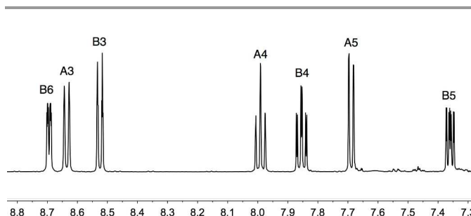
Fig. 1. 500 MHz 1 H NMR spectrum of compound 3 in CDCl 3 . Chemical shifts in \delta /ppm. See Scheme 3 for ring labelling.
