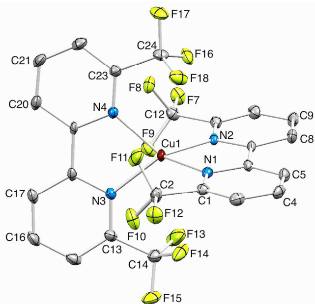
Fig. 5. Structure of the [\text{Cu}(\mathbf{2})_2]^+ cation in [\text{Cu}(\mathbf{2})_2][\text{PF}_6] ; H atoms omitted and ellipsoids plotted at 30% probability level. Selected bond parameters: Cu1–N1 = 2.036(3), Cu1–N2 = 2.021(3), Cu1–N3 = 2.030(3), Cu1–N4 = 2.027(3) Å; N1–Cu1–N2 = 82.41(11) , N1–Cu1–N3 = 124.71(12) , N2–Cu1–N3 = 127.02(11) , N1–Cu1–N4 = 123.51(11) , N2–Cu1–N4 = 122.05(11) , N3–Cu1–N4 = 82.85(12)^\circ ; C–F bond distances are in the range 1.319(5) to 1.341(4) Å.
