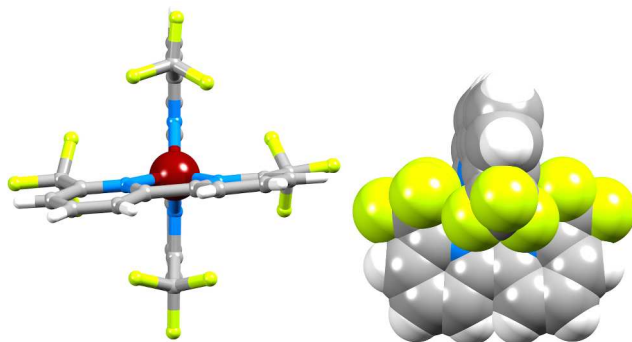
Fig. 6. (a) View of the [\text{Cu}(\mathbf{2})_2]^+ cation showing helical twist in one ligand; (b) space-filling diagram illustrating the shielding of the Cu1 atom by the four \text{CF}_3 groups.
