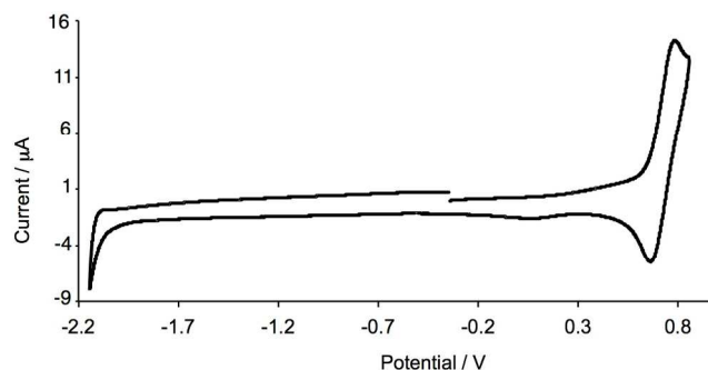
Fig. 4. Cyclic voltammogram of [\text{Cu}(\mathbf{3})_2][\text{PF}_6] in \text{CH}_2\text{Cl}_2 (referenced externally to \text{Fc}/\text{Fc}^+ ). Scan rate = 300 \text{ mV s}^{-1} ; Pt working electrode.
