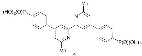
Scheme 4. Structure of the anchoring ligand 4 used in DSCs.
