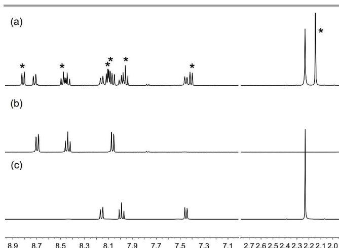
Fig. 7. 500 MHz NMR spectra of \text{CD}_2\text{Cl}_2 solutions of (a) [\text{Cu}(\mathbf{1})_2][\text{PF}_6] and [\text{Cu}(\mathbf{2})_2][\text{PF}_6] 15 minutes after mixing; peaks due to [\text{Cu}(\mathbf{1})(\mathbf{2})]^+ are shown with *; (b) [\text{Cu}(\mathbf{2})_2][\text{PF}_6] ; (c) [\text{Cu}(\mathbf{1})_2][\text{PF}_6] . The initial solution for (a) contained 0.38 mmol of each of [\text{Cu}(\mathbf{1})_2][\text{PF}_6] and [\text{Cu}(\mathbf{2})_2][\text{PF}_6] . Chemical shifts in \delta / ppm. Note that in the mixture shown in (a), signals for \mathbf{1} in [\text{Cu}(\mathbf{1})_2][\text{PF}_6] are slightly broader than those \mathbf{1} in [\text{Cu}(\mathbf{1})(\mathbf{2})][\text{PF}_6] ; for the Me signals, FWHM = 9 Hz in [\text{Cu}(\mathbf{1})_2][\text{PF}_6] and 7 Hz in [\text{Cu}(\mathbf{1})(\mathbf{2})][\text{PF}_6] .
