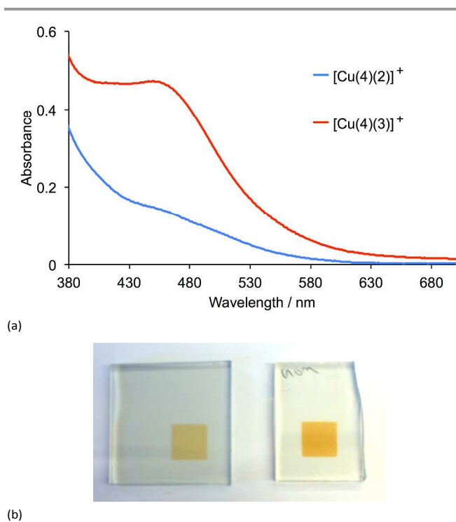
Fig. 8. (a) Solid-state absorption spectra of transparent \text{TiO}_2 electrodes functionalized with the dyes [\text{Cu}(\mathbf{4})(\mathbf{2})]^+ and [\text{Cu}(\mathbf{4})(\mathbf{3})]^+ . (b) Photographs of the two electrodes with dyes [\text{Cu}(\mathbf{4})(\mathbf{2})]^+ (left) and [\text{Cu}(\mathbf{4})(\mathbf{3})]^+ (right).
