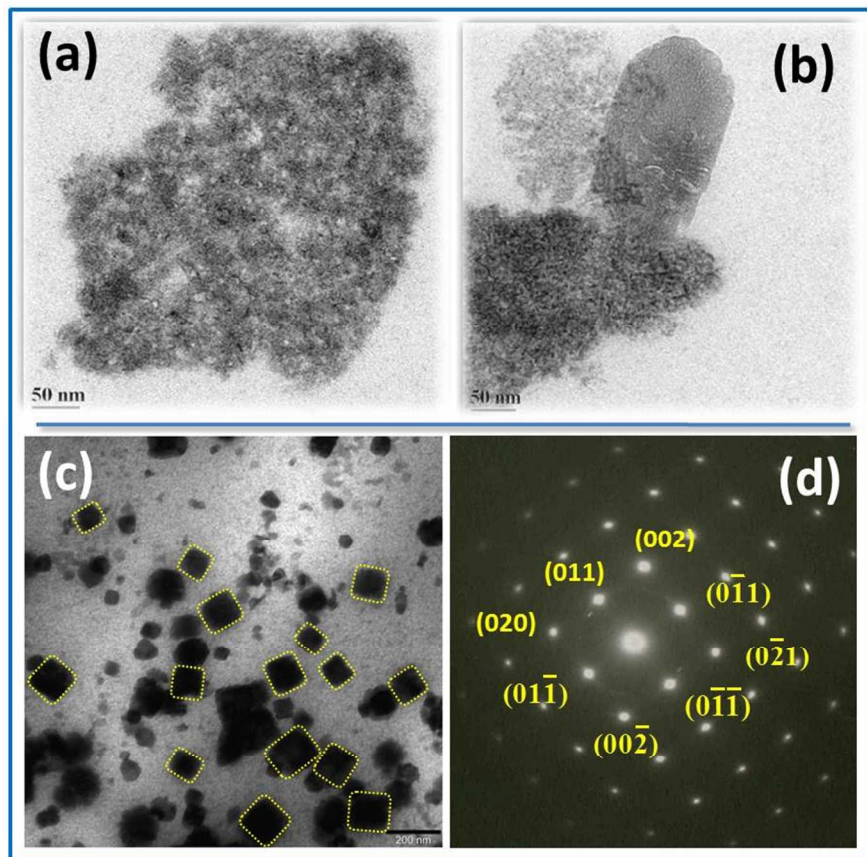
Fig.4. TEM images showing the (a) self-assembling of primary nanoparticles (image recorded within 5 minutes of the reaction); (b) formation of sheet like nanostructures (image recorded after ~ 20 minutes of the reaction); (c) nanosheets of SnSe ( bar dimensions = 200 nm ) (image recorded after ~ 2 hours of the reaction); (d) SAED pattern indicating the single crystalline nature of the nanosheets of SnSe.
