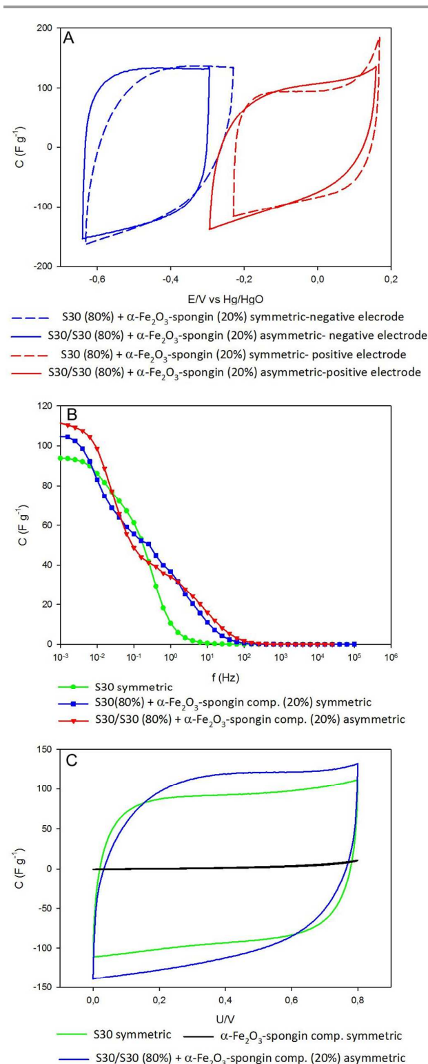
Fig. 8 (A) Cyclic voltammograms of pellets of composite ( \alpha -Fe 2 O 3 -spongine composite) mixed with activated carbon Supra DLC 30 (20:80) at 10 mVs -1 scan rate (two-electrode cell); (B) Capacitance vs frequency dependence of the composite blend ( \alpha -Fe 2 O 3 -spongine composite) with activated carbon Supra DLC 30 (20:80); (C) Cyclic voltammograms at 5 mVs -1 scan rate for the three-electrode cell.
