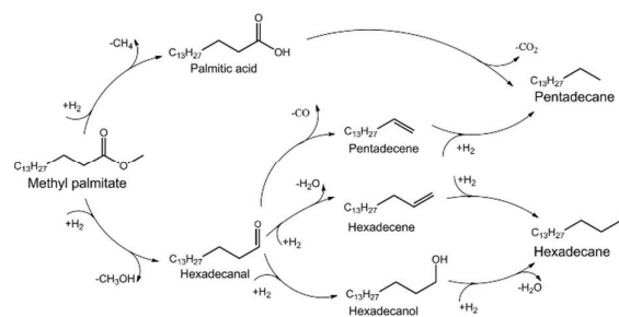
Scheme 1. The HDO route of methyl palmitate over Ni 2 P/SiO 2 .
