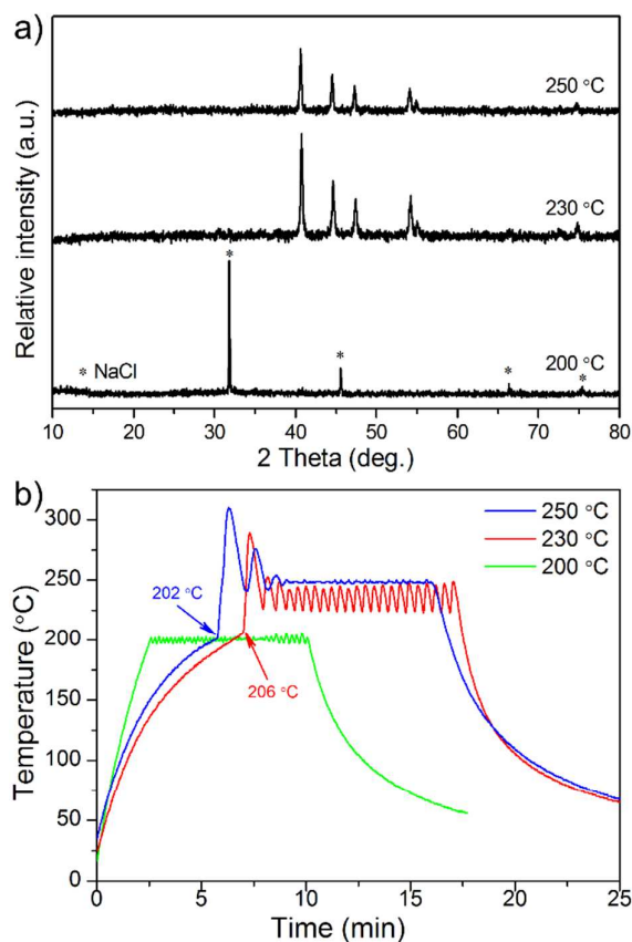
Fig. 1. (a) The XRD patterns of the samples prepared at different temperatures for 10 min from the precursors with a mole ratio of P/Ni = 1.5, (b) microwave temperature patterns of the samples in different setting values.
