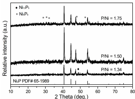
Fig. 2. The XRD patterns of bulk Ni 2 P prepared with different mole ratios of P/Ni (microwave radiation at 230 °C for 10 min).
