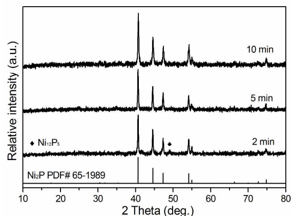
Fig. 3. The XRD patterns of bulk Ni 2 P prepared with different microwave radiation time (microwave radiation at 230 °C, P/Ni = 1.5).
