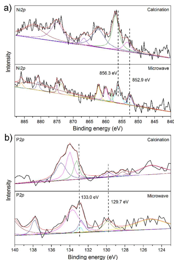
Fig. 6. The XPS spectra of 30 wt% \text{Ni}_2\text{P}/\text{SiO}_2 catalysts prepared using different methods: (a) \text{Ni}2p core level spectra of \text{Ni}_2\text{P}/\text{SiO}_2 , (b) \text{P}2p core level spectra of \text{Ni}_2\text{P}/\text{SiO}_2 .
