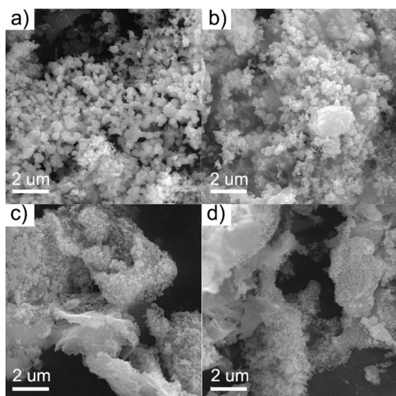
Fig. 4. The SEM images of bulk \text{Ni}_2\text{P} prepared using different methods, (a) and (b) prepared using calcination method ( \text{P}/\text{Ni} = 1.5 , 250\text{ }^\circ\text{C} , 30 min), (c) and (d) prepared using microwave method ( \text{P}/\text{Ni} = 1.5 , 230\text{ }^\circ\text{C} , 5 min).
