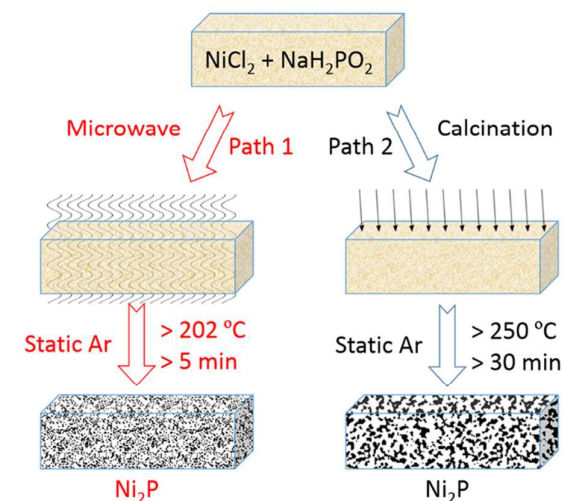
Scheme 2. Pathway of two methods.
