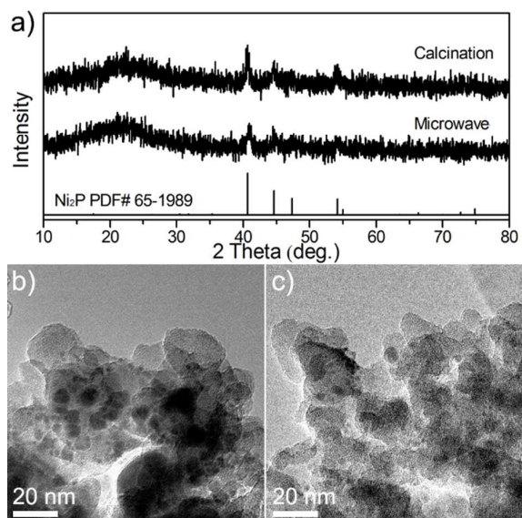
Fig. 5. The XRD patterns and TEM images of 30 wt% \text{Ni}_2\text{P}/\text{SiO}_2 catalysts prepared using different methods, (a) XRD patterns, (b) prepared using calcination method ( \text{P}/\text{Ni} = 1.5 , 250\text{ }^\circ\text{C} , 30 min), and (c) prepared using microwave method ( \text{P}/\text{Ni} = 1.5 , 230\text{ }^\circ\text{C} , 5 min).
