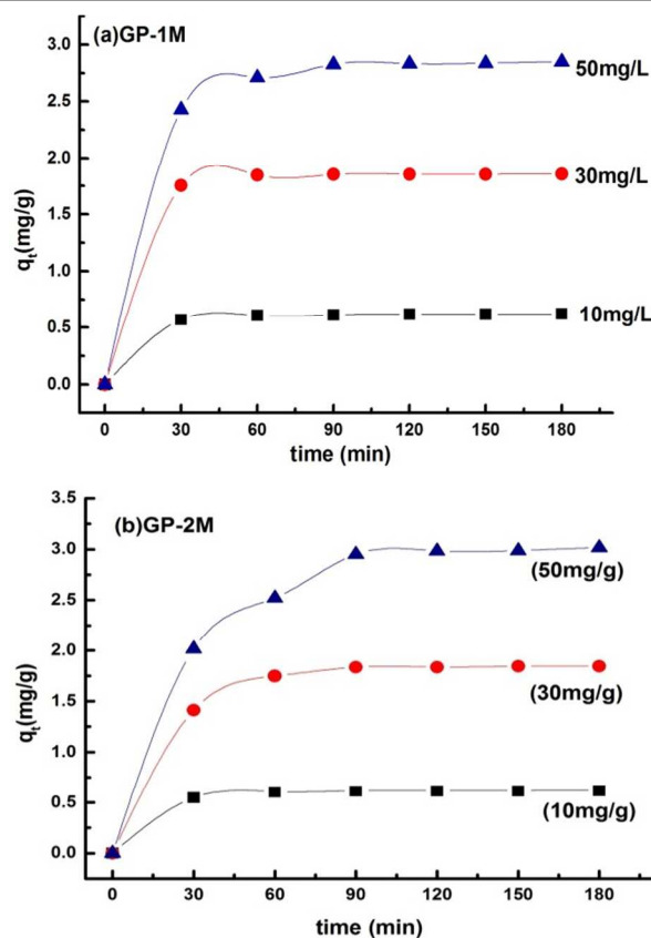
Figure 7 Effect of initial conc. and time on the MB adsorption over (a) GP-1M (b) GP-2M. (25ml of MB solution was used at 28°C and 150rpm.)
