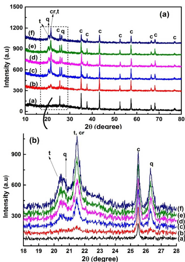
Figure 5(a) XRD analysis of the PAGPs (b) a closer view of the selected region. In the figure samples details are; (a) GP-1M (b) GP-2M (c) GP-1MT (d) GP-2MT (e) GP-1MR and (f) GP-2MR, whereas "T" represents samples treated at 800^\circ\text{C} for 2 hours and "R" stands for regenerated adsorbents. Small letter c, cr, t and q are used to represent corundum, cristobalite, tridymite and quartzite phases.
