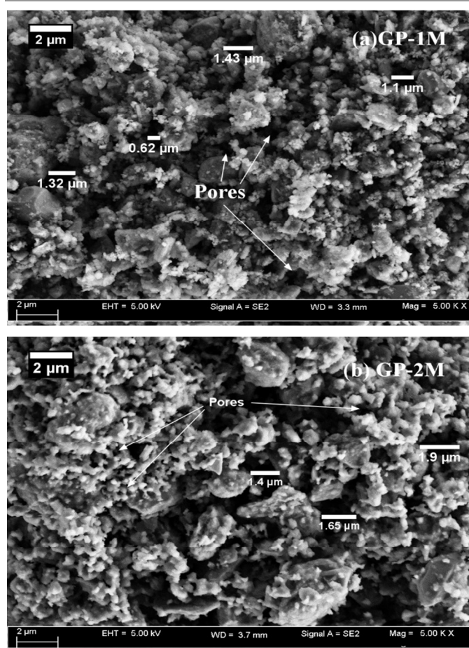
Figure 3 FESEM analysis of (a) GP-1M (b) GP-2M
