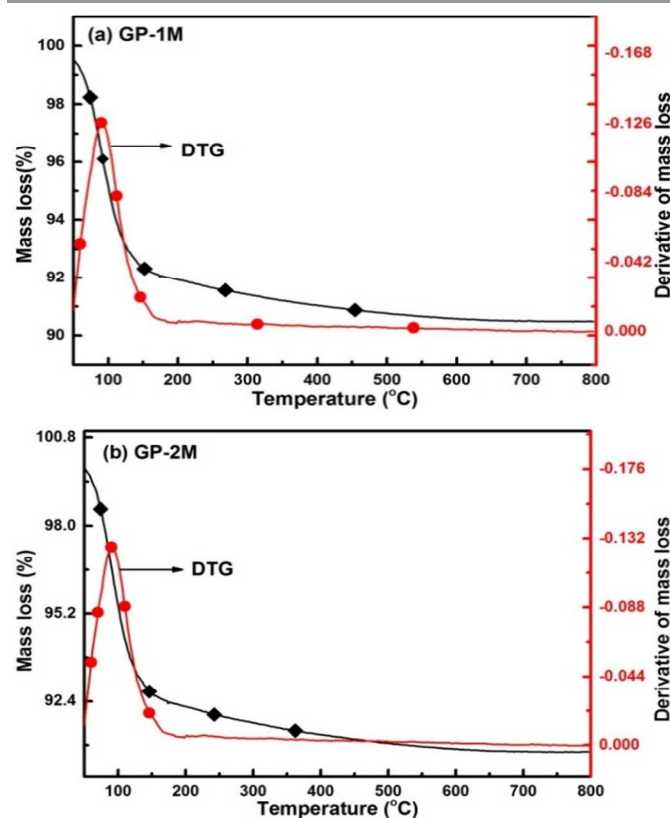
Figure 4 Thermogravimetric analysis of (a) GP-1M (b) GP-2M in N 2 environment
