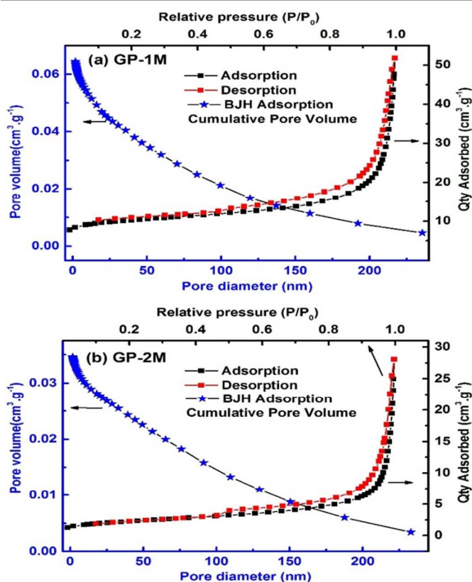
Figure 2 Nitrogen adsorption-desorption isotherm and pore analysis profile of (a) GP-1M (b) GP-2M
