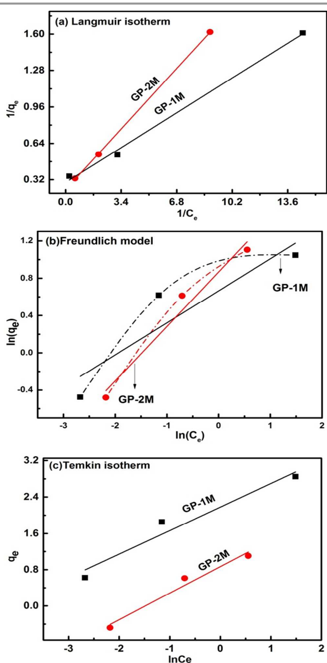
Figure 10 Isotherm plots of GP-1M and GP-2M (a) Langmuir isotherm (b) Freundlich isotherm and (c) Temkin isotherm
