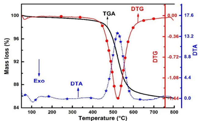
Figure 1 Thermogravimetric analysis of the kaolin in \text{N}_2 environment. TG, DTG and DTA curves are shown in the Figure.
