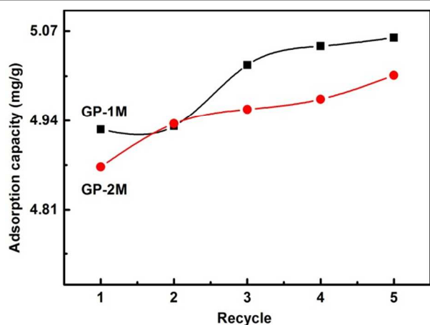
Figure 11 Adsorption capacity of GP-1M and GP-2M after regeneration (50ml of 50mg/L MB solutions were used at 28°C and 150rpm.)
