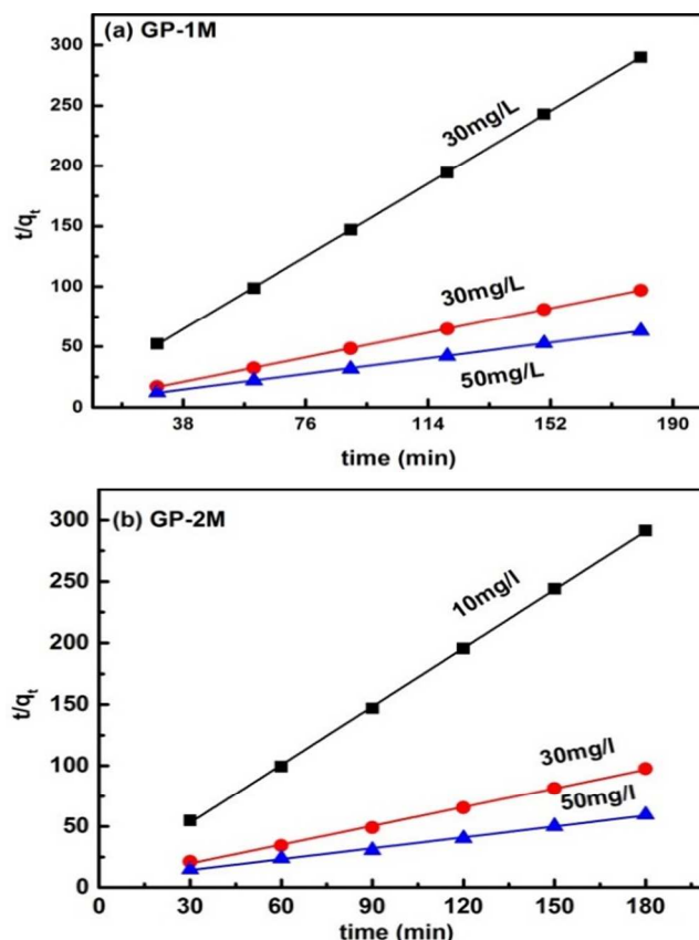
Figure 9 Pseudo second order kinetics model of (a) GP-1M (b) GP-2M. (25ml of MB solutions were used at 28°C and 150rpm.)
