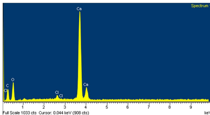
Fig. 6 EDS of finely powdered cuttlebone.
