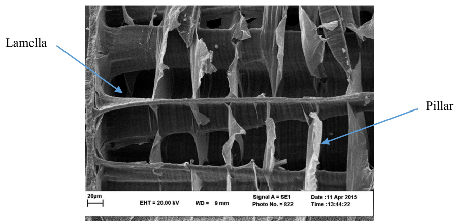
Fig. 4 SEM image of cuttlebone.
