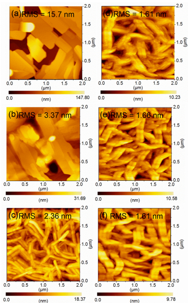
Figure 10. AFM images of thin films (45 nm) of (a) 1 , (b) 2 and (c) 3 thermally evaporated on TTC (20 nm) modified substrates and thin film of 3 deposited elevated substrate temperature at (d) r.t., (e) 80 °C, and (f) 100 °C
