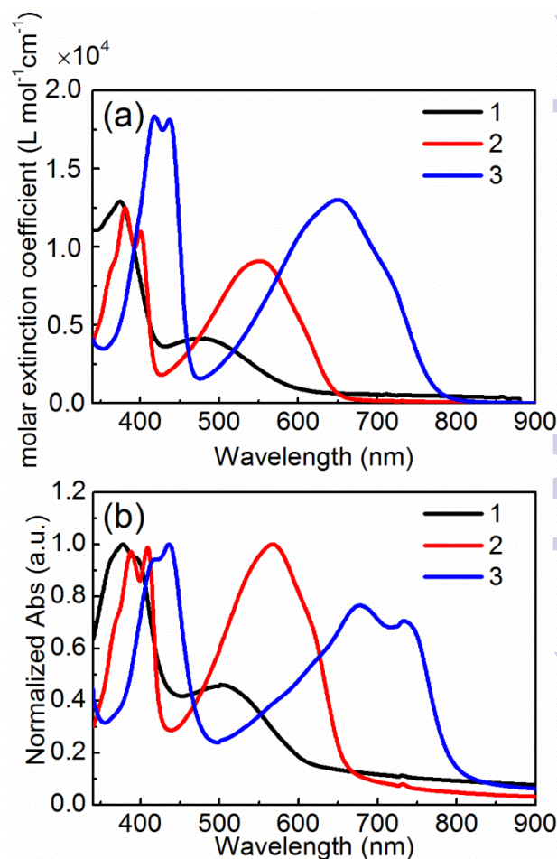
Figure 3. UV-vis absorption spectra of 1-3 for (a) 10^{-5} M \text{CHCl}_3 solutions and (b) thin films spin-coated from \text{CHCl}_3 solutions
