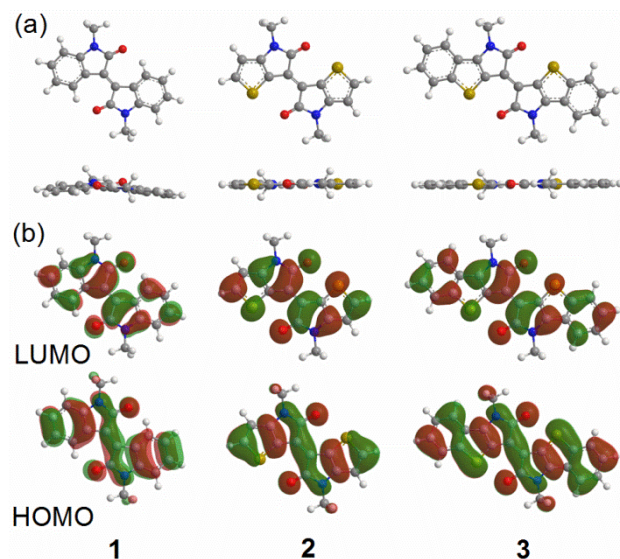
Figure 2. (a) Optimized molecular geometries and (b) the calculated distributions of the HOMO and LUMO orbitals of methyl-substituted 1-3 estimated from the DFT calculations
