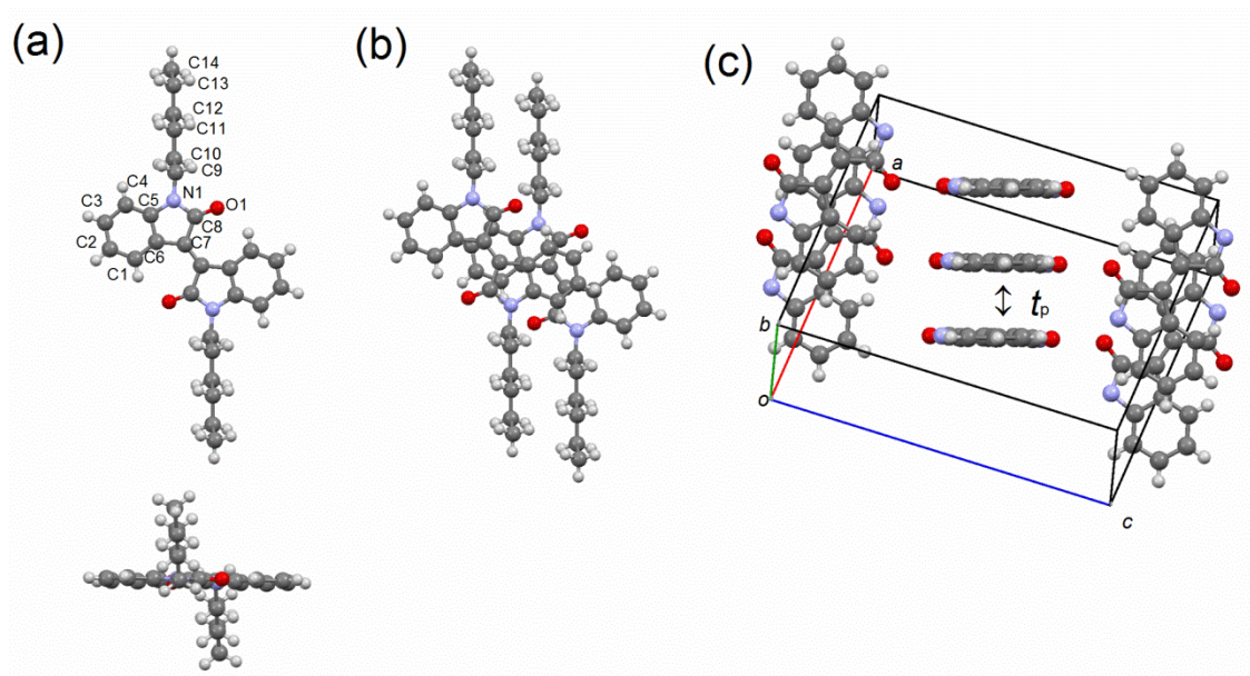
Figure 5. (a) Molecular structure, (b) overlap mode, and (c) molecular packing of 1 , in which alkyl chains are omitted for clarification.
