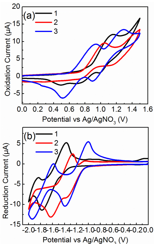
Figure 4. Cyclic voltammograms of 1-3 measured in 0.1 M \text{Bu}_4\text{NPF}_6 in \text{CH}_2\text{Cl}_2 at the scan rate of 100 \text{ mV s}^{-1} , (a) positive scans for oxidation steps and (b) negative scans for reducing steps.
