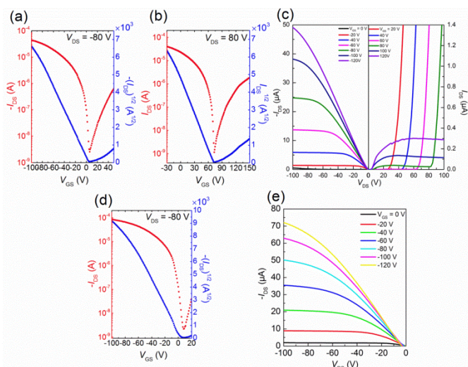
Figure 8. (a) p -type and (b) n -type transfer curves, and (c) output curve for the TTC modified device of 3 . (d) p -type transfer curve and (e) output curve for the OTMS modified substrate elevated at 80 °C of 3 .
