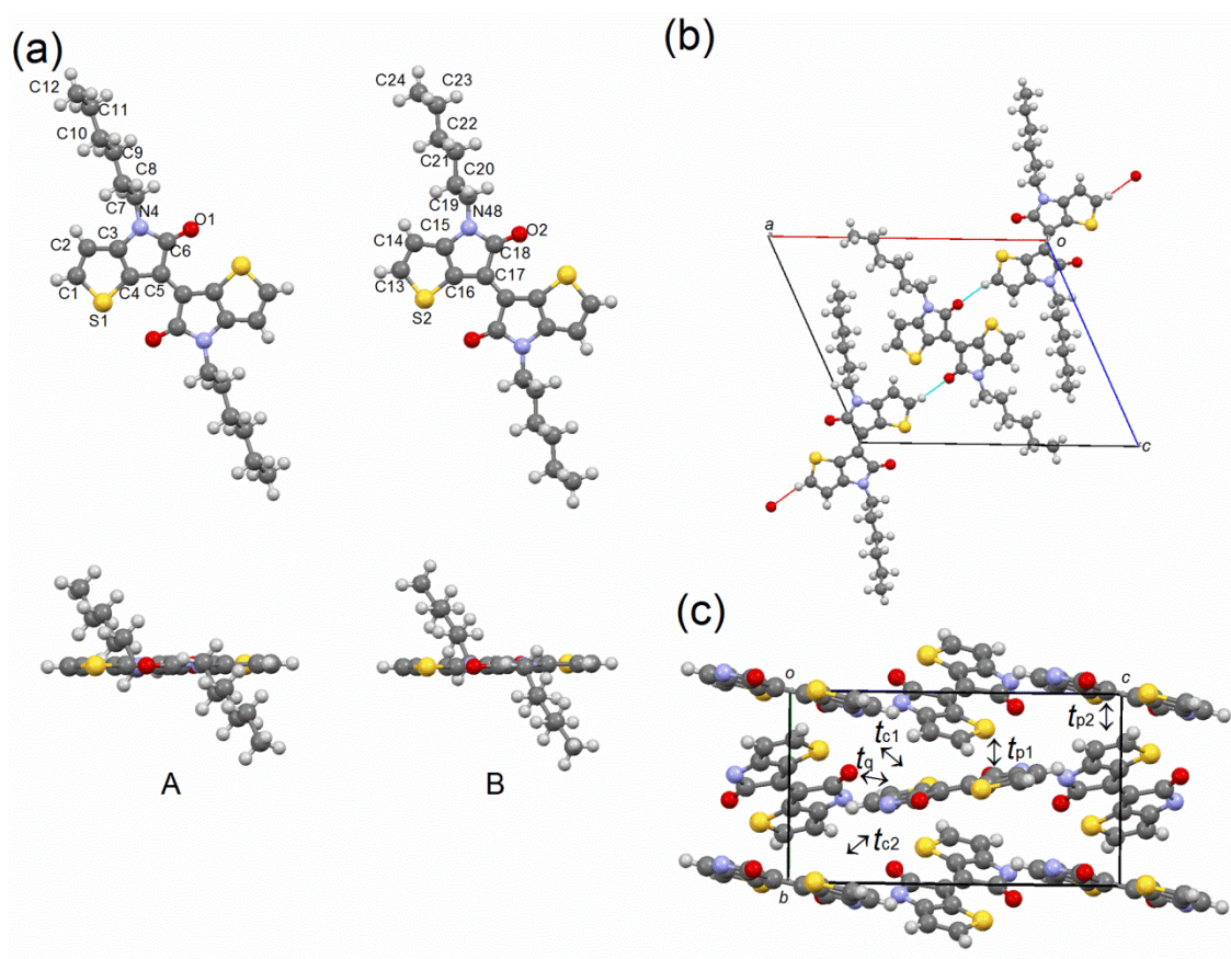
Figure 6. (a) Molecular structure, (b) H-bonding chains along the a + c direction, and (c) molecular packing of 2 , in which the alkyl chains are omitted for clarification.
