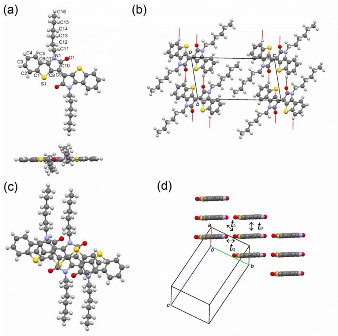
Figure 7. (a) Molecular structure, (b) H-bonding chains along the b axis, (c) overlap mode, and (d) molecular packing of 3 , in which alkyl chains are omitted for clarification.
