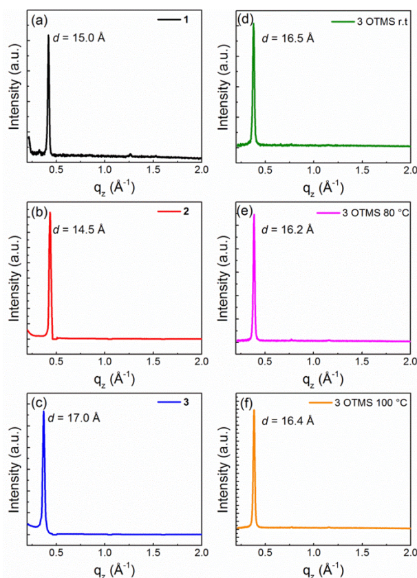
Figure 9. X-ray diffraction patterns of (a) 1 , (b) 2 and (c) 3 thin films (45 nm) deposited on TTC (20 nm) modified substrates and thin film of 3 deposited elevated substrate temperature at (d) r.t., (e) 80 °C, and (f) 100 °C
