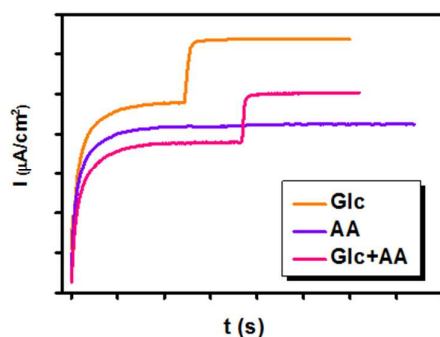
Figure 11. Amperometric biosensor response of (SNS-NH 2 )/GOx to glucose in the presence of AA
