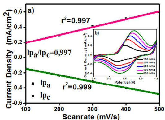
Figure 4. (a) Dependence scan rate on peak current for P(SNS-mNH 2 ) ( I_{p_a} : anodic peak current value, I_{p_c} : cathodic peak value, r^2 : linear regression value). (b) CV of P(SNS-mNH 2 ) at different scan rates
