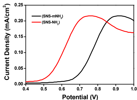
Figure 2. Anodic polarization curves of SNS-NH 2 and SNS-mNH 2
