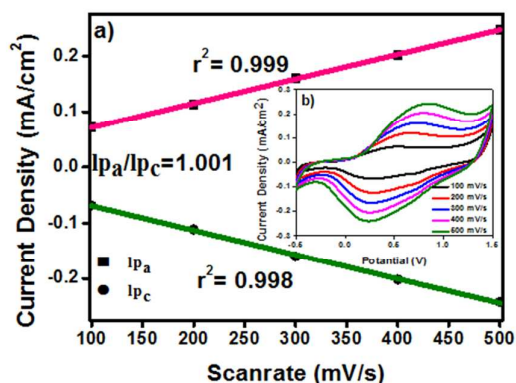
Figure 3. (a) Dependence scan rate on peak current for P(SNS-NH 2 ) ( I_{p_a} : anodic peak current value, I_{p_c} : cathodic peak value, r^2 : linear regression value), (b) CV of P(SNS-NH 2 ) at different scan rates
