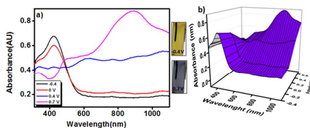
Figure 6. Optoelectrochemical spectrum of P(SNS-mNH 2 ) film (a) 2D and (b) 3D.
