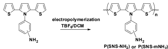
Scheme 2. Electrochemical synthesis route for P(SNS-NH 2 ) and P(SNS-mNH 2 ).
