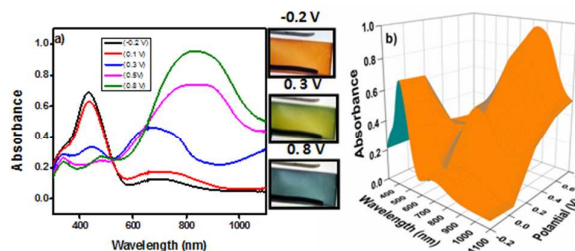
Figure 5. Optoelectrochemical spectrum of P(SNS-NH 2 ) film (a) 2D and (b) 3D.
