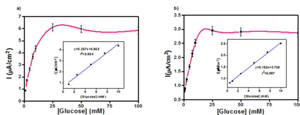
Figure 10. Calibration curve of (a) P(SNS-NH 2 )/GOx (b) P(SNS-mNH 2 )/GOx enzyme electrode by amperometric detection in Na-Acetate buffer
