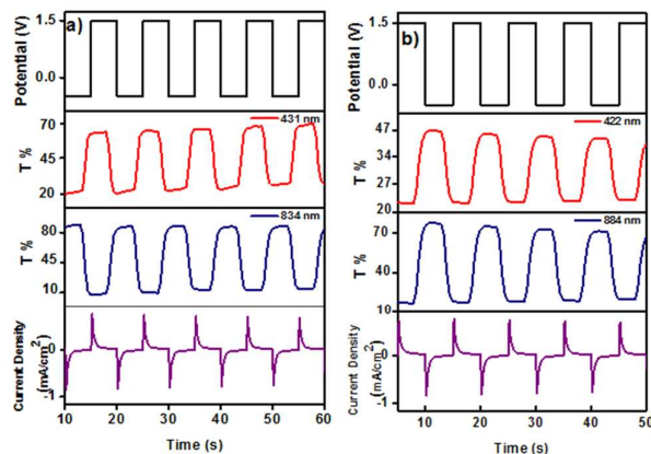
Figure 7. Potential, absorbance and current density versus-time graphs of P(SNS-NH 2 ) (a) and P(SNS-mNH 2 ) (b)
