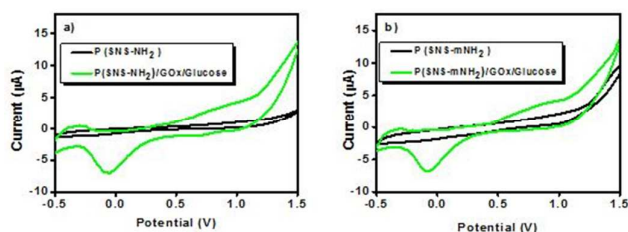
Figure 8. CVs of (a) P(SNS-NH 2 ), P(SNS-NH 2 )/GOx/Glucose b) P(SNS-mNH 2 ), P(SNS-mNH 2 )/GOx/Glucose (Na-acetate buffer pH 4.5, 50 mM at 250 mV/scan rate)
