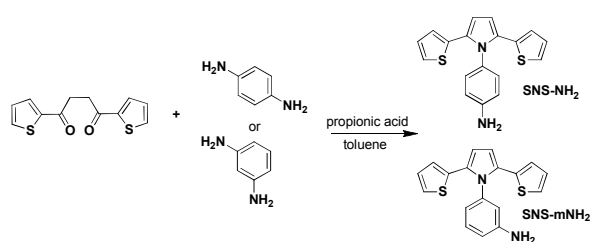
Scheme 1. The synthetic route of SNS-NH 2 and SNS-mNH 2
