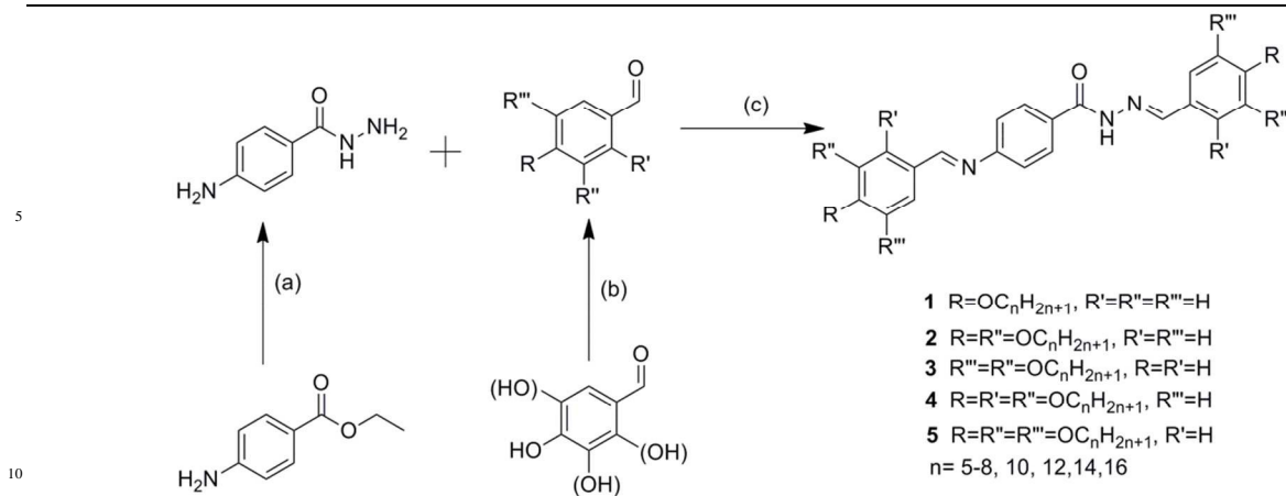
Scheme 1. Reactions and reagents: (a) \text{NH}_2\text{NH}_2 (1.5 equiv.), refluxing in absolute EtOH, 12 h, 85–90%. (b) RBr (n equiv.), \text{K}_2\text{CO}_3 (4xn equiv.), KI (catalyst), refluxing in 2-butanone, 24–72 h, 70–85%. (c) acetic acid (cat.), refluxing in EtOH, 12 h, 74–87%.
