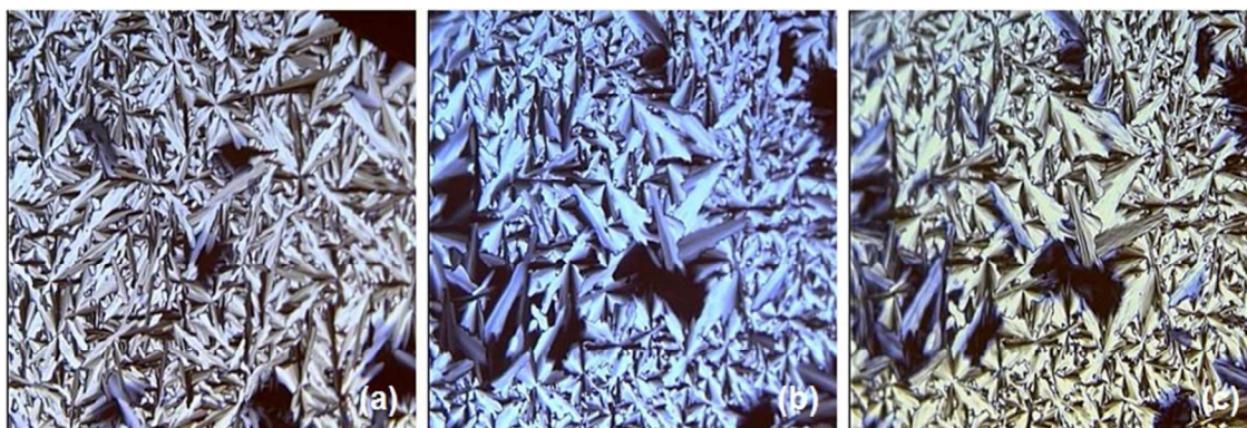
Fig. 8 Microphotographs of the compounds 5(n=10) Col r phase in cooling cycle (a) at 109.1^\circ\text{C} (b) at 104.2^\circ\text{C} (c) 90.2^\circ\text{C}
