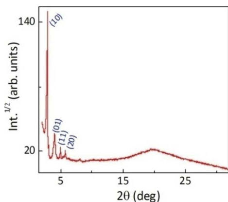
Fig. 9 XRD pattern of the compound 5(n=10) at 100^\circ\text{C} .
