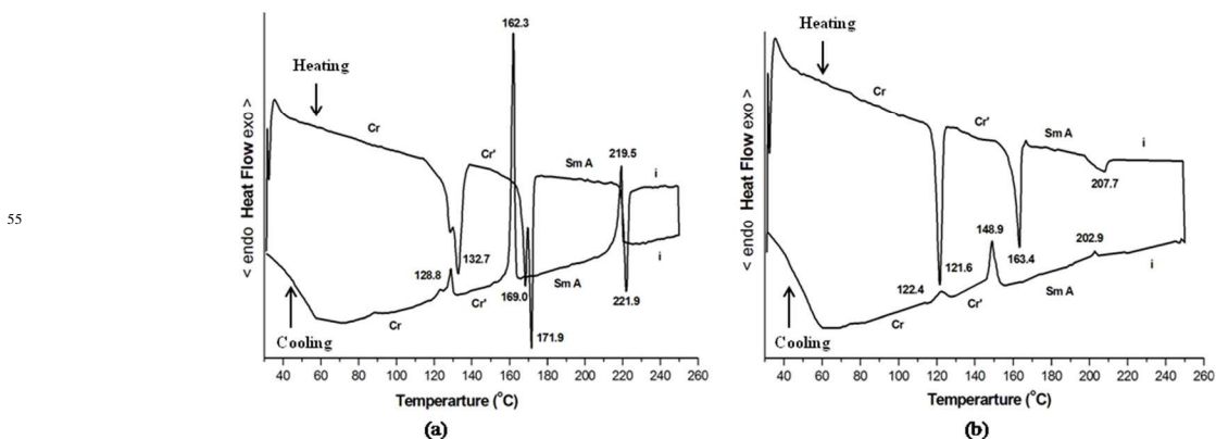
Fig. 2 DSC thermograms of the compound 1 (a) n= 12 and (b) n=14 showing enantiotropic mesophase
