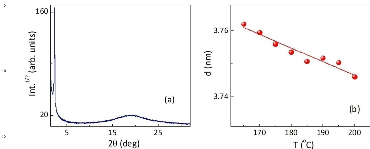
Fig. 4 X-ray measurements on the I ( n=12 ) compound. (a) Raw XRD profile collected at 200°C, exhibiting a sharp low angle peak and a wide angle diffuse maximum. (b) Thermal variation of the layer thickness.
