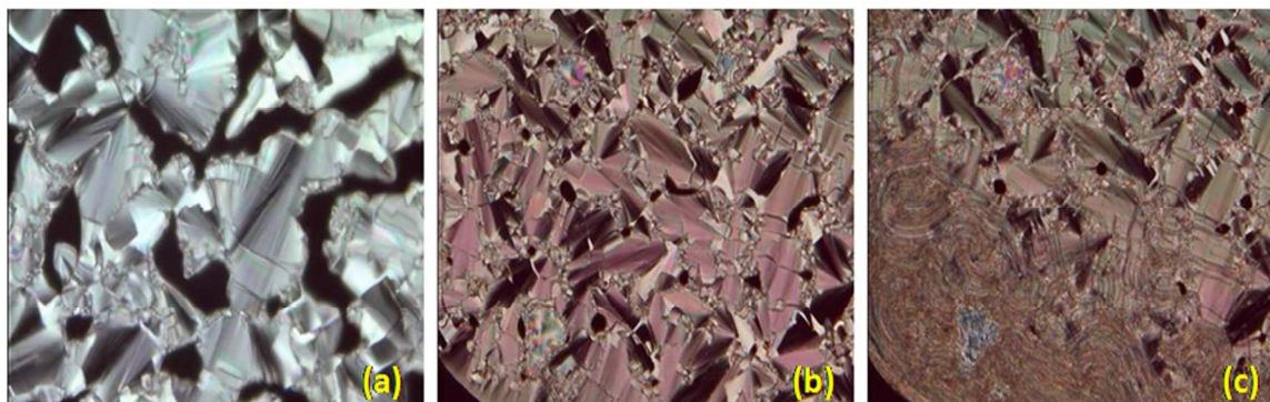
Fig. 3 Microphotographs of the compound 1 ( n=12 ) in SmA phase in cooling cycle (a) broken focal conic texture of compound at 192.1°C, (b) broken focal conic texture at 184.1°C and (c) SmA to crystal transition of the compound at 162.2°C.
