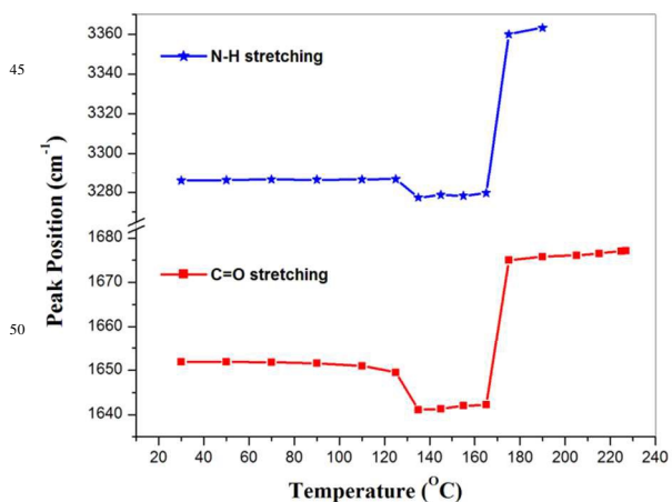
Fig. 5. Peak position variation with temperature of C=O and N-H stretching Raman bands of compound 1 ( n=12 ).
