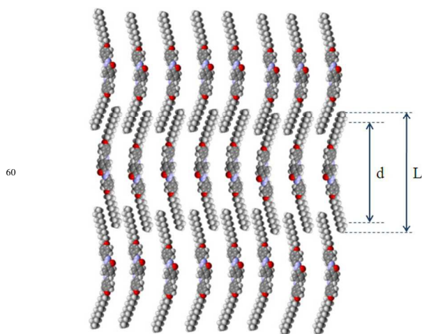
Fig. 6. Schematic representation of molecules in SmA phase.
