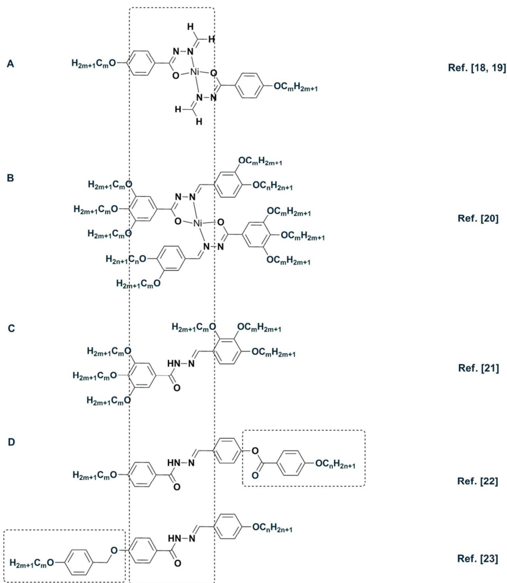
Fig. 1 A: Mesogenic mono-alkoxy arylhydrazone-nickel (II) complex reported by McCabe et al. 18-19 B: Polycatenar arylhydrazone-nickel (II) complexes reported by Lai et al. 20 C: Structure of non-symmetrical polycatenar arylhydrazones reported by Yelamaggad et al. 21 D: Substituted arylhydrazones at benzylidene- 22 and benzoyl- position 23 reported by Singh et al.
