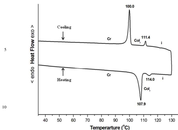
Fig. 7 DSC thermogram of the compound 5 (n=10) showing enantiotropic mesophase
