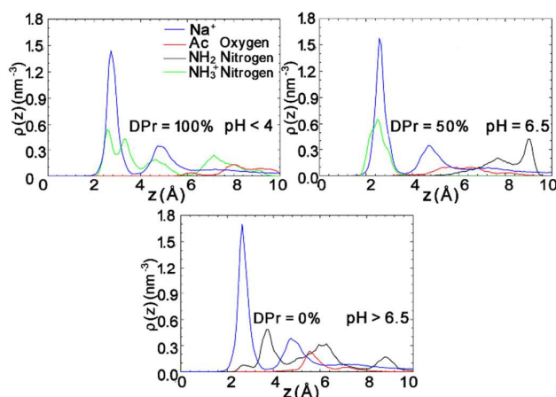
Figure 7. Density profiles of the different functional group atoms of the polymer and counter ions at the interfacial area of CHS 20% -Mnt systems at different DPr. Density value of counter ions \text{Na}^+ are divided by a factor of 5 to present all plots in a uniform range. Plots are calculated from the last 50ns trajectories.
