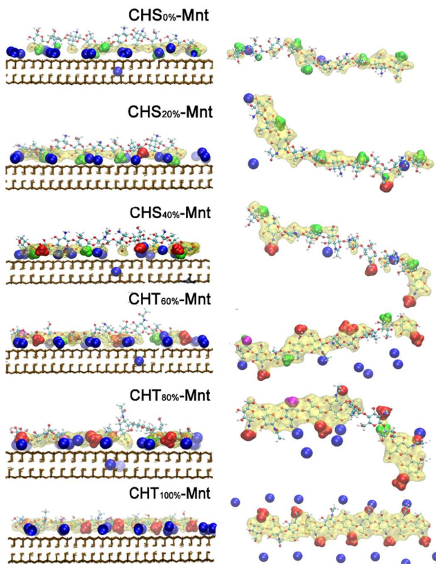
Figure 5. Snapshot of the equilibrated CHS or CHT-Mnt conformation. The left panel is in a front view corresponding to each CHS-Mnt or CHT-Mnt system at different DA. The right panel is in a top view of the conformation of CHS or CHT
