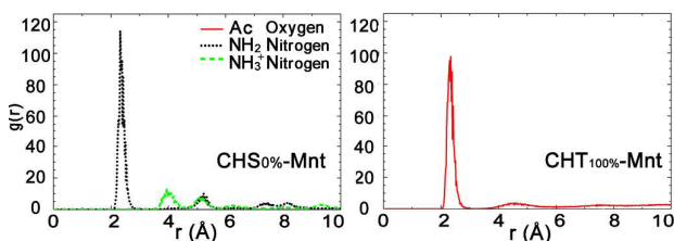
Figure 4. Radial distribution functions (RDFs) between the functional group atoms of the polymer and counterions \text{Na}^+ in the \text{CHS}_{0\%} -Mnt (left) and \text{CHT}_{100\%} -Mnt (right) systems. Plots are calculated from the last 50ns trajectories.
