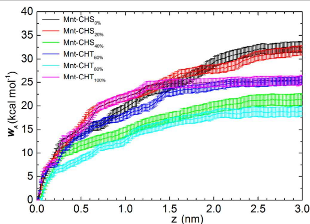
Figure 2. Free energy profiles for the studied CHS-Mnt or CHT-Mnt systems at different DA. The starting point of x-axis is normalized to the adsorbed conformation in each system; the distance ( z ) is measured along the perpendicular direction of the clay surface. The y-axis refers to the free energy difference, known as the work of adhesion ( W_A ).
