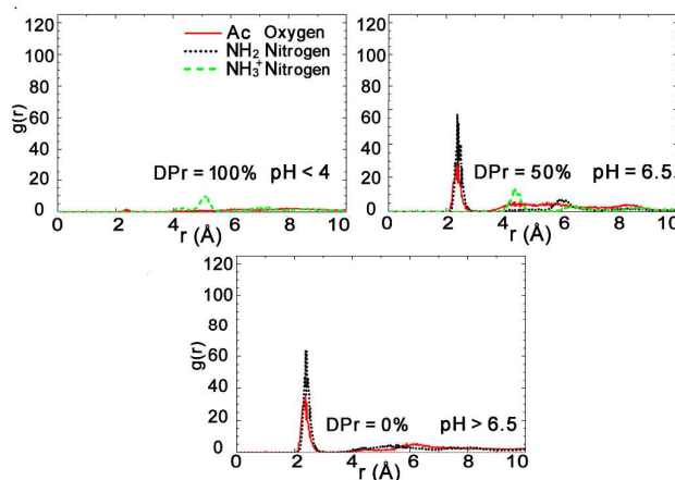
Figure 9. Radial distribution functions (RDFs) between the functional group atoms of CHS 20% and counter ions \text{Na}^+ for CHS 20% -Mnt systems at different DPr. Plots are calculated from the last 50ns trajectories.
