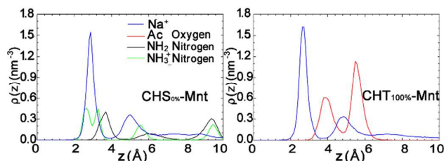
Figure 3. Density profiles of the different functional group atoms of the polymer and counter ions at the interfacial area of CHS 0% -Mnt (left) and CHT 100% -Mnt (right) systems. Density value of counter ions Na^+ are divided by a factor of 5 to present all plots in a uniform range. Plots are calculated from the last 50ns trajectories.
