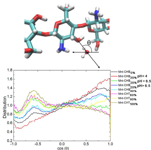
Figure 10. Orientation distribution of water molecules within a 0.5 nm radius of the hydroxyl O3 atom of the studied oligomers when adsorbed to Mnt. The horizontal axis shows the average value of the cosine of the angle \theta , which is defined by two vectors: one is the water dipole vector, the other is the vector formed between the O3 and the water oxygen, as marked by the black arrows in the upper panel. Color scheme for the sugar unit in the upper panel: carbon (cyan), oxygen (red), hydrogen (white), nitrogen (blue).
