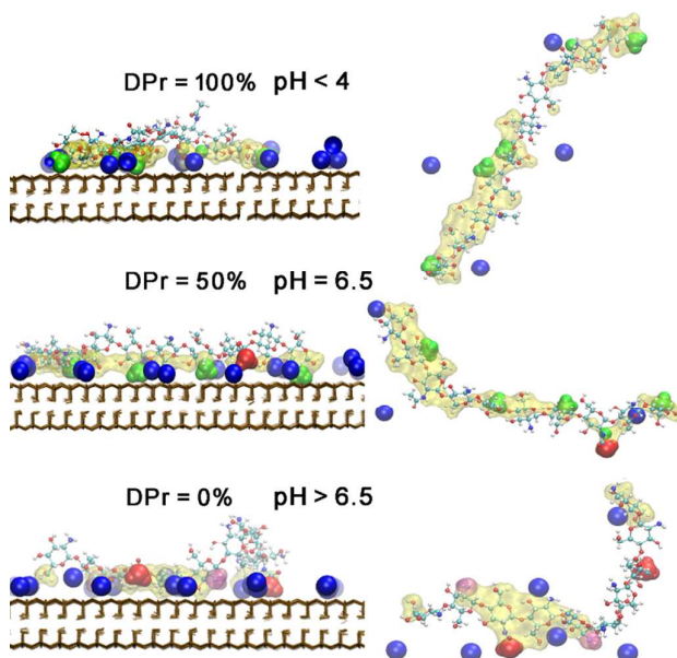
Figure 8. Snapshots of equilibrated CHS 20% -Mnt complex at three different DPr. The left panel is in a front view. Right panel is in a top view of each CHS 20% polymer, corresponding to the left panel. Colour and drawing scheme is the same as Figure 5.
