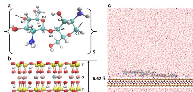
Figure 1. Molecular presentation of a) molecular structure of one glucosamine dimer, the CHS or CHT chain formed by five dimers with different number of acetylated unit to present different DA; Glucosidic linkage dihedral angles \phi and \psi are defined by atoms O5 C1 O4 C4 and C1 O4 C4 C3, respectively. b) Molecular structure of the super unit cell of Mnt clay: T, the tetrahedral layer; O, the octahedral layer. c) The front view of the simulation box for CHS-Mnt or CHT-Mnt system; the CHS or CHT chain is presented by licorice method, Mnt and counter ions are shown by CPK, and waters are drawn by lines.
