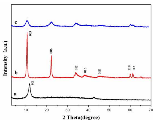
30 Fig. 2 XRD patterns of GO (a), NiAl-LDH (b) and NiAl-LDH/RGO (c).
