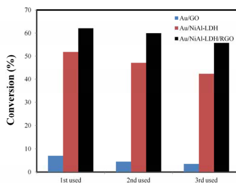
Fig. 12 Reusability of 1% Au catalysts supported by GO, NiAl-LDH and NiAl-LDH/RGO.
