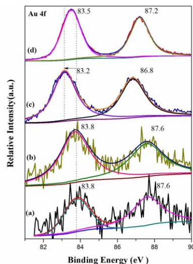
Fig. 8 Au 4f XPS of Au/silicon wafers (a), Au/GO (b), Au/NiAl-LDH (c) and Au/NiAl-LDH/RGO (d).
