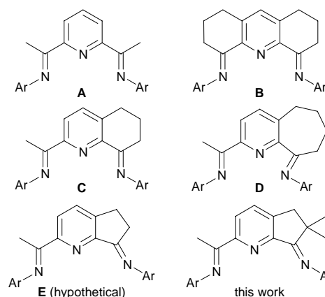
Scheme 1. Ligands derived from bis(imino)pyridines
