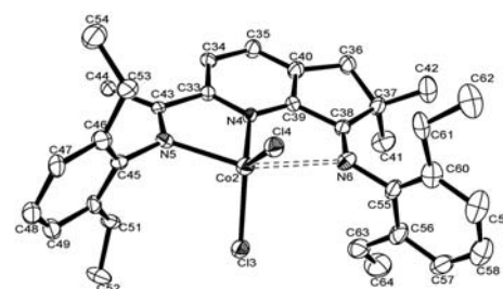
Figure 2B. Molecular structure of complex Co2 with thermal ellipsoids at 30% probability. Hydrogen atoms have been omitted for clarity. Selected bond lengths (Å) and angles (°): Co(2)–N(4) = 2.042(2), Co(2)–N(5) = 2.145(2), Co(2)–N(6) = 2.785, Co(2)–Cl(3) = 2.2360(8), Co(2)–Cl(4) = 2.2513(8); N(4)–Co(2)–N(5) = 76.69(7), N(4)–Co(2)–Cl(3) = 119.84(6), N(5)–Co(2)–Cl(3) = 103.61(6), N(4)–Co(2)–Cl(4) = 121.69(6), N(5)–Co(2)–Cl(4) = 107.72(6), Cl(3)–Co(2)–Cl(4) = 115.31(3).
