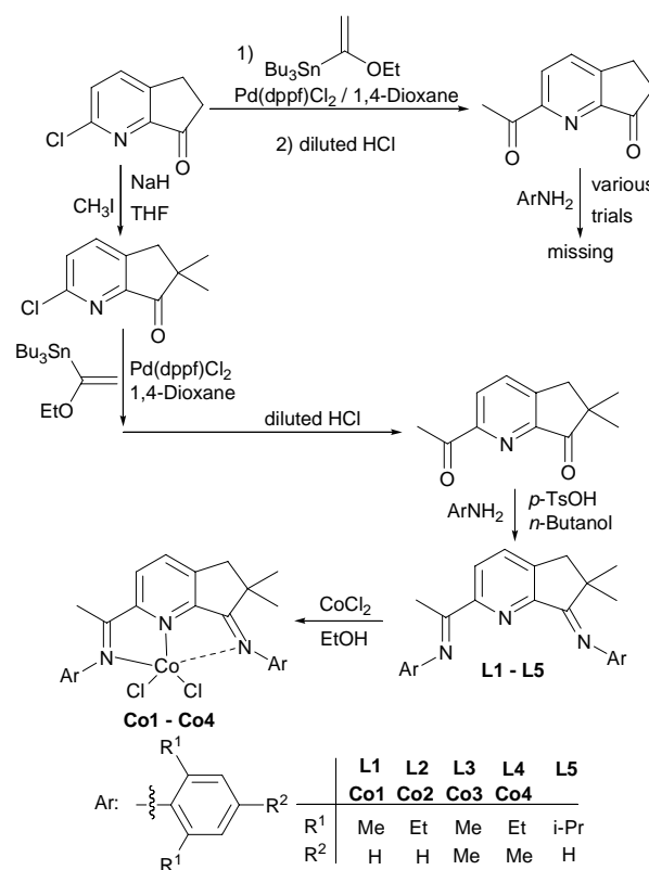
Scheme 2. Synthetic procedure for L1 - L5 and Co1 - Co4
