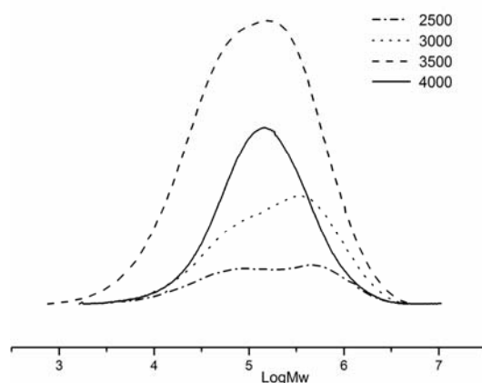
Figure 4. GPC traces of PEs produced with different Al/Co ratios (entries 3, 9-11, Table 1).
