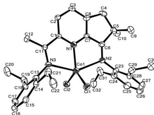
Figure 2A. Molecular structure of complex Co2 with thermal ellipsoids at 30% probability. Hydrogen atoms have been omitted for clarity. Selected bond lengths (Å) and angles (°): Co(1)–N(1) = 2.014(2), Co(1)–N(2) = 2.423(2), Co(1)–N(3) = 2.314(2), Co(1)–Cl(1) = 2.2450(10), Co(1)–Cl(2) = 2.2307(9); N(1)–Co(1)–N(3) = 73.54(8), N(1)–Co(1)–Cl(1) = 123.11(7), N(3)–Co(1)–Cl(1) = 95.11(6), N(1)–Co(1)–Cl(2) = 115.93(7), N(3)–Co(1)–Cl(2) = 98.26(6), Cl(1)–Co(1)–Cl(2) = 120.88(3).
