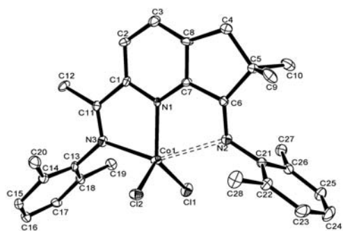
Figure 1. Molecular structure of complex Co1 with thermal ellipsoids at 30% probability. Hydrogen atoms have been omitted for clarity. Selected bond lengths (Å) and angles (°): Co(1)–N(1) = 2.018(3), Co(1)–N(2) = 2.690, Co(1)–N(3) = 2.188(3), Co(1)–Cl(1) = 2.2365(12), Co(1)–Cl(2) = 2.2454(12); N(1)–Co(1)–N(3) = 76.53(13), N(1)–Co(1)–Cl(1) = 125.03(11), N(3)–Co(1)–Cl(1) = 107.43(9), N(1)–Co(1)–Cl(2) = 112.89(11), N(3)–Co(1)–Cl(2) = 102.17(10), Cl(1)–Co(1)–Cl(2) = 119.14(5).
