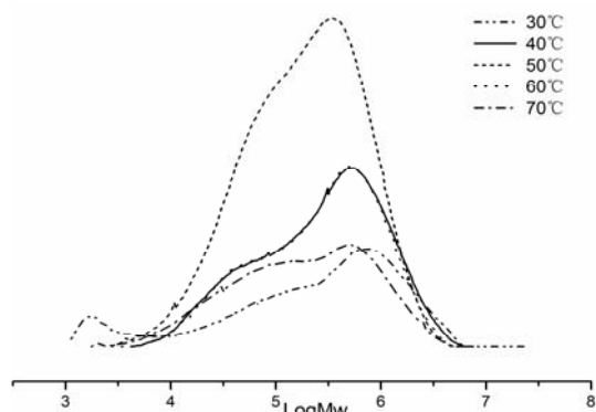
Figure 3. GPC traces of PEs produced at different reaction temperatures (entries 1-5, Table 1).
