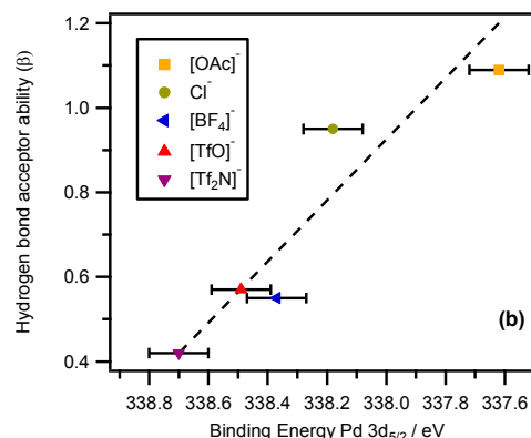
Figure 4 Pd 3d 5/2 binding energies for phosphineimidazolylidene palladium complexes in different [C 8 C 1 Im] + -based ionic liquids compared to hydrogen bond acceptor ability ( \beta ). All binding energies obtained were charge corrected by referencing the C alkyl 1s component to 285.0 eV. It must be noted that the experimental error with the XPS measurement is of the order \pm 0.1 eV.
