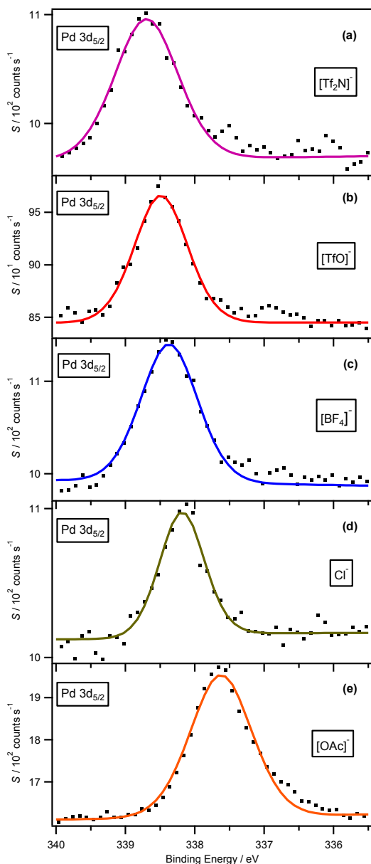
Figure 3 XPS spectra of Pd 3d 5/2 for phosphineimidazolylidene palladium complexes in a range of [C 8 C 1 Im] + -based ionic liquids, (a) [Tf 2 N] - (b) [TfO] - (c) [BF 4 ] - (d) Cl - and (e) [OAc] - . All XPS spectra were charge corrected by referencing the C alkyl 1s component to 285.0 eV.
