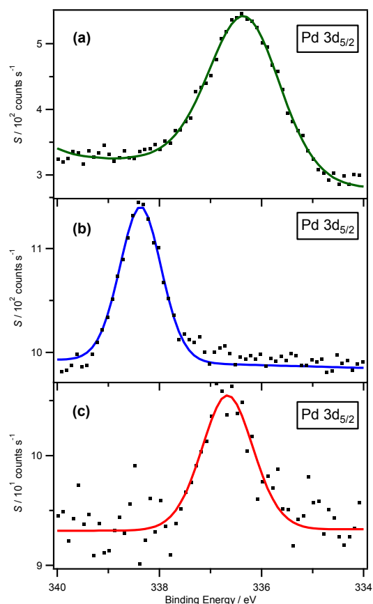
Figure 2 Pd 3d spectra of (a) solid [\text{Pd}(\text{PPh}_3)_4] , (b) the phosphineimidazolylidene palladium complex in [\text{C}_8\text{C}_1\text{Im}][\text{BF}_4] and (c) \text{Pd}(\text{PPh}_3)_4 dissolved in [\text{C}_8\text{Py}][\text{BF}_4] . The XP spectrum obtained for solid [\text{Pd}(\text{PPh}_3)_4] was charge corrected to \text{C}_{\text{benzene}} 1s
