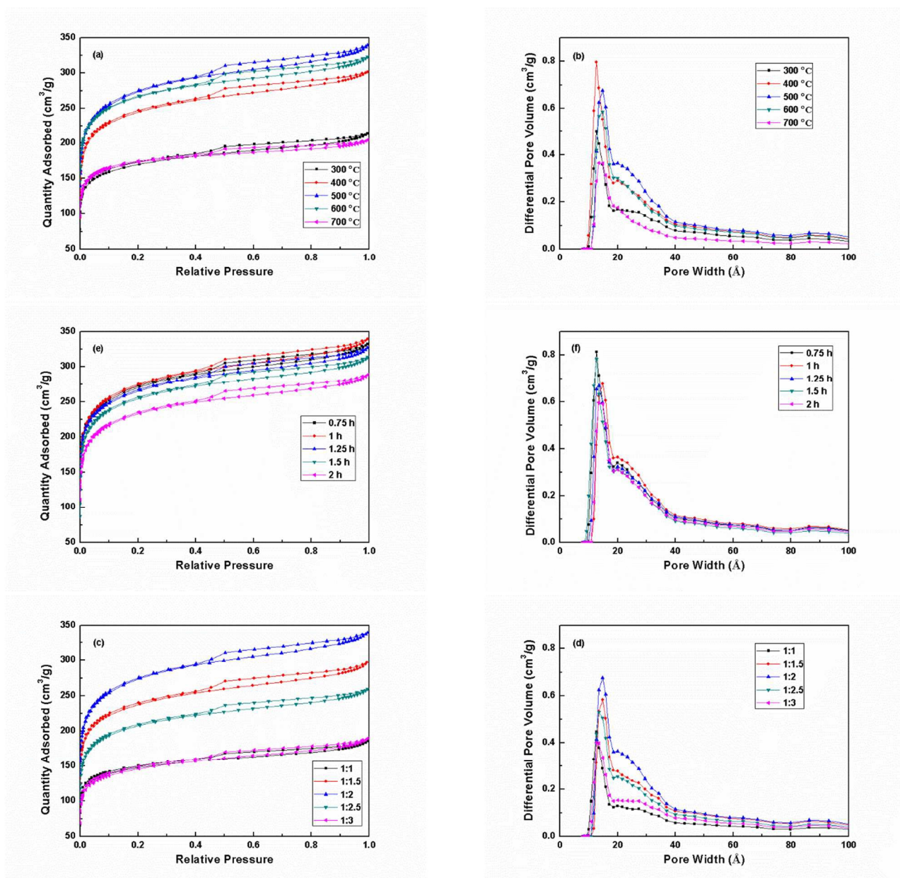
Fig. 4 N_2 adsorption-desorption isotherms and DFT pore size distributions for AC with different activation temperature (a, b), different impregnation ratios (c, d) and different activation time (e, f).
