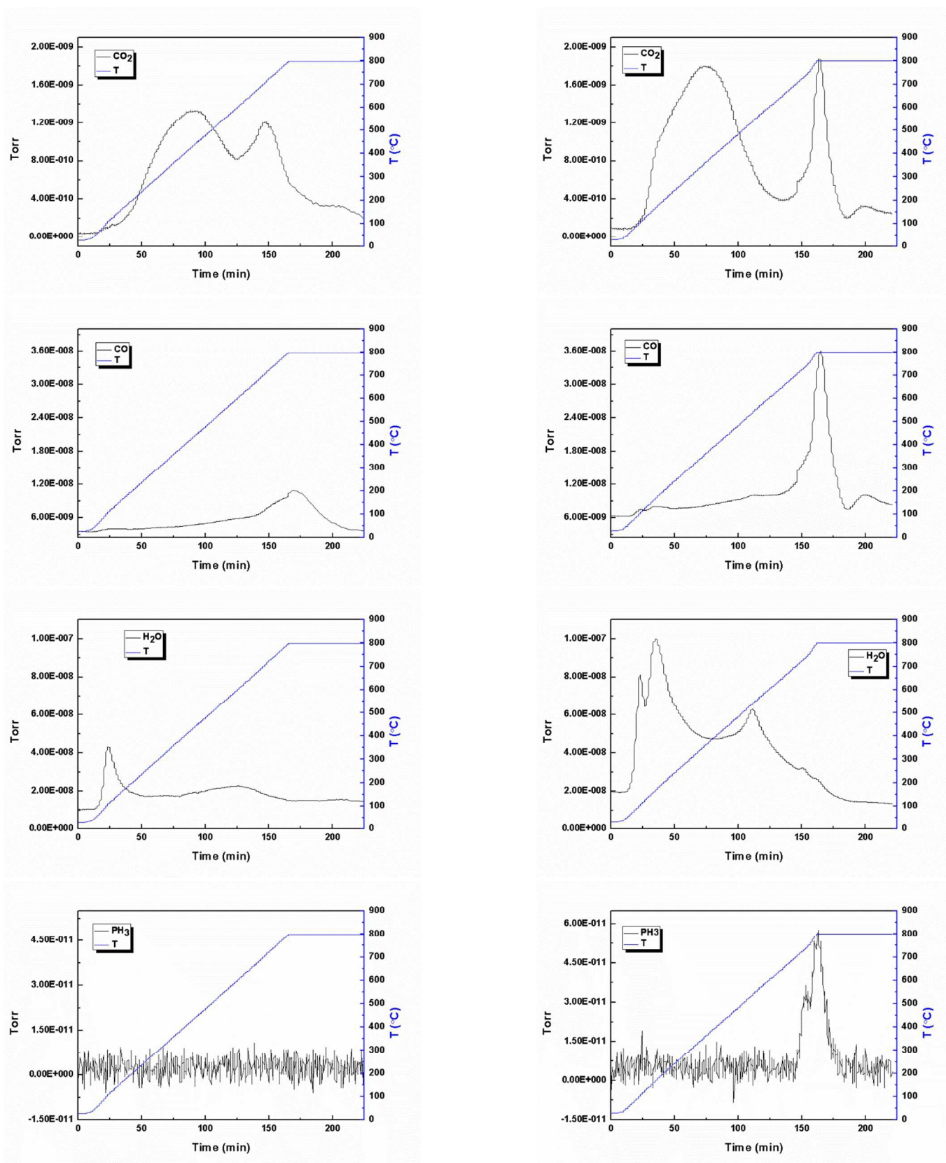
Fig. 5 CO 2 , CO, H 2 O and PH 3 TPD-MS spectra of BTRHR (left) and PBTRHR (right).
