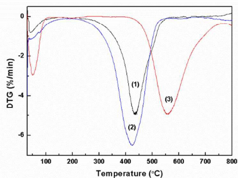
Fig. 7 TGA (a) and DTG (b) curves of (1) RHR, (2) BTRHR and (3) AC (1:2/1/500).
