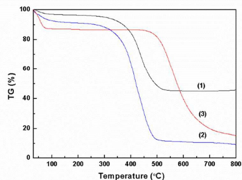
Fig. 6 TGA and DTG curves of BTRHR and PBTRHR.
