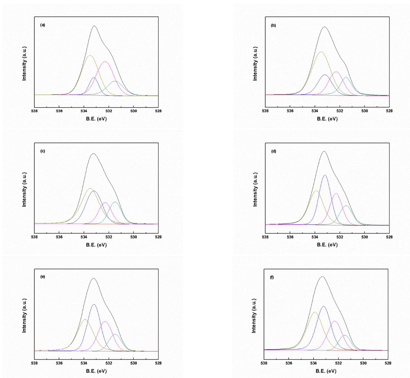
Fig. 9 XPS spectra of O1s peak of (a) PBTRHR and the samples (b-f) activated at 300, 400, 500, 600 and 700 °C.
