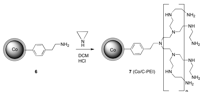
Scheme 2. Synthesis of poly(ethyleneimine) functionalised nanoparticles 7 . 36
