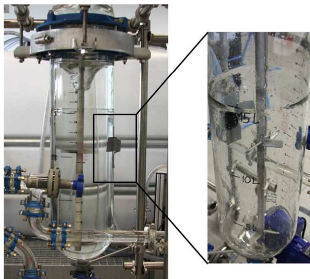
Figure 6. Large-scale experiment was performed in a reactor containing 20 L of an aqueous mercury solution ( 30 \mu\text{g}\cdot\text{L}^{-1} ). The extraction was done at RT during one hour using 0.3 \text{ mg NPs 7 per liter} , which were recovered by an external neodymium magnet (magnification, right picture).
