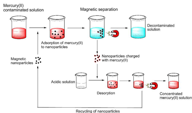
Figure 4. Recycling protocol for the extraction of mercury in tap water samples.
