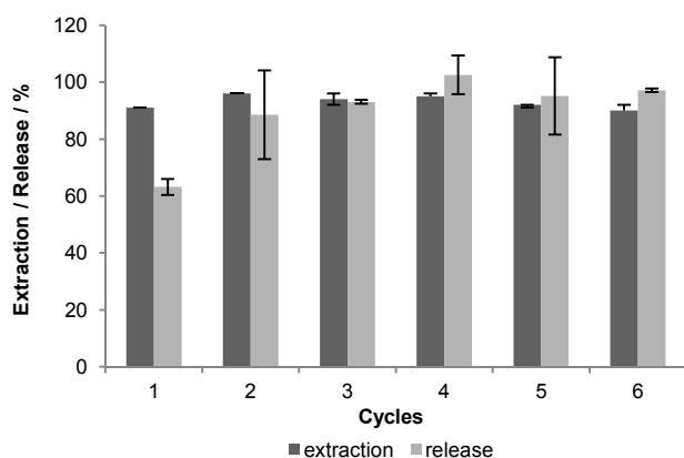
Figure 5. Reusability of Co/C-PEI 7 in six consecutive runs (extraction and subsequent release). Extraction: Co/C-PEI 7 (3 mg) were shaken in 100 mL of 2 \text{ mg}\cdot\text{L}^{-1} \text{Hg}(\text{II}) containing aqueous sample (pH 6.7) for 10 min. Release: 20 mL 0.5 M \text{H}_2\text{SO}_4 within 20 min.
