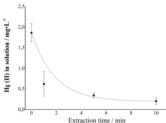
Figure 2. Mercury(II) extraction over time. 100 mL of an aqueous solution ( 1.64 \text{ mg}\cdot\text{L}^{-1} , solution pH 6.71), 3 mg Co/C-PEI nanoparticles 7 . The dashed curve represents the exponential decay fit of the data set (decay constant: 1.8 \pm 1.2 \text{ min}^{-1} ). After 10 min, the detection limit ( 100 \mu\text{g}\cdot\text{L}^{-1} ) of the ICP-OES analysis was reached.
