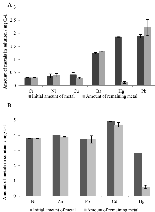
Figure 3. Selective extraction of Hg 2+ using Co/C-PEI 7 in the presence of competitive metal ions. A) 3 mg of NPs were used to decontaminate a 100 mL solution containing Hg 2+ , Cu 2+ , Pb 2+ , Ni 2+ , Ba 2+ and Cr 3+ in equimolar amounts (10 μM), solution pH 5.59; B) 3 mg of NPs were used to decontaminate an aqueous 100 mL solution containing Hg, Pb, Ni, Zn and Cd, solution pH 6.16.
