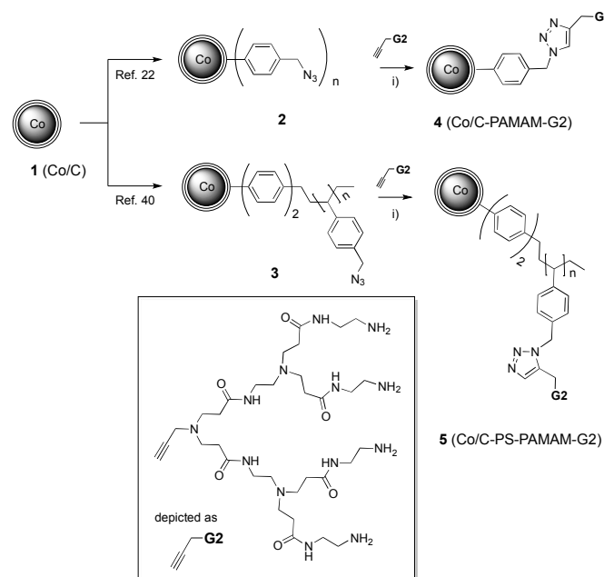
Scheme 1. Covalent immobilization of PAMAM dendron G2 on Co/C nanoparticles via click chemistry. Reagents and conditions: i) CuSO 4 •5H 2 O (10 mol%), Na ascorbate (30 mol%), THF-H 2 O (3 : 1), 24 h, RT.
