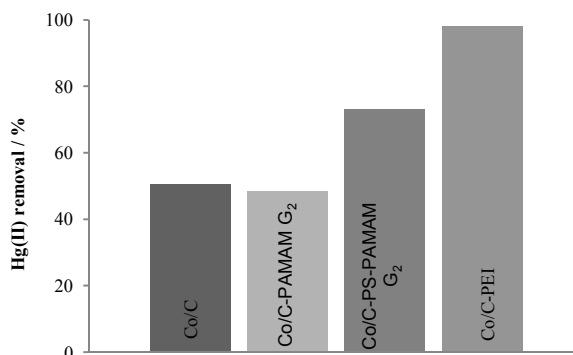
Figure 1. Comparison of the extraction capacity from the different nanobeads (cf Scheme 1, 2). Reaction conditions: 5 mg of NPs, 5 mL of \text{Hg}^{2+} solution ( 30 \text{ mg}\cdot\text{L}^{-1} ), 10 min extraction time, solution pH 6.53.
