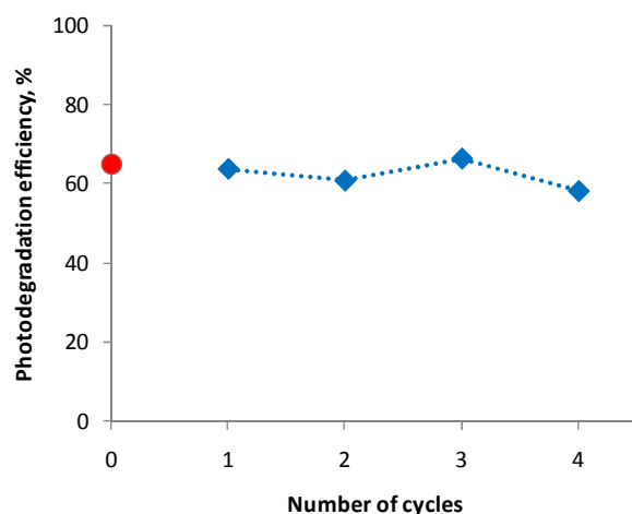
Fig. 9 Reusability of the LcTi(2:1)-800 catalyst under UVA illumination at room temperature.
