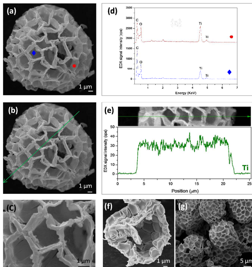
Fig. 3 (a-c) SEM images of the hollow micron-sized buckyball-like \text{TiO}_2 architectures calcined at 800^\circ\text{C} for 3h in air (LcTi(2:1)-800); (d) EDX spot analysis for the corresponding points ( i.e. , ● and ◆) given in (a); (e) Line-scan analysis of EDX Ti-signal (green curve) along the line depicted in (b); SEM images of (f) LcTi(3:2)-800 and (g) LcTi(3:2)-900.
