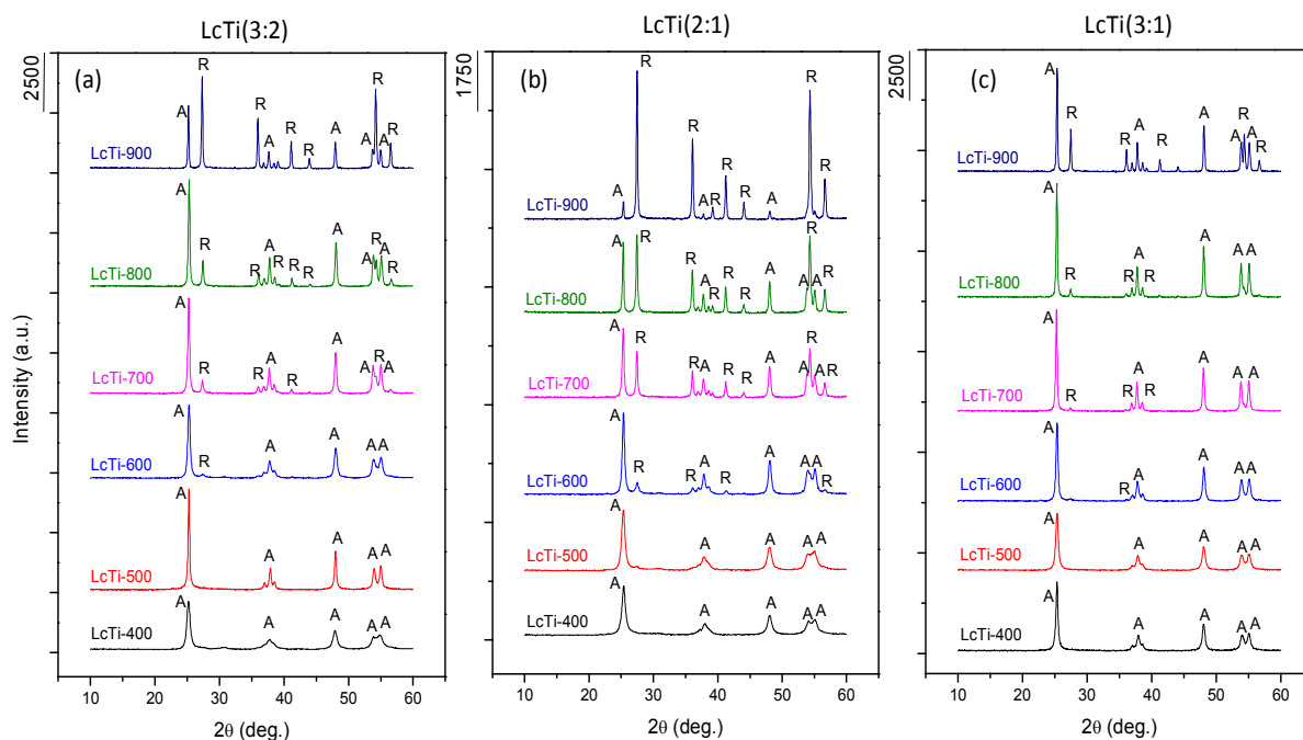
Fig. 5 XRD patterns of the micron-sized buckyball-like \text{TiO}_2 architectures synthesized via different precursor loadings: (a) LcTi(3:2); (b) LcTi(2:1) and (c) LcTi(3:1) which were calcined in air at 400, 500, 600, 700, 800, and 900 °C for 3 h after the synthesis. “A” and “R” stand for anatase and rutile phases, respectively.
