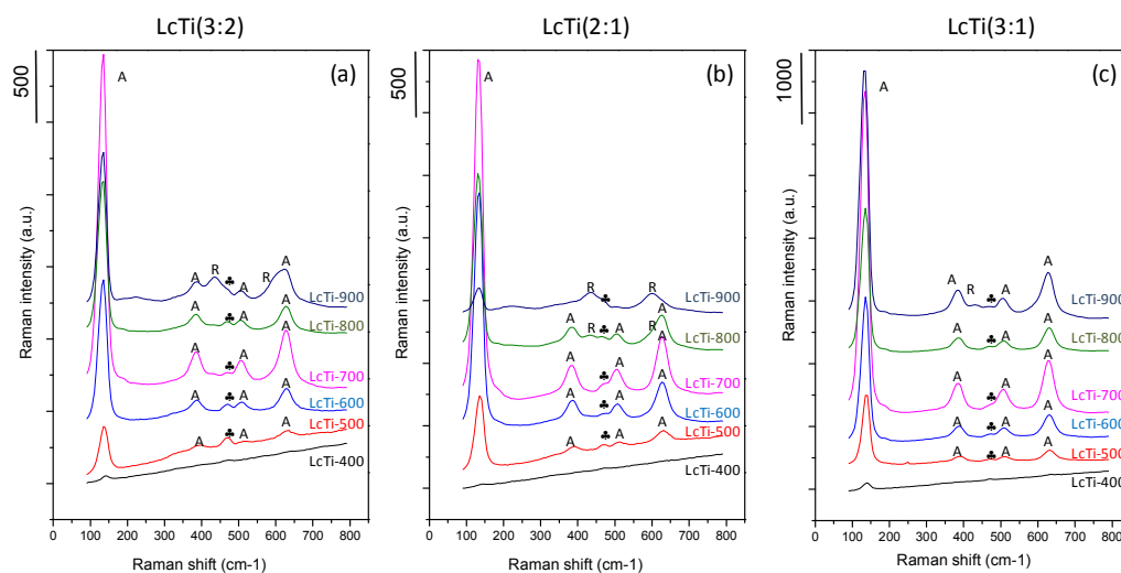
Fig. 7 Raman spectra of the micron-sized buckyball-like TiO 2 architectures synthesized via different precursor solutions: (a) LcTi(3:2); (b) LcTi(2:1) and (c) LcTi(3:1) which were calcined in air at 400, 500, 600, 700, 800 and 900 °C for 3 h after the synthesis; (A) TiO 2 anatase, (R) TiO 2 rutile, (♣) biopolymer.
