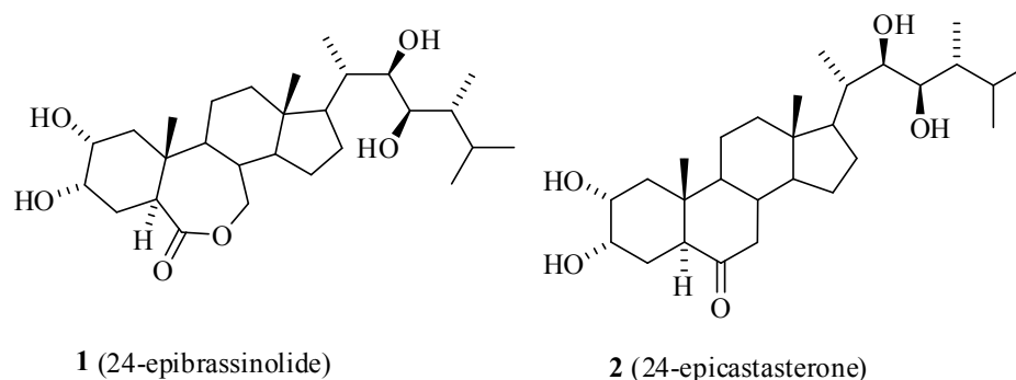
Figure 1 Structures of 24-epibrassinolide (24-epiBL) and 24-epicastasterone (24-epiCS)
