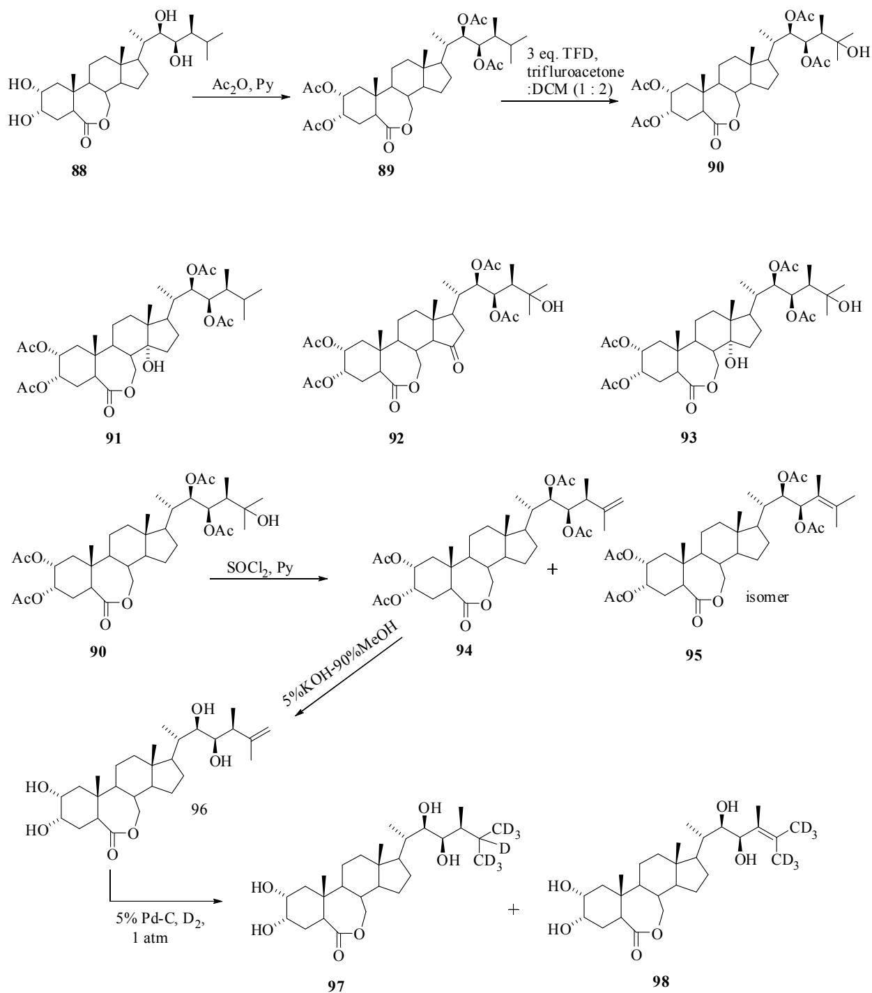
Scheme 11 Synthesis of [25, 26, 27- 2 H 7 ]BL.
