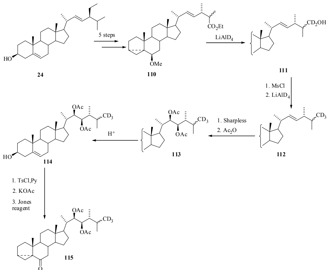
Scheme 13 Synthesis of cycloketone 115 from stigmasterol 24
