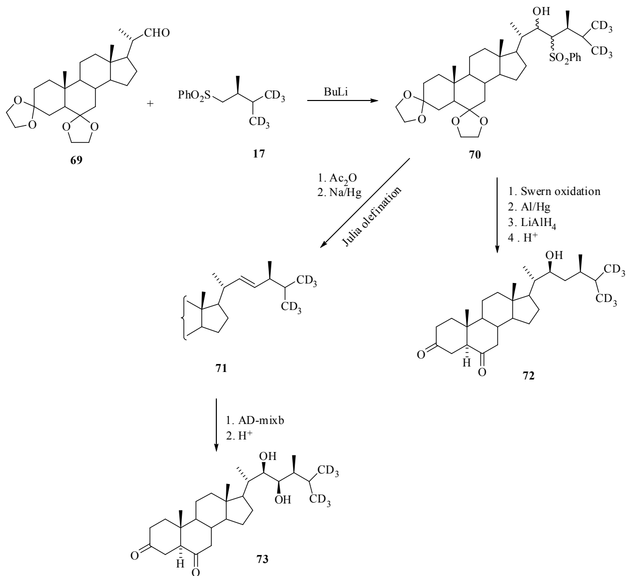
Scheme 9 Synthesis of 3,6-diketo-[26,27- ^2\text{H}_6 ] BRs
