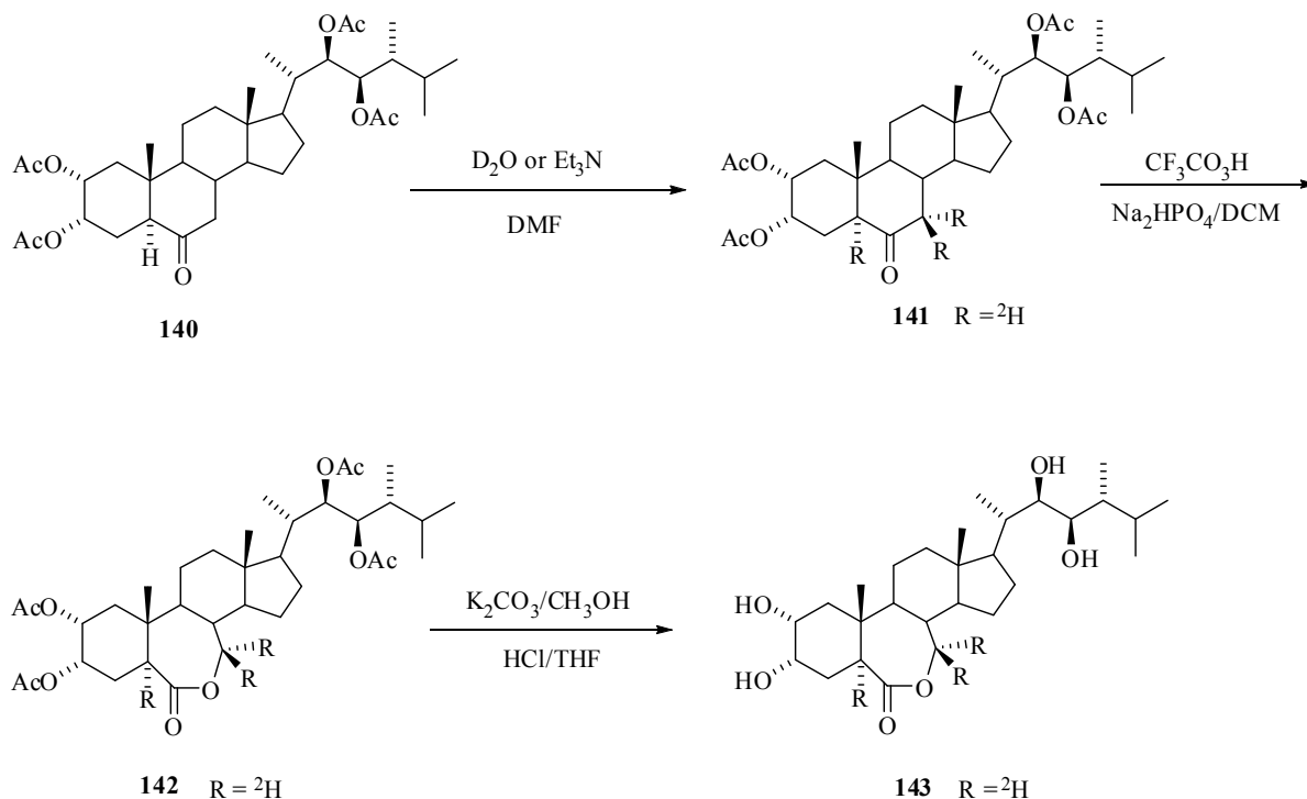
Scheme 18 Synthesis of 24-[5, 7, 7- 2 H 3 ] epiBL
