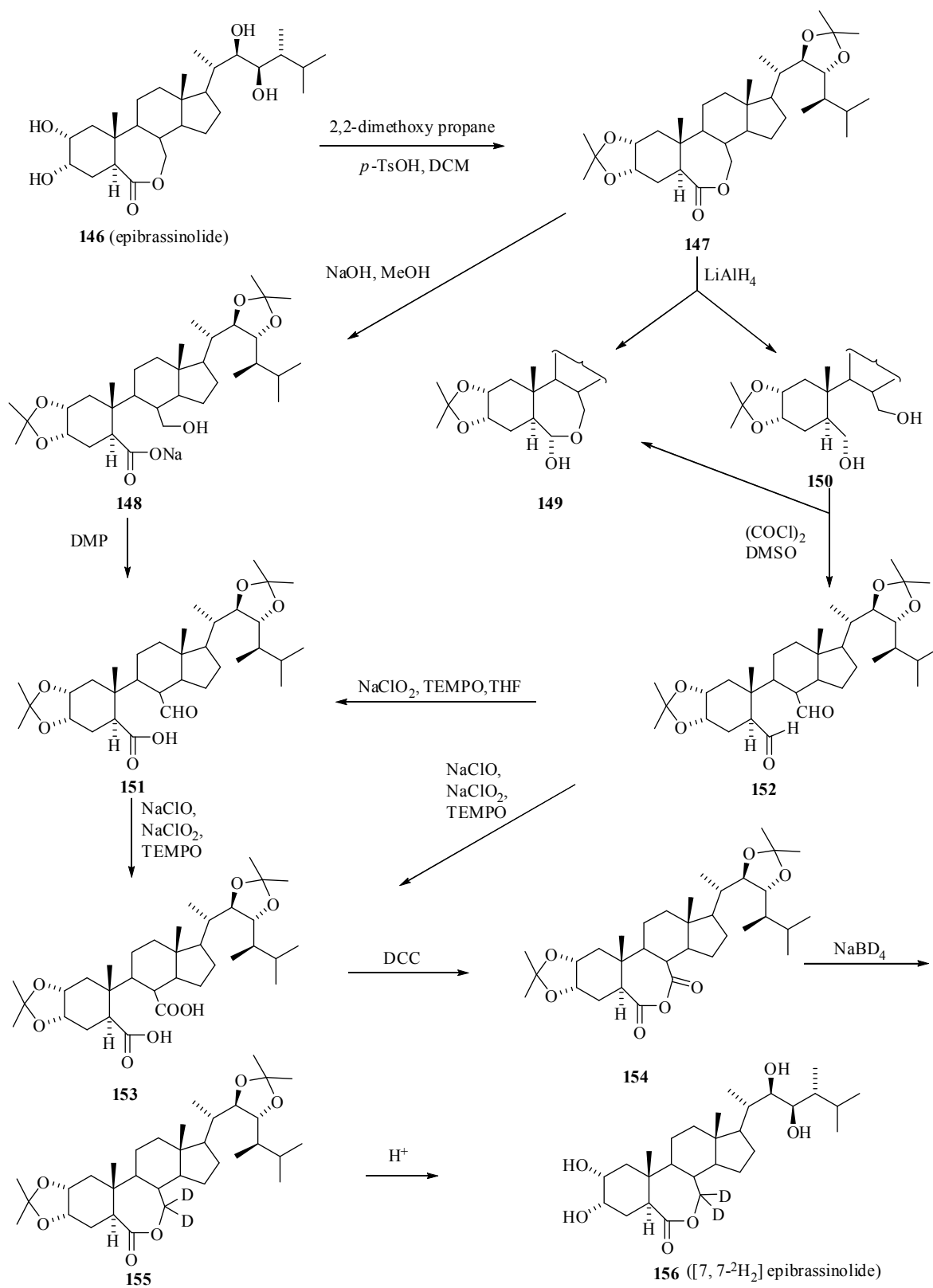
Scheme 19 Synthesis of 24-[7,7- ^2\text{H}_2 ]epiBL
