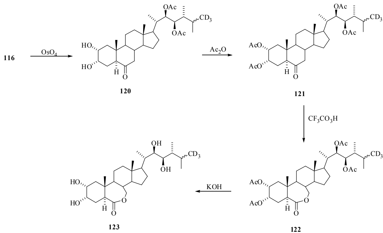
Scheme 15 Synthesis of deuterated 24-[26- ^2\text{H}_3 ] epiBL 123
