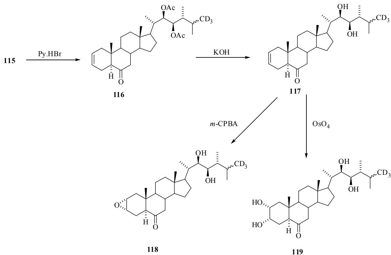
Scheme 14 Synthesis of 24-[26- ^2\text{H}_3 ] epiCS 119
