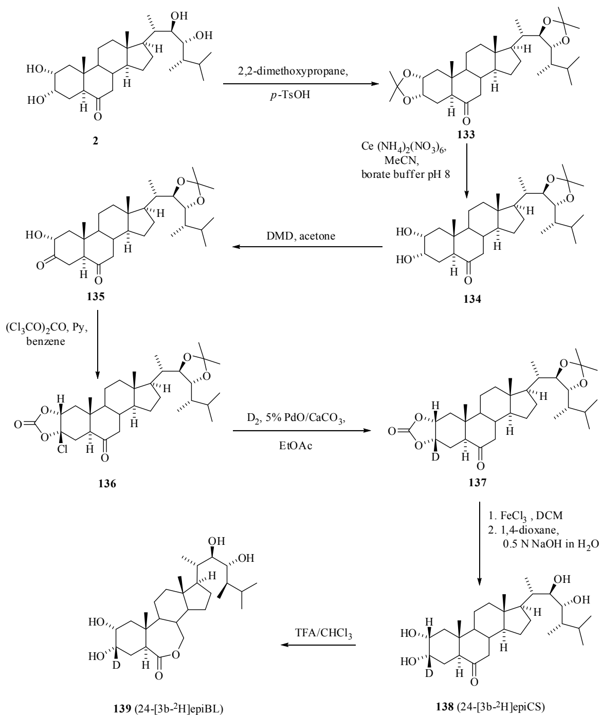
Scheme 17 Synthesis of 24-[3 \beta - 2 H]epiCS and 24-[3 \beta - 2 H]epiBL
