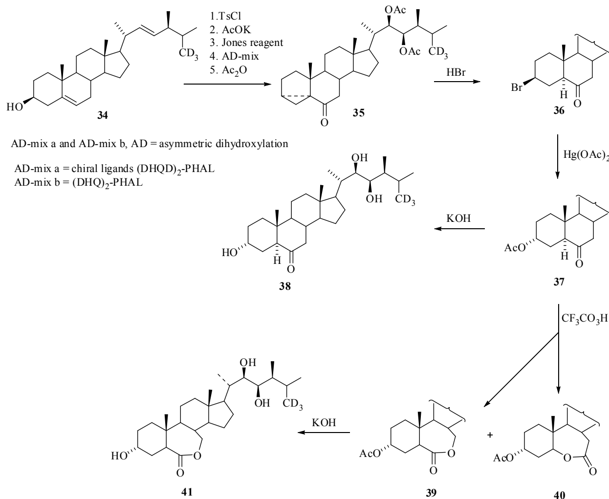
Scheme 4 Synthesis of [26- 2 H 3 ]TY 38 and related compounds
