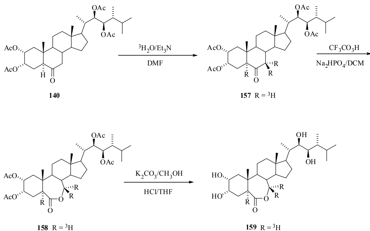
Scheme 20 Synthesis of 24-[5,7,7- 3 H]epiBL
