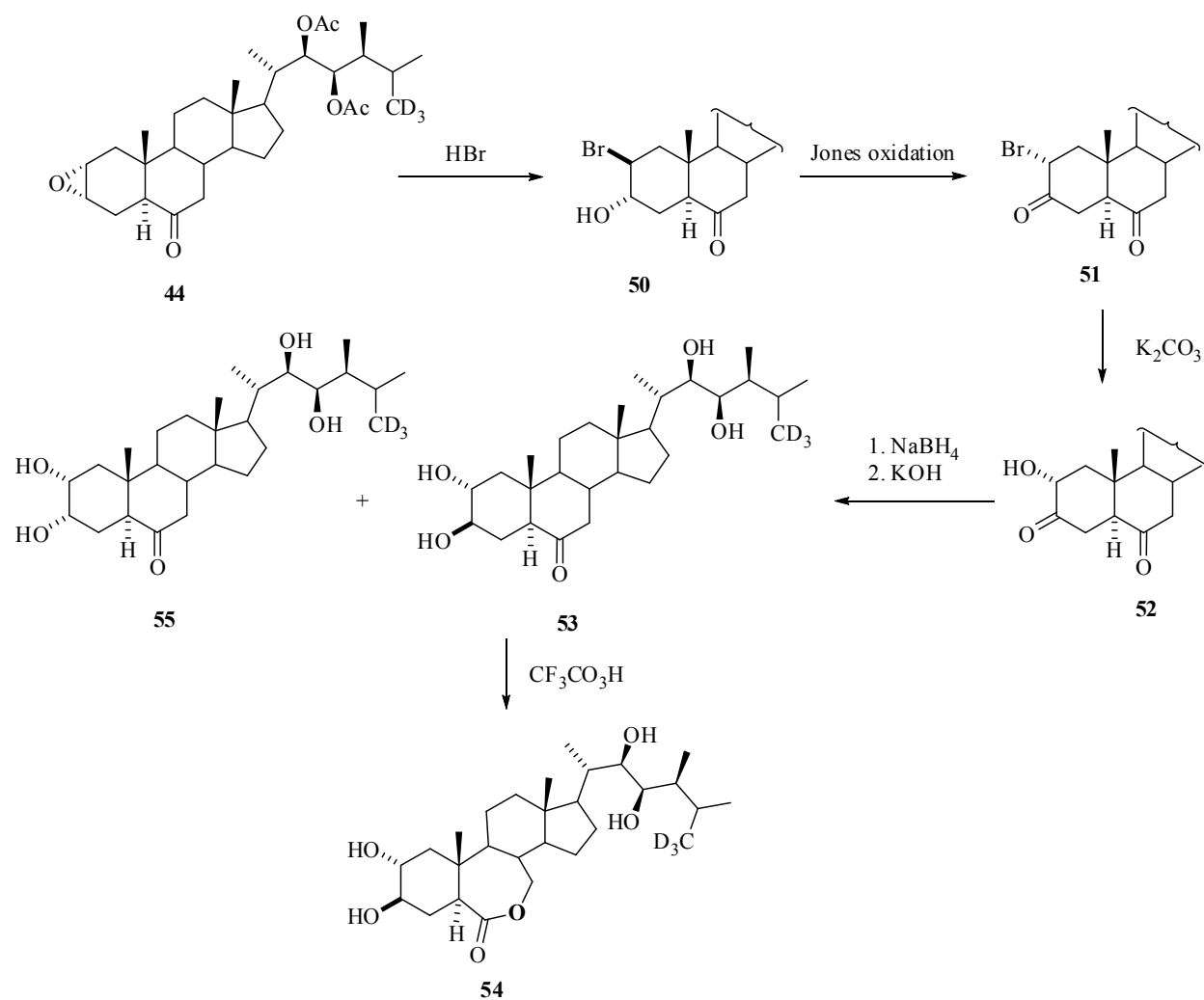
Scheme 6 Synthesis of deuterated tetra-hydroxyl BRs
