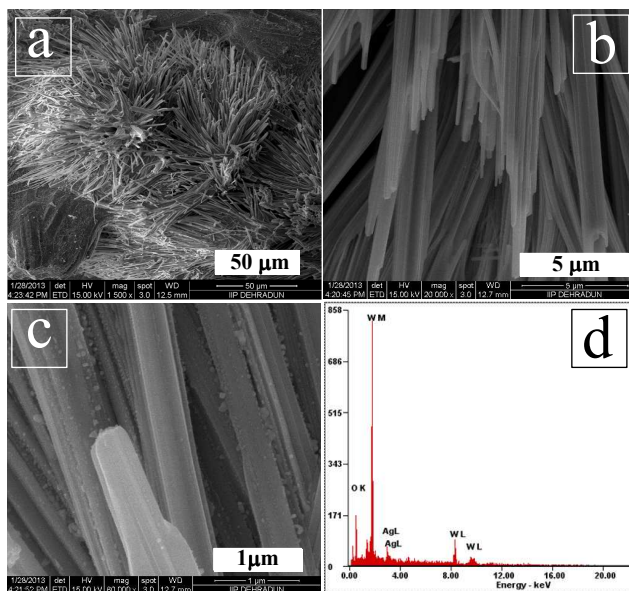
Fig. 2 SEM images (a-c) in increasing magnifications and (d) SEM-EDAX of \text{Ag}/\text{WO}_3 aloevera-type catalyst.
