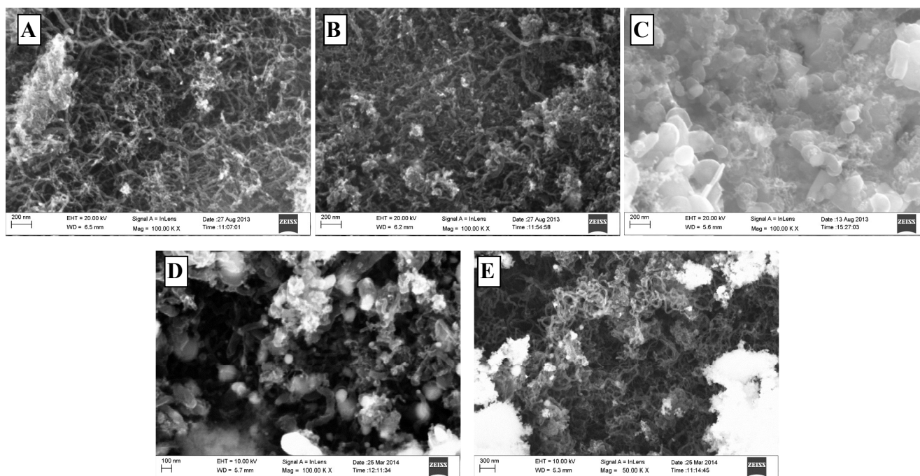
Fig. 8 SEM image of spent A. 4.3NiAl, B. 4.3CoAl, C. 4.3MoAl, D. 4.3NiSi, and E. 4.3NiZr. SR conditions: SCMR = 2.2, WHSV = 6.62 \text{ h}^{-1} .
