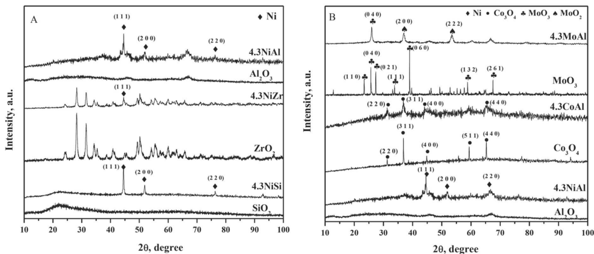
Fig. 9 Powder XRD pattern of spent A. 4.3NiAl, 4.3NiZr, and 4.3NiSi and B. 4.3NiAl, 4.3CoAl, and 4.3MoAl. SR conditions: 923 K, SCMR = 2.2, and WHSV = 6.62 \text{ h}^{-1} .
