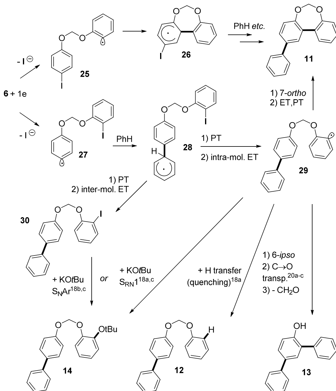
SCHEME 4. Likely Mechanism for the Multi-BHAS to form 11–14.
