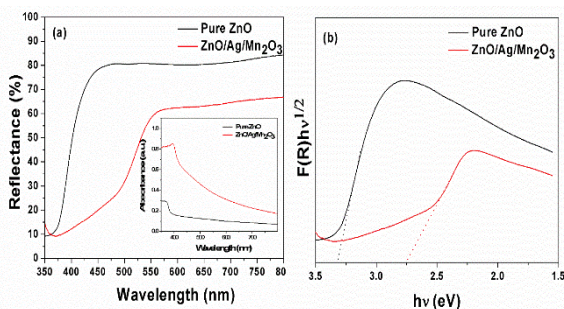
Fig. 4 (a) UV-vis diffuse reflectance spectra, and the inset shows UV-vis absorption spectra, and, (b) F(R)hv^{1/2} vs hv plot of the pure ZnO and ternary ZnO/Ag/Mn 2 O 3 nanocomposite.
