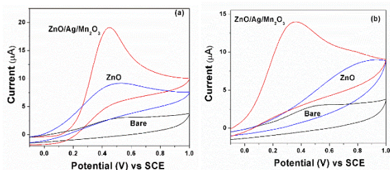
Fig. 6 The CV results of bare GCE and pure ZnO nanorods as well as ternary ZnO/Ag/Mn 2 O 3 nanocomposite modified GCE in presence of 3 mM (a) UA and (b) AA.
