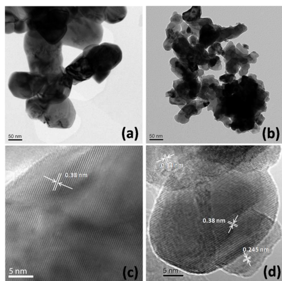
Fig. 3. TEM images and HRTEM images of LBC0 (a,c) and LBC3 (b,d).
