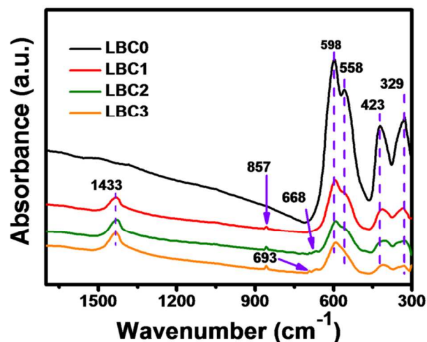
Fig. 2. FT-IR spectra of fresh LBC oxides.
