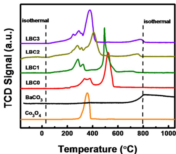
Fig. 4. H 2 -TPR profile of the LBC oxide catalysts. The display values of Co 3 O 4 were equal to the real values * 0.15.
