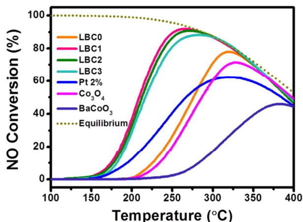
Fig. 6. NO removal percentage as a function of temperature and composition: 400 ppm NO, 10% O 2 and a balance of N 2 .
