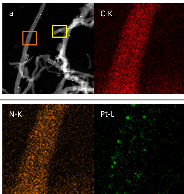
Fig. 2 TEM dark-field image and STEM-EDX elemental mappings of 1% Pt/N-CNTs(5.74) catalyst. (a) Dark-field image. Other images represent the elemental STEM-EDX mapping images of measured C-K intensity, N-K intensity, and Pt-L intensity, which are obtained from the light brown square. The yellow rectangle is used to correct any drift in the sample.
