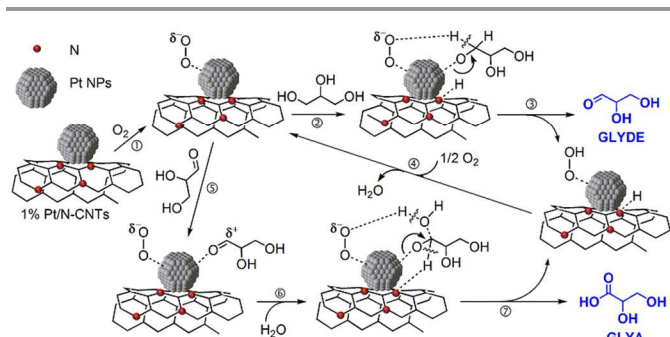
Scheme 1 Proposed reaction pathway for glycerol oxidation catalyzed by Pt/N-CNTs.
