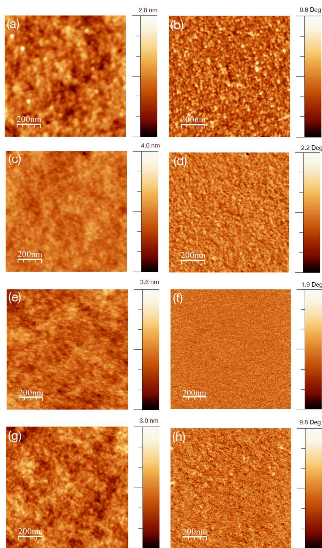
Figure 7. Tapping mode AFM height and phase images (1 \mu\text{m} \times 1\mu\text{m} ) of blends films spin-coated from chlorobenzene: o -DCB of (a and b) truxTTF:PC 61 BM (1:6), (c and d) truxTTF:PC 71 BM (1:6), (e and f) truxTTF-CO:PC 61 BM (1:4) and (g and h) truxTTF-CO:PC 71 BM (1:4).
