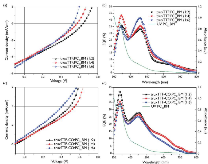
Figure 5. (a) Current density-voltage ( J-V ) curves of the blend truxTTF:PC 61 BM, (b) EQE plots for the devices derived from truxTTF:PC 61 BM at different w/w ratio, (c) current density-voltage ( J-V ) curves of the blend truxTTF-CO:PC 61 BM and (d) EQE plots for the devices derived from truxTTF-CO:PC 61 BM at different w/w ratio.
