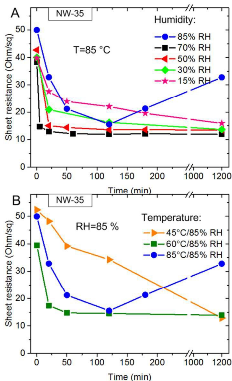
Figure 4. Sheet resistance vs. annealing time for AgNW-35 films: (A) at constant temperature of 85 °C and different RH values; (B) at constant RH of 85 % and different temperatures. The blue line represents the sample treated under 85 °C/ 85 % RH similarly in both frames.
