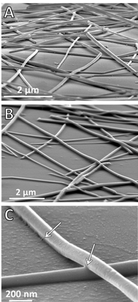
Figure 2. SEM images of Ag90-NW directly after spraying (A), after 180 min annealing at 85 °C / 85 % RH (B) and 85 °C / 70 % RH (C) demonstrating changes in the morphology of the NW networks. White arrows in (C) highlight the closer alignment of the wires and a better contact to the substrate.
