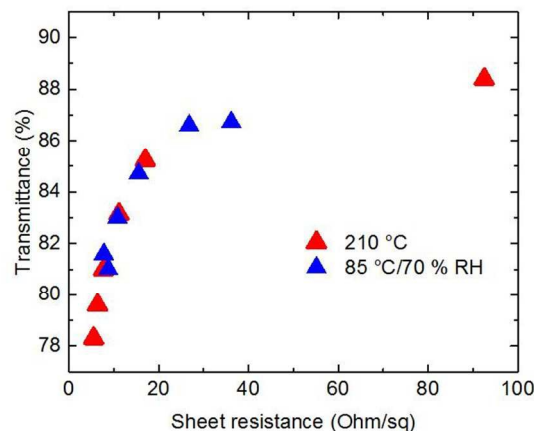
Figure 5. Plot of total transmittance at 550 nm vs sheet resistance for NW-90 films heated for 90 min at 210 °C on a heating plate (red triangles) and that of films treated for 120 min at 85 °C/70 % RH in a climate chamber (blue triangles).
