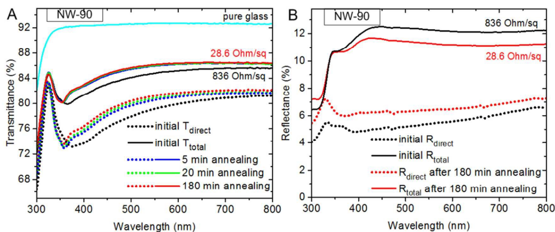
Figure 1. (A) Total transmittance spectra of pure glass substrate (the same before and after annealing) as well as total and direct transmittance spectra of an NW-90 electrode heated at 85 °C/ 85 % RH. (B) Total and direct reflectance of the same NW-90 electrode before and after annealing at 85 °C/ 85 % RH. Total and direct transmittance spectra of an NW-90 electrode heated at 85 °C/ 85 % RH.
