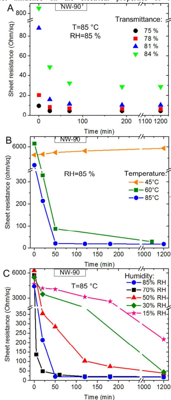
Figure 3. Sheet resistance vs. annealing time for NW-90 films: (A) at different coverages during annealing at 85 °C and 85 % RH; (B) at constant RH of 85 % and different temperatures; and (C) at constant temperature of 85 °C and different RH values. The blue line representing the sample treated under 85 °C / 85 % RH is the same in both B and C frames.
