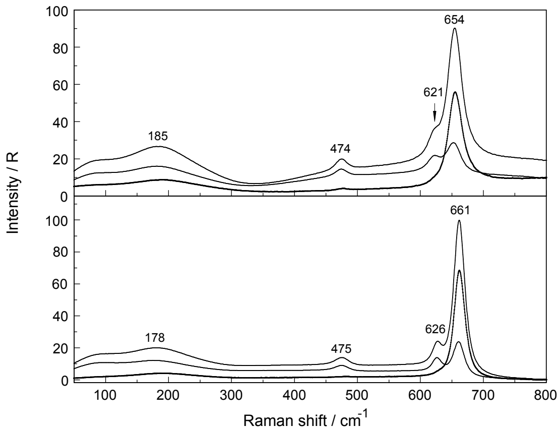
Figure 2. Comparison of the Raman scattering profiles in R-format: polarized, depolarized and isotropic (presented as a thick, dark line) of \text{NaCH}_3\text{CO}_2(\text{aq}) . Upper panel: 2.183 \text{ mol}\cdot\text{L}^{-1} solution in water and lower panel: 3.944 \text{ mol}\cdot\text{L}^{-1} solution in heavy water. Note, that the deformation mode, \delta\text{CO}_2 , for \text{CH}_3\text{CO}_2^-(\text{aq}) appears at 654 \text{ cm}^{-1} and for \text{CH}_3\text{CO}_2^-(\text{D}_2\text{O}) at 661 \text{ cm}^{-1} .
