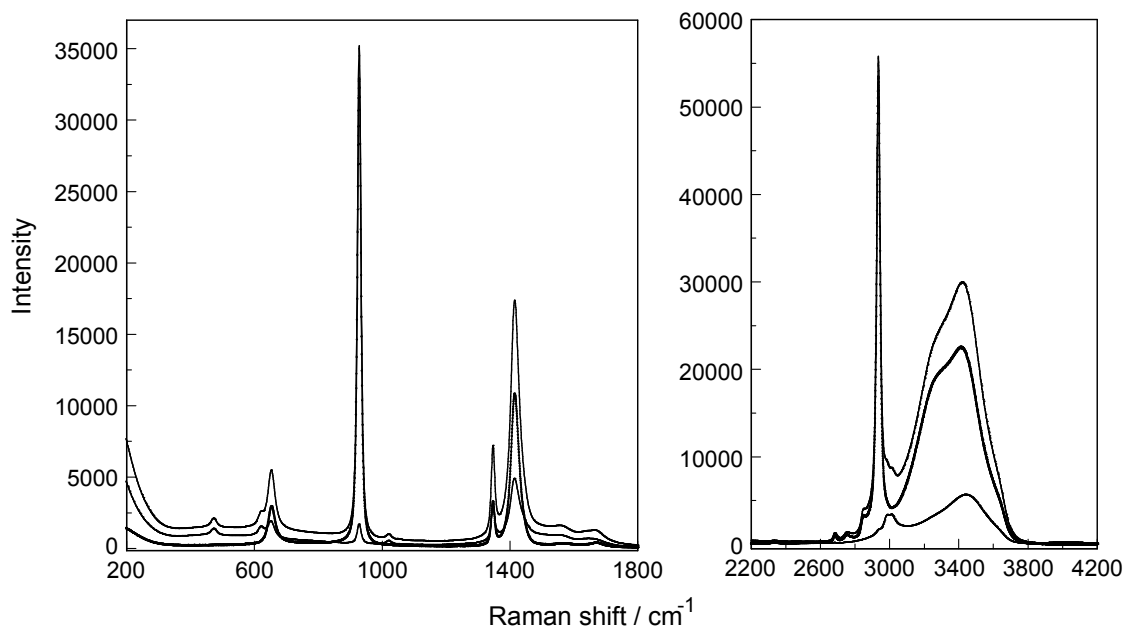
Figure 4. Overview Raman spectrum of an aqueous solution of \text{NaCH}_3\text{CO}_2 ( 5.022 \text{ mol}\cdot\text{L}^{-1} ). All scattering orientations are given: polarized, depolarized and isotropic which is presented as a thick, dark line. Left panel: Raman bands of \text{CH}_3\text{CO}_2^-(\text{aq}) in the wavenumber range from 200\text{-}1800 \text{ cm}^{-1} . Right panel contains spectra in the wavenumber range from 2400\text{-}4000 \text{ cm}^{-1} . Along with the \nu \text{ C-H} modes of \text{CH}_3\text{CO}_2^-(\text{aq}) the very broad O-H stretching band of water is given.
