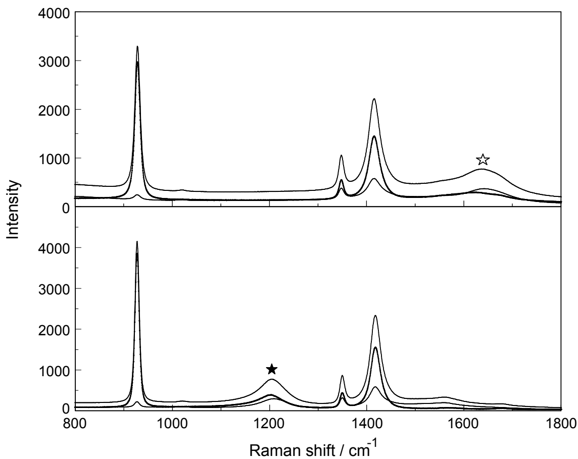
Figure 6. Comparison of the Raman scattering profiles (polarized, depolarized and isotropic scattering, which is shown as a thick, dark line) of \text{NaCH}_3\text{CO}_2 solutions in water and heavy water. Upper panel: 1.209 \text{ mol}\cdot\text{L}^{-1} solution in water; Lower panel: 0.790 \text{ mol}\cdot\text{L}^{-1} solution in heavy water. Note, the deformation mode, \delta\text{H}_2\text{O} , for water at 1641 \text{ cm}^{-1} (upper panel, open star) and at 1206 \text{ cm}^{-1} for \text{D}_2\text{O} , the deformation mode of heavy water in the lower panel (black star).
