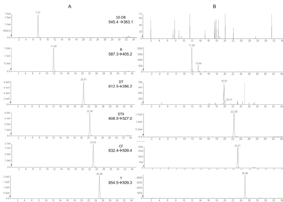
Figure 3 Identification chromatograms for taxane traces, A: Standard solution at 1.2 \mu\text{g mL}^{-1} with 1 \mu\text{g mL}^{-1} DTX as IS. B: C. avellana sample with 1 \mu\text{g mL}^{-1} DTX. 120x85mm (300 x 300 DPI)
