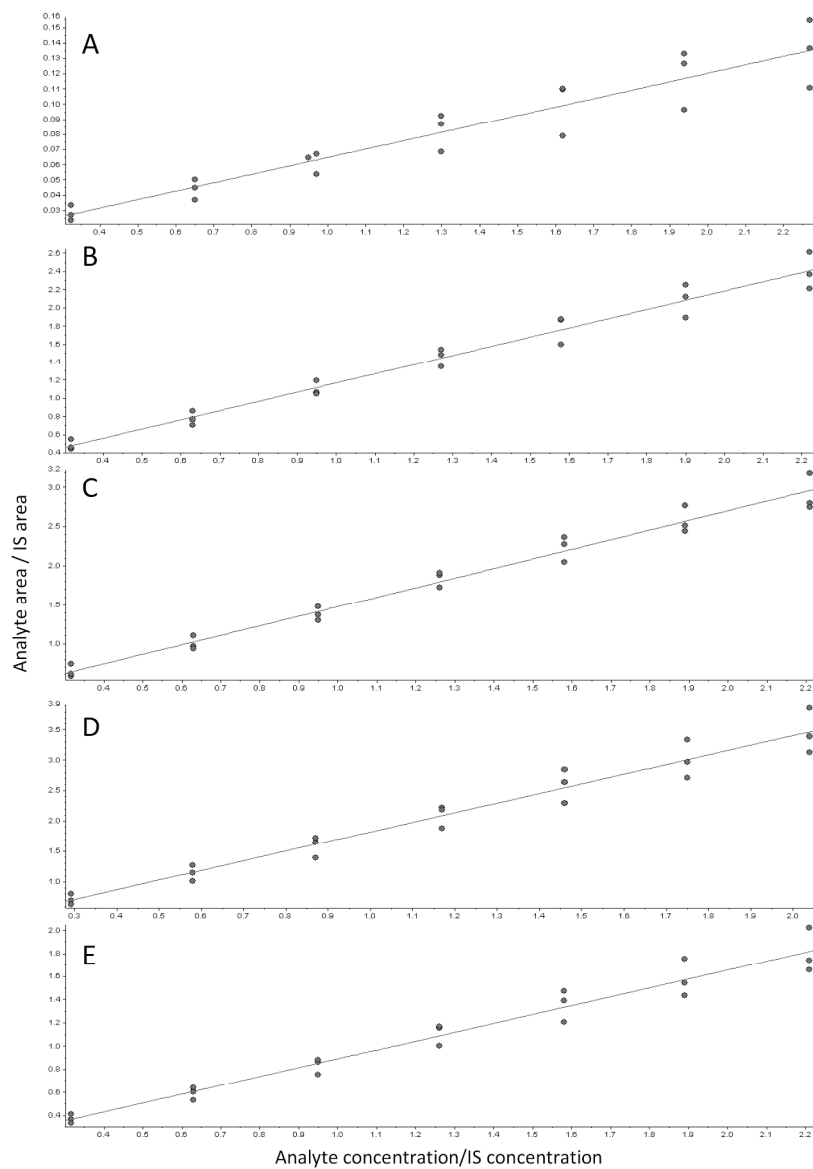
Figure 2: Standard curves of 10-deacetylbaccatin III (A), baccatin III (B), 10-deacetyltaxol (C), cephalomannine (D) and taxol (E) in the range of 0.3-2.1 \mu\text{g mL}^{-1} . 1 \mu\text{g mL}^{-1} of DTX was added as the internal standard (IS), therefore the analyte area/IS area vs analyte concentration is represented.
