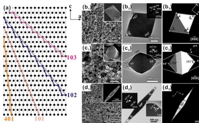
Fig. 7. (a) Schematic model of stepwise \{101\} , \{102\} , \{103\} , and \{401\} surfaces projected along the [010] direction. SEM images, TEM images, and ideal models of \text{TiO}_2 particles with exposed (b 1 –b 3 ) \{102\} , (c 1 –c 3 ) \{103\} and (d 1 –d 3 ) \{401\} facets. Reprinted with permission from ref.64 and ref.66. Copyright 2012 Wiley-VCH and 2013 Wiley-VCH.
