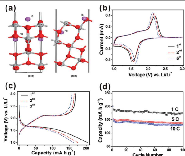
Fig. 4. (a) Scheme of the anatase lattice with insertion of Li ions (purple spheres) between octahedral voids. The initial and final states of Li + are indicated as 'IS' and 'FS', respectively. Grey spheres: titanium, red spheres: oxygen. Reprinted with permission from ref. 53. Copyright 2010 Royal Society of Chemistry. (b) Representative CVs at a scan rate of 0.2 mV s -1 for the first, second, and fifth cycles. (c) Charge-discharge profiles at a current rate of 5 C (850 mA g -1 ) for the first, second, and fifth cycles. (d) Cycling performance at different C rates. All of the measurements were conducted using a voltage window of 1.0-3.0 V. Reprinted with permission from ref. 54. Copyright 2010 American Chemical Society.
