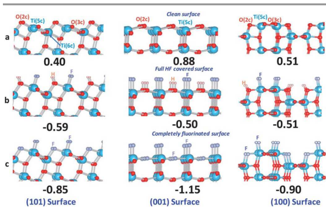
Fig. 6 DFT calculated surface energies (the unit is \text{J m}^{-2} ) and structures for different stages of HF interaction with single crystal anatase \text{TiO}_2 ( \{101\} (left) ( \{001\} (middle) and ( \{100\} (right) surfaces. (a) Clean surfaces; (b) full HF-covered surfaces; (c) complete fluorinated surfaces. All structures are optimized structures. Reprinted with permission from ref. 135. Copyright 2012 Royal Society of Chemistry.
