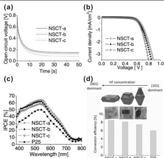
Fig. 3. (a) Open-circuit voltage decay profiles, (b) dark current potential scans and (c) IPCE spectra of DSSCs based on the A-TiO 2 crystals with different percentages of {001} ( i.e. , NSCT-a, NSCT-b, NSCT-c) and P25. (d) Schematic of the correlation between the particle morphology and the photovoltaic conversion efficiency of the A-TiO 2 crystals with different percentages of {001} facets. Reprinted with permission from ref. 107. Copyright 2011 Wiley-VCH.
