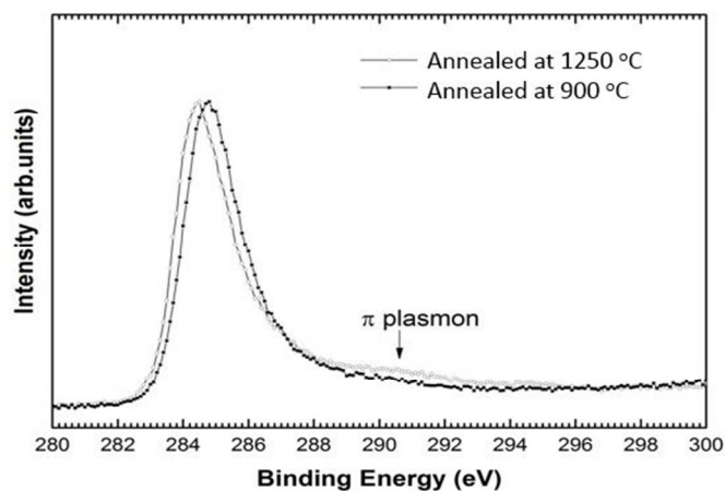
Figure 7. C 1s XPS spectra of carbon monoliths containing DND which underwent pyrolysis at temperatures of 900 °C and 1250 °C. Spectra were obtained in normal emission geometry at a photon energy of 1486.6 eV.
