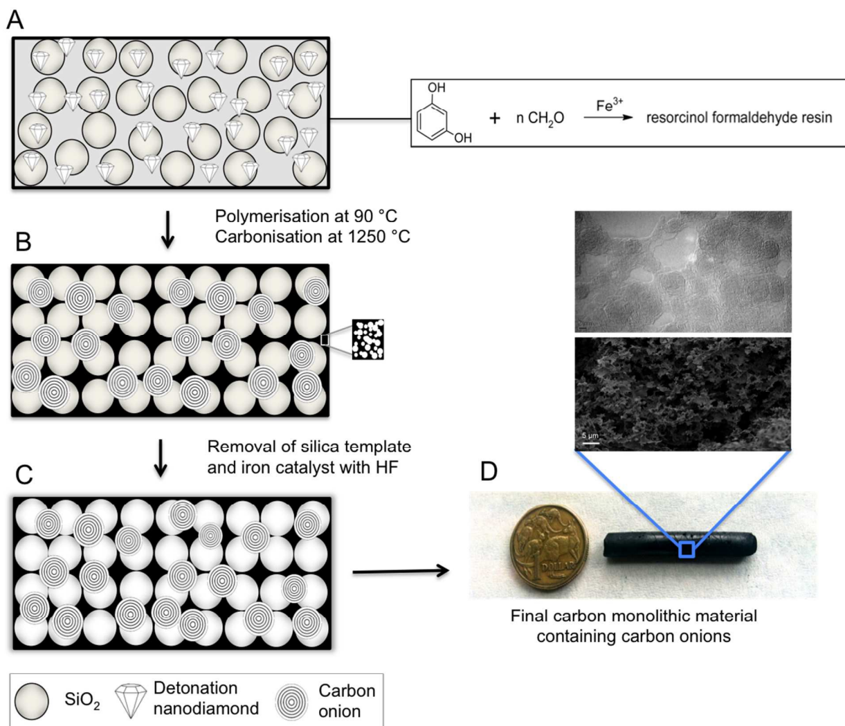
Figure 1. Scheme for fabrication and pyrolysis of carbon monolithic composites.
