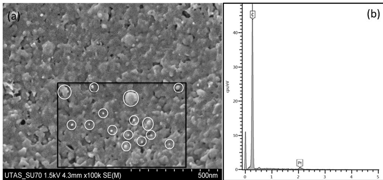
Figure 4. (a) High magnification (x 100 K) image of the wall of monolith macropore, showing the presence of a mesoporous structure (with surviving surface detonation nanodiamonds highlighted between 10 and 100 nm). (b) EDX spectrum for carbon monolith showing presence of carbon only (Pt from splutter coating).
