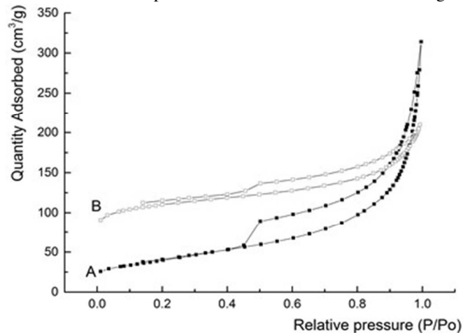
Figure 8. Nitrogen adsorption/desorption isotherms for A - Bare carbon monolith (prepared without the addition of carbon nanoparticles for comparative purposes) and B - carbon on carbon monolithic composite containing carbon onions.
