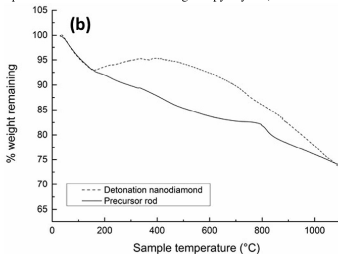
Figure 2. (a) SEM image taken of a cross section of the precursor rod containing silica particles, and DND, before carbonisation at 1250 °C. (b) Thermogravimetric analysis curves for detonation nanodiamond (DND), and precursor rod containing the resorcinol-formaldehyde resin, with \text{Fe}^{3+} catalyst, silica particles, and DND.
