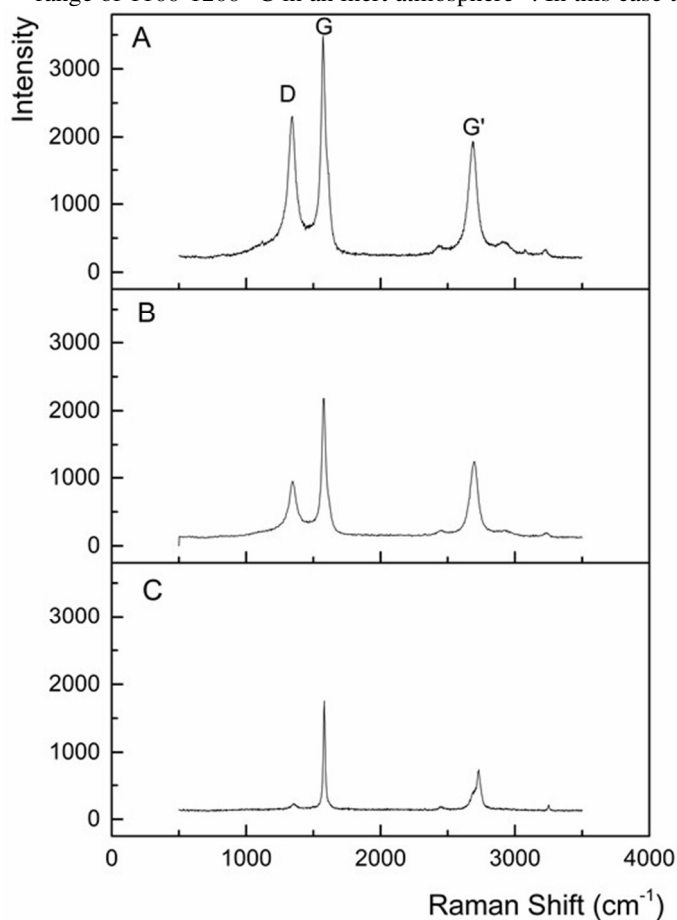
Figure 6. Raman spectra for A - bare carbon monolith (prepared without addition of carbon nanoparticles for comparative purposes), B - carbon on carbon monolithic composite, and C - commercial graphite. Both carbon monolithic materials underwent pyrolysis at 1250 °C.
