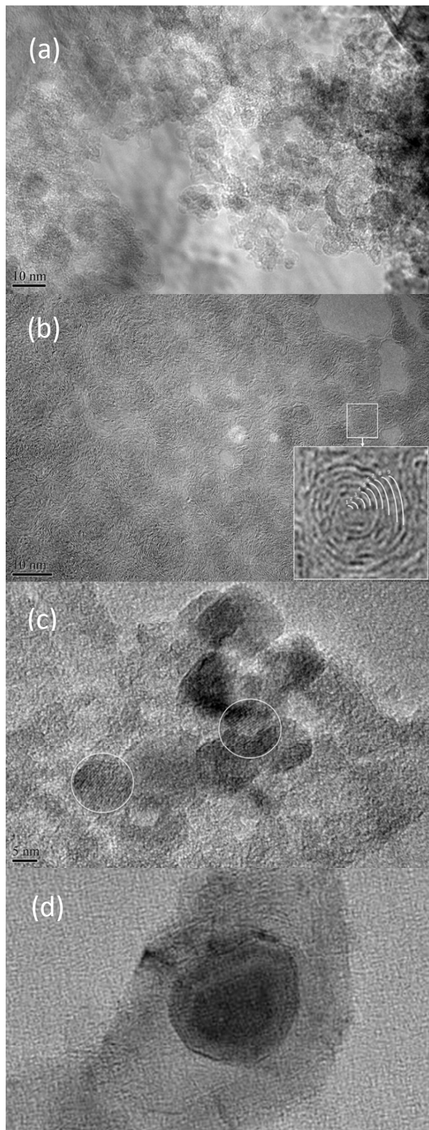
Figure 5. TEM images of porous graphitic carbon composites. (a) Amorphous carbon, (b) carbon onions resulting from the thermal annealing of detonation DND under N 2 at 1250 °C, (c) DND remains intact within the porous graphitic carbon composite following pyrolysis up to 900 °C, (d) DND showing surface graphitisation following pyrolysis up to 900 °C.
