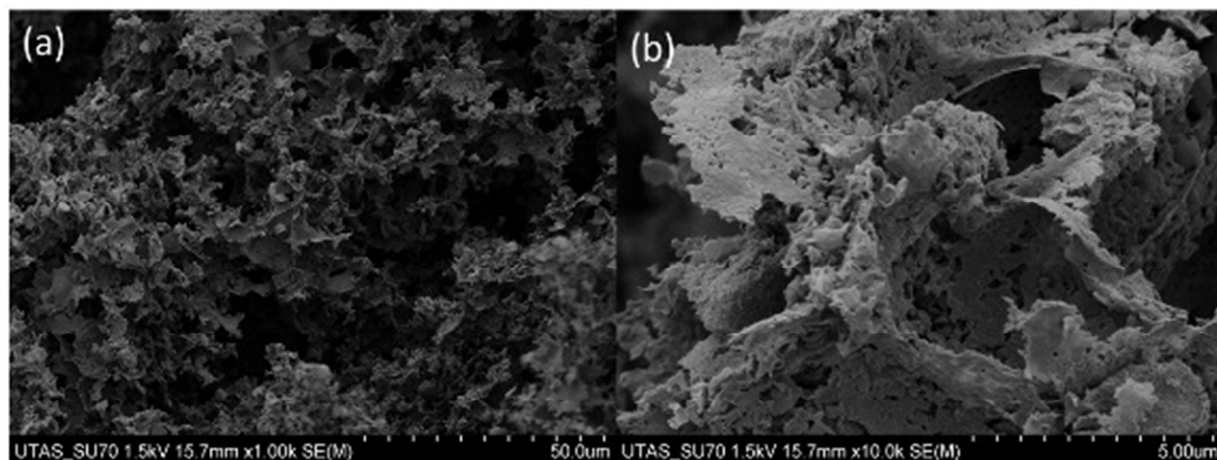
Figure 3. SEM images showing the porous graphitic carbon monolith with carbon onions. (a) Macroporous network mag X 1 K, (b) mag X 10 K.
