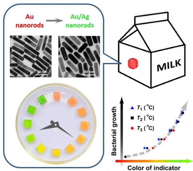
Fig. 9 A kinetically programmable time-temperature indicator. (Left) Chronochromism during the overgrowth of silver shell layer on gold nanorods. (Bottom right) A temperature-independent correlation between the indicator color and the magnitude of microbial growth in perishable.
