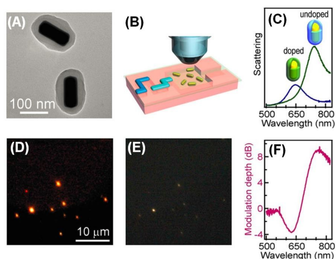
Fig. 4 Gold nanorod/polyaniline core/shell nanostructures as resonance-coupling-based plasmon switches. (A) Transmission electron microscope image of the core/shell nanostructures. (B) Schematic illustration of core/shell nanostructures embedded in a microfluidic chip for optical measurement. (C) Dark-field scattering spectrum for a representative nanostructures before and after proton doping. (D,E) Dark-field scattering photograph observed before and after proton doping, respectively. (F) Modulation depth of the plasmon switch. (Reprinted with permission from Ref. 83)
