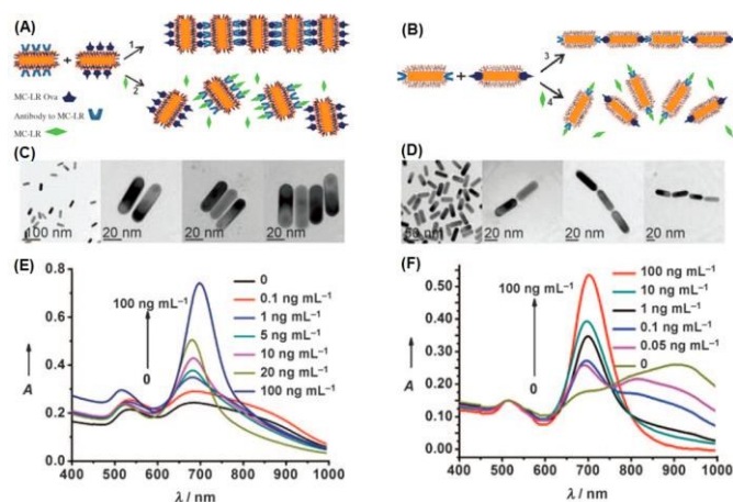
Fig. 6 (A,B) Schematic illustration of assembling gold nanorods into side-by-side and end-to-end aggregates, respectively. (C,D) Corresponding transmission electron microscope images of individually dispersed nanorods and assembled ones. (E,F) Extinction spectra when nanorod aggregates disassembled. (Reprinted with permission from Ref. 86)
