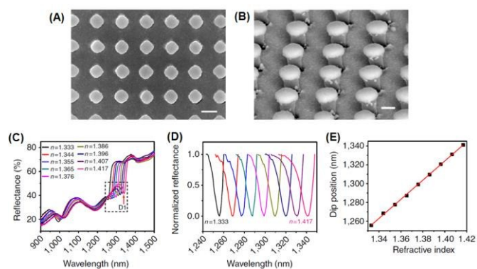
Fig. 2 Sensing platform comprising gold mushroom arrays. (A, B) Scanning electron microscope images of gold mushroom arrays. (C) Reflectance spectra of gold mushroom arrays immersed in solutions with varying refractive indexes ( n ). (D) Spectral profiles for D1 after normalization. (E) The linear correlation between the dip wavelength and the refractive index. (Reprinted with permission from Ref. 67)
