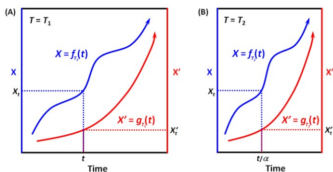
Scheme 3 Illustration of the correlatability between two monotonic process functions, namely, X = f(t) and X' = g(t) , when (A) T = T_1 and (B) T = T_2 .
