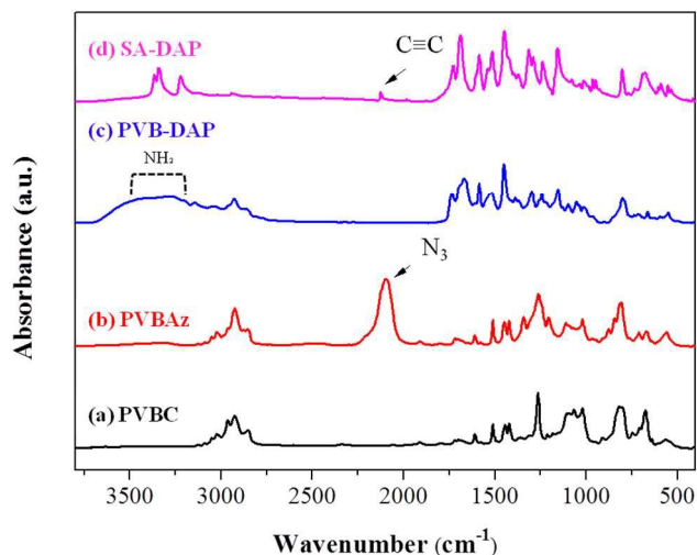
Fig. 1: FTIR spectra of (a) PVBC, (b) PVBAz, (c) PVB-DAP, and (d) SA-DAP
