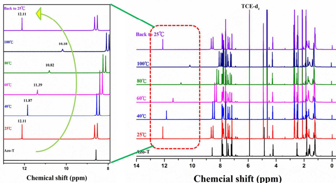
Fig. 8: ^1\text{H} NMR spectra of Azo-T/SA-DAP supramolecular complex plotted with respect to temperature at a concentration of 10 wt %
