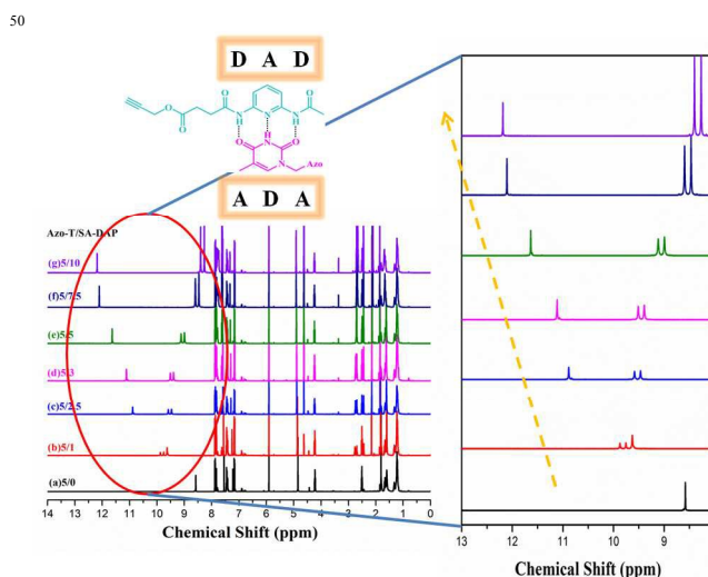
Fig. 7: ^1\text{H} NMR titration spectrum of the Azo-T/SA-DAP complex
