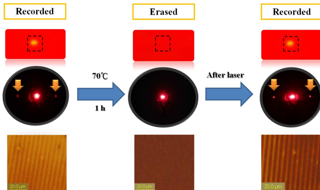
Fig. 13: Photographs and diffraction patterns of supramolecular films after erasing and subsequent laser-recording
