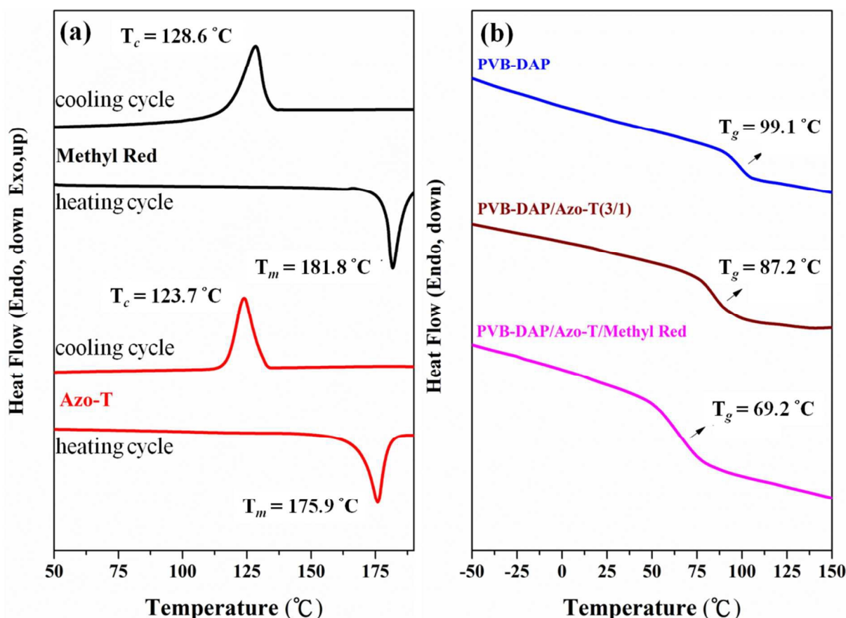
Fig. 11: (a) DSC cooling/heating cycles for Methyl Red (black curve) and Azo-T (red curve). (b) DSC thermograms for PVB-DAP, PVB-DAP/Azo-T, and PVB-DAP/Azo-T/Methyl Red recorded during the second heating cycle
