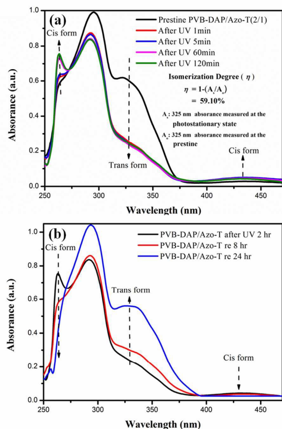
Fig. 9: UV-Vis spectra of the PVB-DAP/Azo-T supramolecular complex (a) before and after illumination with a UV lamp at 365 nm and (b) after standing in the dark at room temperature
