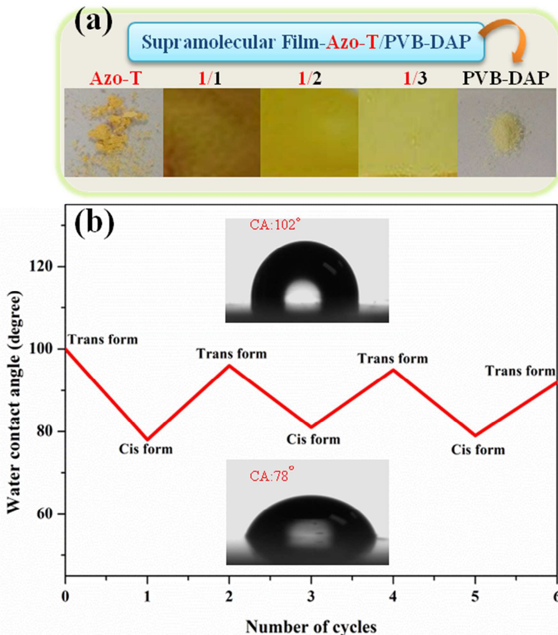
Fig. 10: (a) Comparison of the morphologies and colors of films of Azo-T, PVB-DAP, and their supramolecular complexes formed at various ratios. (b) WCAs of PVB-DAP/Azo-T supramolecular complexes after several cycles of UV irradiation and leaving in the dark
