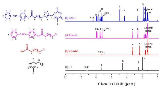
Fig. 5: 1 H NMR spectra of (a) PT, (b) Az-acid, (c) Azo-Az, and (d) Azo-T in CDCl 3
