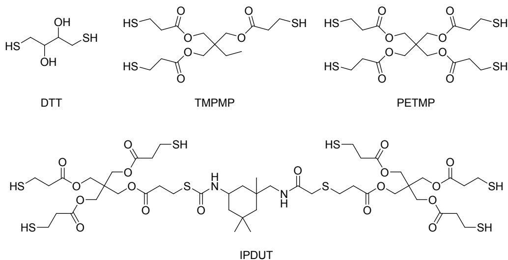
Fig. 18 Examples of thiols typically used as additives in photopolymerizable formulations.
