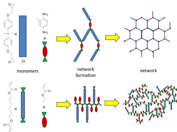
Fig. 4 Network formation via step-growth polymerization of epoxy thermosets (above) and radical chain growth of acrylates (below).
