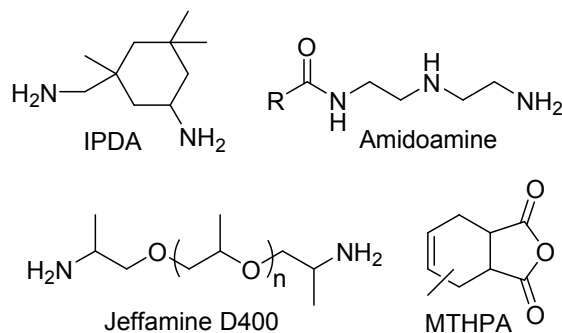
Fig. 17 Amine and anhydride curing agents claimed to give tougher epoxy polymers.
