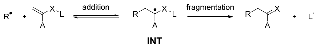
Scheme 5 General mechanism for addition-fragmentation chain transfer (AFCT).
