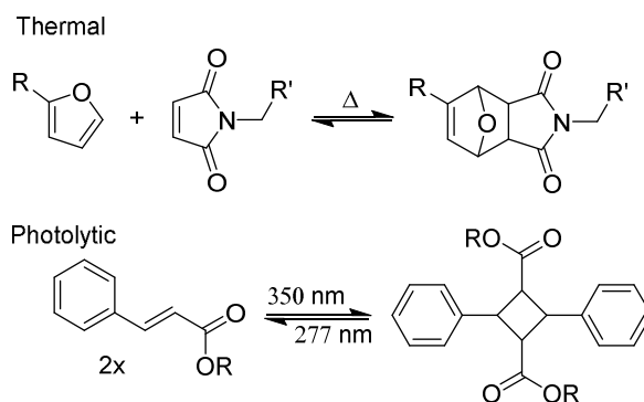
Scheme 6. Thermal and photolytic methods of intrinsic self-healing
