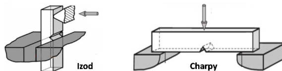
Fig. 2 Schematics of Izod and Charpy impact testing setups.
