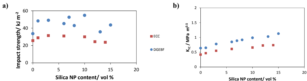
Fig. 10 Toughening effects of SNPs on epoxy thermosets.
