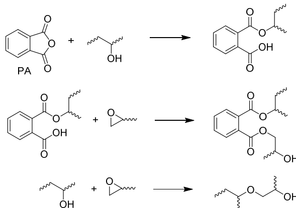
Scheme 2 Crosslinking of epoxy thermosets with acid anhydrides. 20
