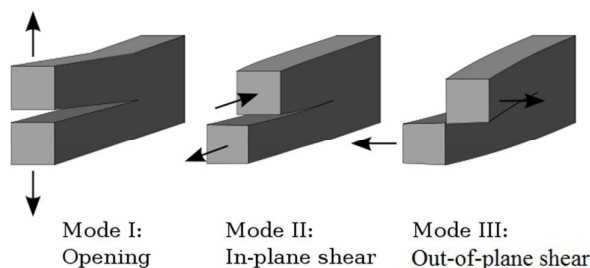
Fig. 3 Modes of crack propagation.
