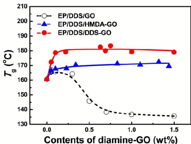
Fig. 6 Glass transition temperatures ( T_g ) of EP/DDS/diamine-GO nanocomposites. T_g was estimated from the second heating DSC results of EP/DDS/diamine-GO mixture..
