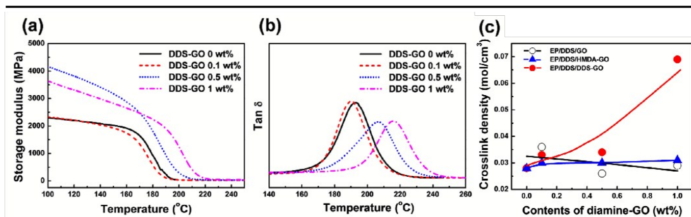
Fig. 7 DMA results of EP/DDS/diamine-GO nanocomposites. (a) Storage modulus, (b) \tan\delta , and (c) crosslink density of the EP/DDS/diamine-GO nanocomposites. Samples were tested in a temperature range of 30 to 260 °C at a scanning rate of 3 °C/min. The crosslink density was calculated using storage modulus and \tan\delta in the rubbery region of EP/DDS/diamine-GO nanocomposites.
