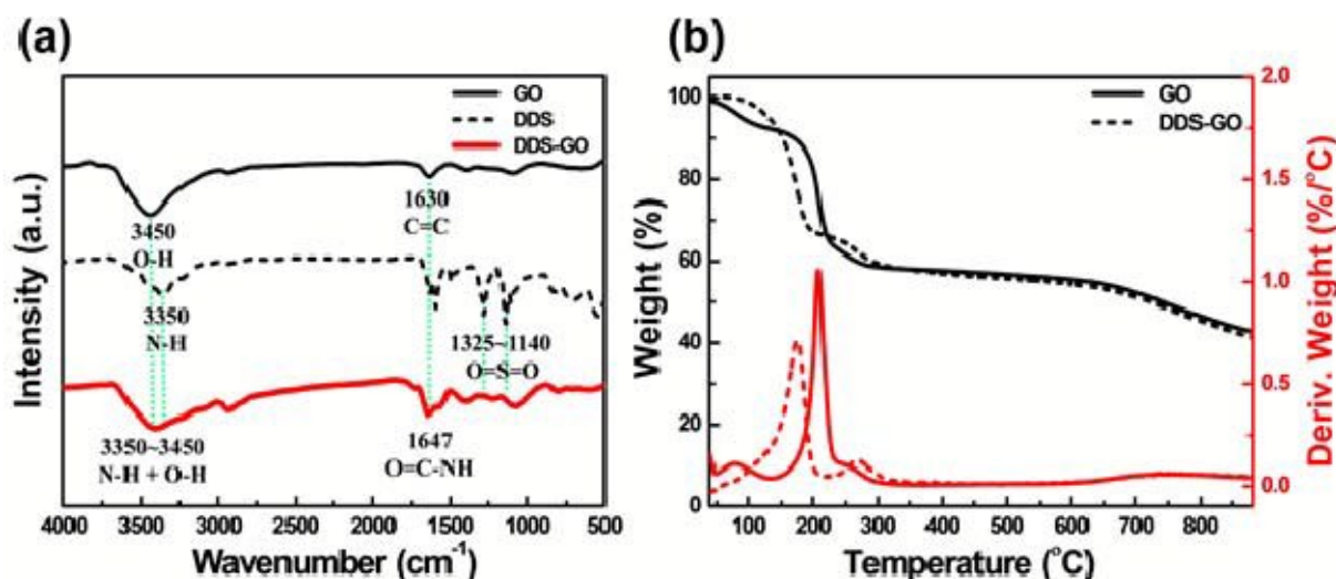
Fig. 2 (a) FT-IR spectra of GO, DDS, and DDS-GO. (b) TG-DTA curves of GO and DDS-GO during heating up to 900 °C in a N 2 atmosphere.
