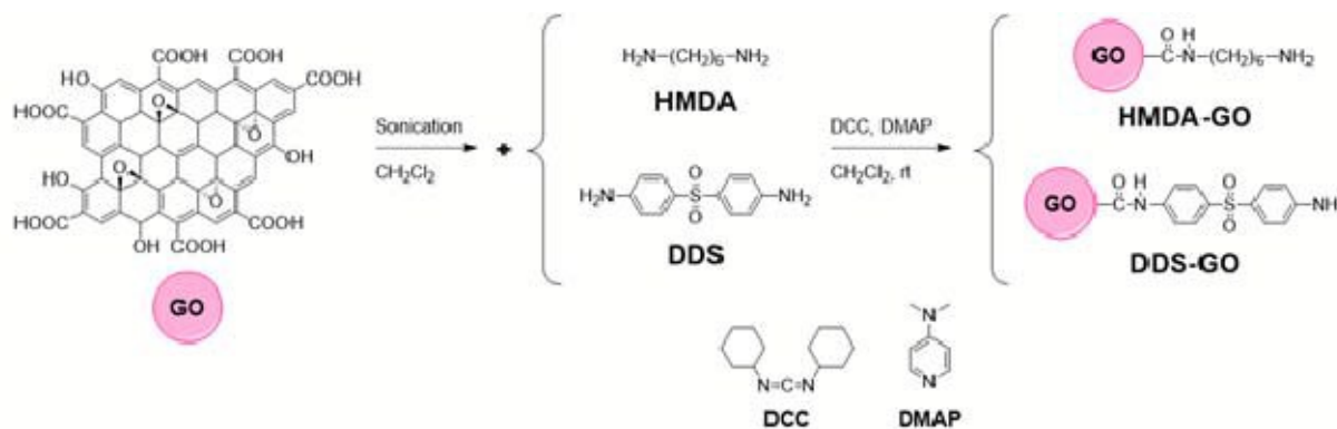
Fig. 1 Synthetic routes for diamine-GO derivatives
