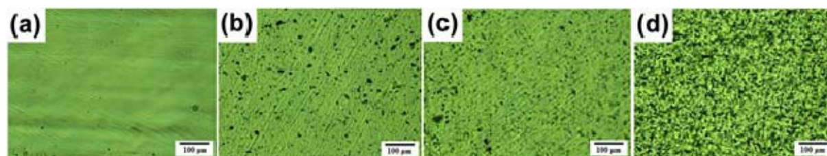
Fig. 5 Optical microscope photographs of EP/DDS/DDS-GO nanocomposites as a function of weight percentage of DDS-GO. (a), (b), (c), and (d) correspond to 0, 0.1, 0.5, and 1.0 wt% of DDS-GO into the mixture of EP/DDS, respectively.
