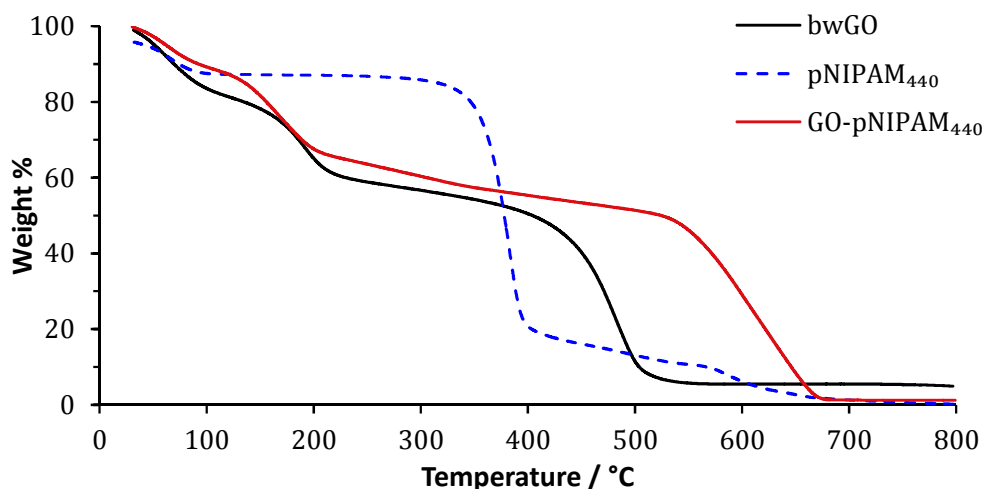
Figure 3 TGA profile of bwGO, pNIPAM 440 and GO-pNIPAM 440 .
