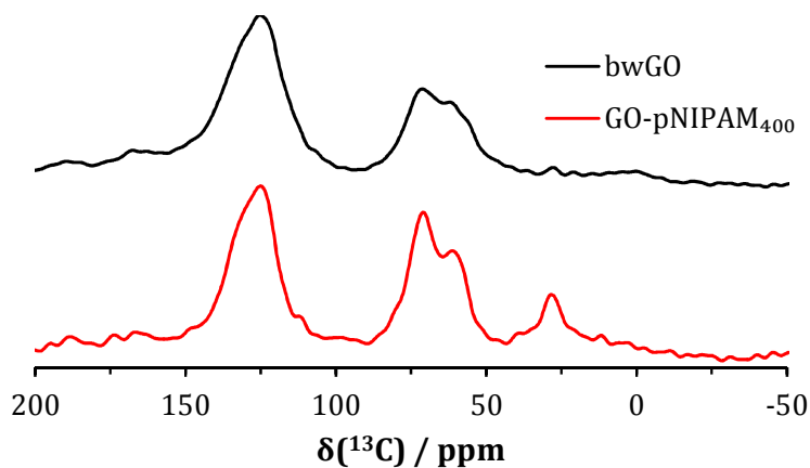
Figure 1 The direct excitation ^{13}\text{C} MAS ssNMR spectra of bwGO and GO-pNIPAM 440 .
