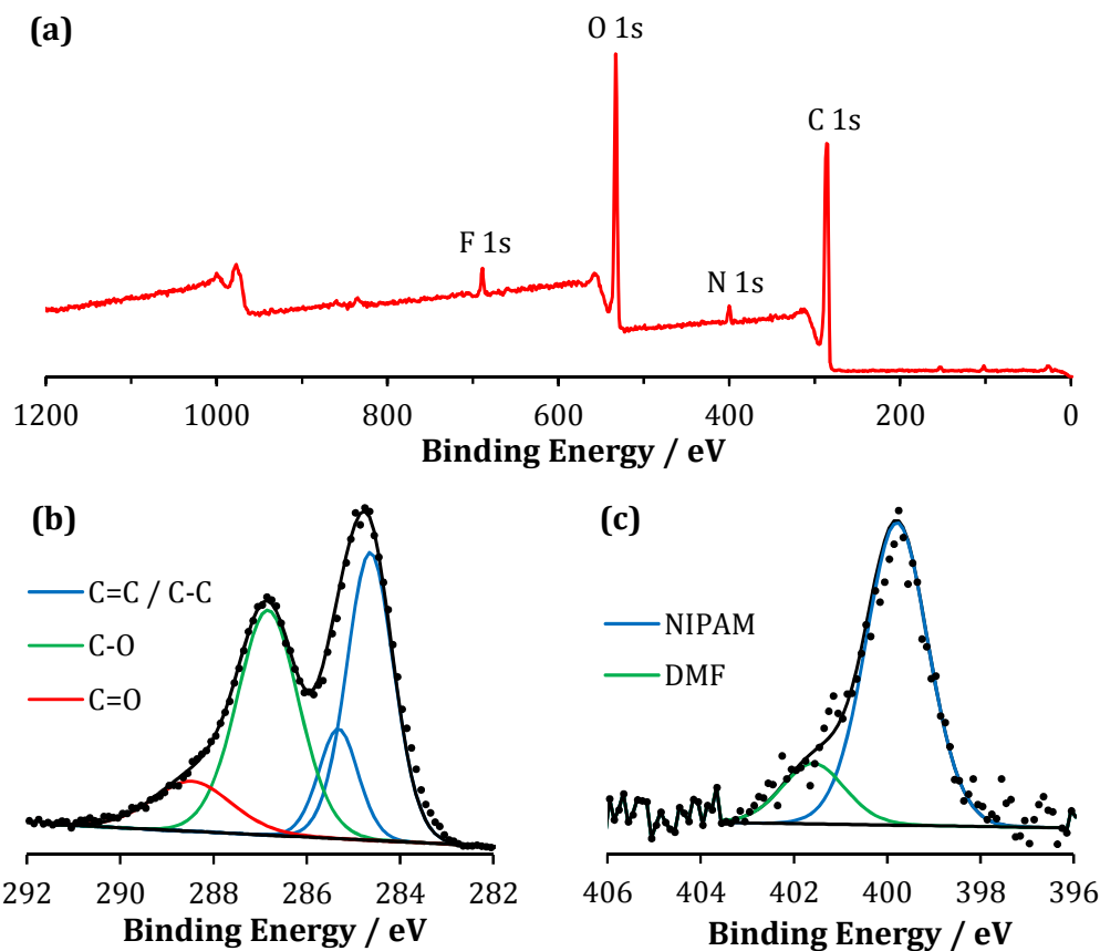
Figure 2 XPS analysis of GO-NIPAM 400 , complete with survey scan (a), and core level spectra C 1s (b) and N 1s (c). The experimental data is shown as points with the underlying lines showing the fitted peaks (assignments as labelled).
