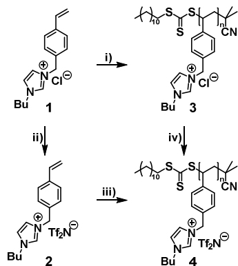
Scheme 1 Synthetic approach for the preparation of p([BVBIM]Cl) ( 3 ) and p([BVBIM]Tf 2 N) ( 4 ) from the monomers [BVBIM]Cl ( 1 ) and [BVBIM]Tf 2 N ( 2 ), respectively. Molar ratio [M]:[CTA]:[I] for i) 200:1:0.2 and for iii) 200:1:0.2 (i: RAFT polymerization; ii: Tf 2 N - vs. Cl - anion exchange; iii: RAFT polymerization; iv: anion exchange).
