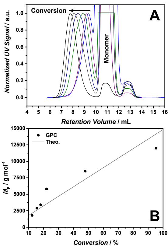
Fig. 2 (A) Molecular weight evolution of the RAFT polymerization of p([BVBIM]Tf 2 N) ( 4 ) at 85 °C in butyronitrile. (B) Molecular weight evolution ( M_p ) with conversion for the RAFT mediated polymerization of ( 2 ). Molar ratio [M]:[CTA]:[I] 200:1:0.2, 85 °C, butyronitrile (CTA: 2-cyano-2-propyl dodecyl trithiocarbonate; I = 1,1'-azobiscyclohexane carbonitrile). THF-SEC system conditions: 10 mmol LiTf 2 N, 10 mmol n -butylimidazole, 35 °C, flow rate 1.0 mL·min -1 .
