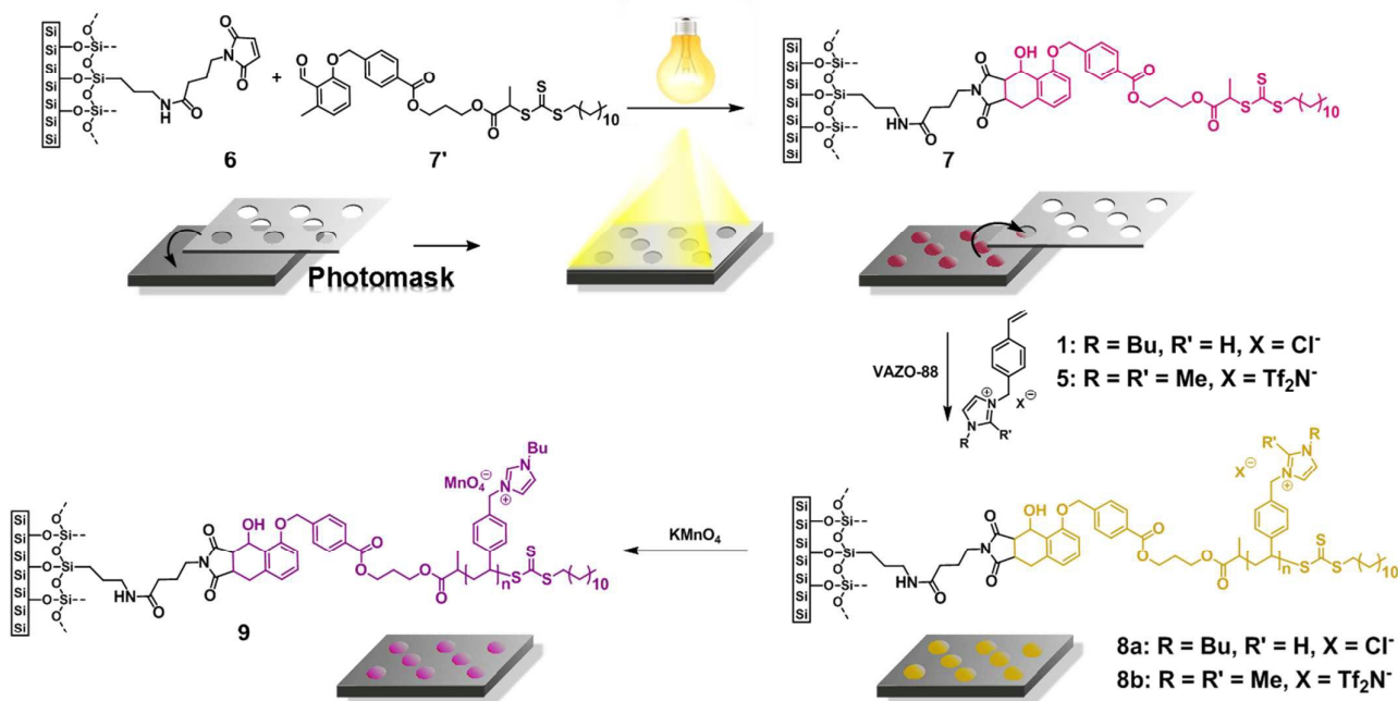
Fig. 7 Schematic illustration of the surface functionalization for the spatially resolved surface functionalization of silicon wafers with ( 1 ) and ( 5 ). (3-Aminopropyl)triethoxysilane (APTES)-coated silicon wafers were coated with 4-maleimidobutyryl chloride to achieve maleimide-functionalized surfaces ( 6 ). After irradiation, the surfaces covered with a photomask with an ARIMED B6 lamp ( \lambda_{max} = 320 nm) in a solution of the photoenol functional CTA to result in ( 7 ) followed by RAFT polymerization of ( 1 ) from the surface. Subsequent salt metathesis of ( 8a ) with KMnO 4 resulted in a highly violet colored meander pattern of p([BVBIM]MnO 4 ) ( 9 ).
