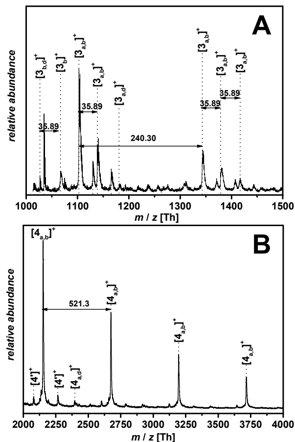
Fig. 4 Zoom of the MALDI-ToF spectrum of (A) p([BVBIM]Cl) ( 3 ) ( M_w = 1900 \text{ g}\cdot\text{mol}^{-1} ) and (B) p([BVBIM]Tf 2 N) ( 4 ) in the representative area of the mass spectrum with the assigned peaks employing DCTB as matrix material, respectively. Please refer to Table S2 and S3 in the Supporting Information for the list of assignments.
