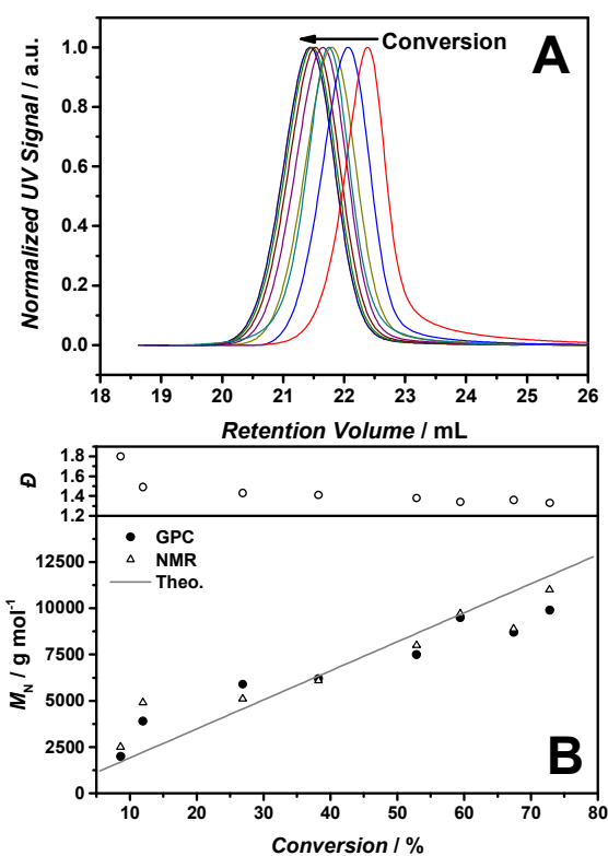
Fig. 1 (A) GPC traces of p([BVBIM]Cl) ( 3 ) via the RAFT mediated polymerization of [BVBIM]Cl ( 1 ) at 85 °C in DMSO. (B) Plot of molecular weight ( M_n ) and dispersity ( \bar{D} ) vs. monomer conversion. Molar ratio of monomer:CTA:initiator 200:1:0.2 (CTA = 2-cyano-2-propyl dodecyl trithiocarbonate; initiator = 1,1'-azobis(cyclohexanecarbonitrile)). H 2 O-SEC system conditions: water/0.3 M formic acid/0.5 g·L -1 NaCl, 30 °C, flow rate 1.0 mL·min -1 .
