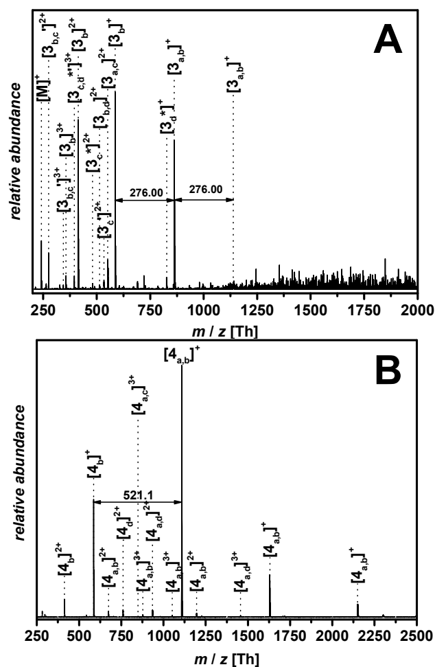
Fig. 6 Zoom of ESI-MS spectra of A) p([BVBIM]Cl) ( 3 ) with a molecular weight of M_w = 1900 \text{ g}\cdot\text{mol}^{-1} measured in THF/MeOH (3:2, v/v) and B) p([BVBIM]Tf 2 N) ( 4 ) measured in a mixture of acetonitrile/water (1:1, v/v). Please refer to the Supporting Information for a list of the assignments (Table S4 and S5).
