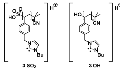
Fig. 5 Chemical structures assigned in the MALDI spectrum of p([BVBIM]Cl) ( 3 ) ( M_w = 1900 \text{ g}\cdot\text{mol}^{-1} ). PIL structure with a sulfonic acid endgroup and a hydroxyl endgroup. 37 The m/z difference of both peaks originates from the loss of \text{SO}_2 .
