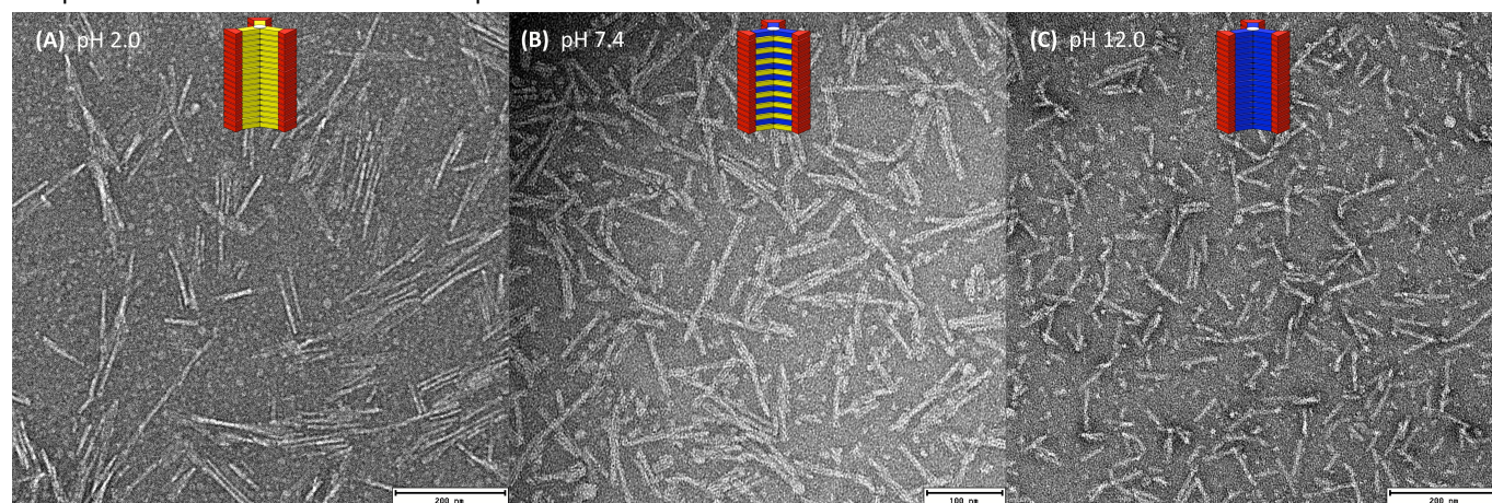
Figure 4. (A) TEM images of the homopolymer of 1a at pH 2.0, (B) the 1a-1b copolymer at pH 7.4 and (C) the homopolymer of 1b at pH 12.0, in tris buffer (10 mM); scale bars are 200 nm (A), (C) and 100 nm (B).
