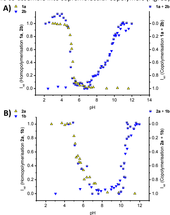
Figure 5. Titration experiments of 60 \mu M aqueous solutions of monomers in 10 mM phosphate buffer at 293 K; (A) the titration curves for the homopolymerisation of an isolated solution of 1a (yellow triangles, Fig. 2A) and 2b (blue triangles, Fig. S4B) and the 1a-2b copolymers (mixed yellow-blue squares, Fig. S3A); (B) the titration curves and normalised CD data for the homopolymerisation (left y-axis) of an isolated solution of 2a (yellow triangles, Fig. S4A) and 1b (blue triangles, Fig. 2A) and the 1b-2a copolymers (mixed yellow-blue squares, right y-axis, Fig. S3B), following the intensity of the CD band at \lambda = 216 nm in all cases, except for the 1b-2a copolymer ( \lambda = 237 nm); I_{rel} = 1 is set for the polymerized state as 'on' and I_{rel} = 0 is set for the polymerized state as switched 'off'.
