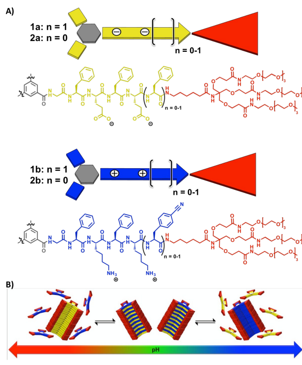
Figure 1. Chemical structures of the C 3 -symmetrical dendritic peptide comonomers 1a , 1b and 2a , 2b (A) and their pH-regulated supramolecular polymerization into copolymers at neutral pH, and homopolymers at high and low pH respectively (B).
