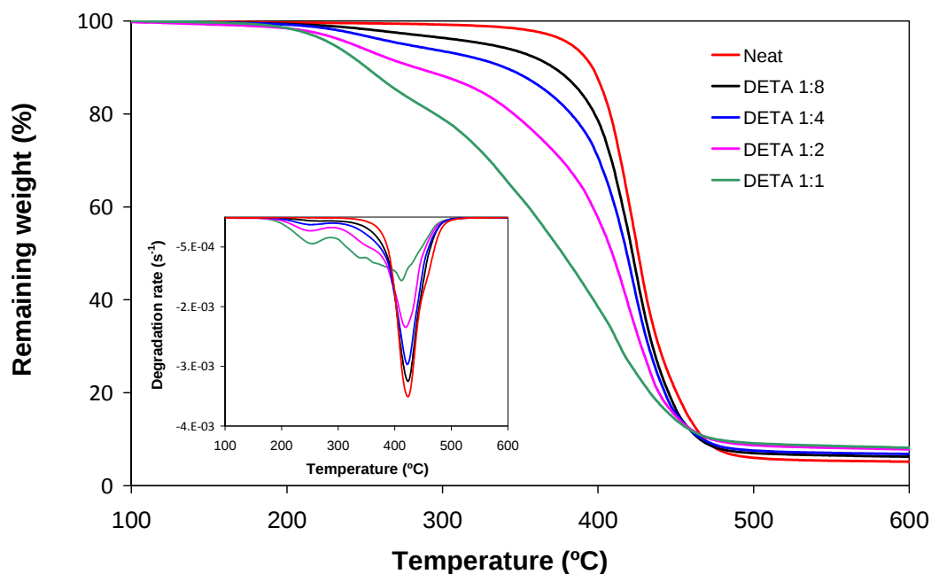
Figure 4. Thermogravimetric curves at 10°C/min in nitrogen atmosphere of dual cured BGDA25/HDDA75 formulations with a 3wt.% of DMPA as photoinitiator and different molar ratio of DETA/acrylate, indicated in the legend.
