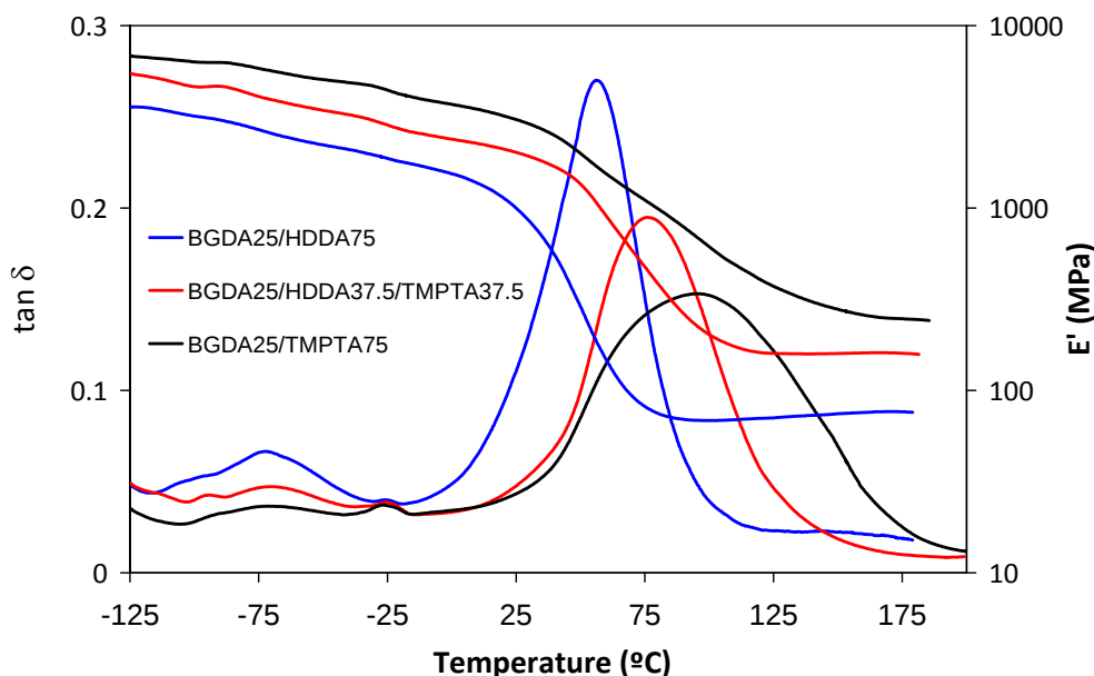
Figure 5. Storage moduli and \tan \delta curves against temperature of dual cured DETA 1:4 formulations with a 3wt.% of DMPA as photoinitiator and different amounts of BGDA, HDDA and TMPTA, indicated in the legend.
