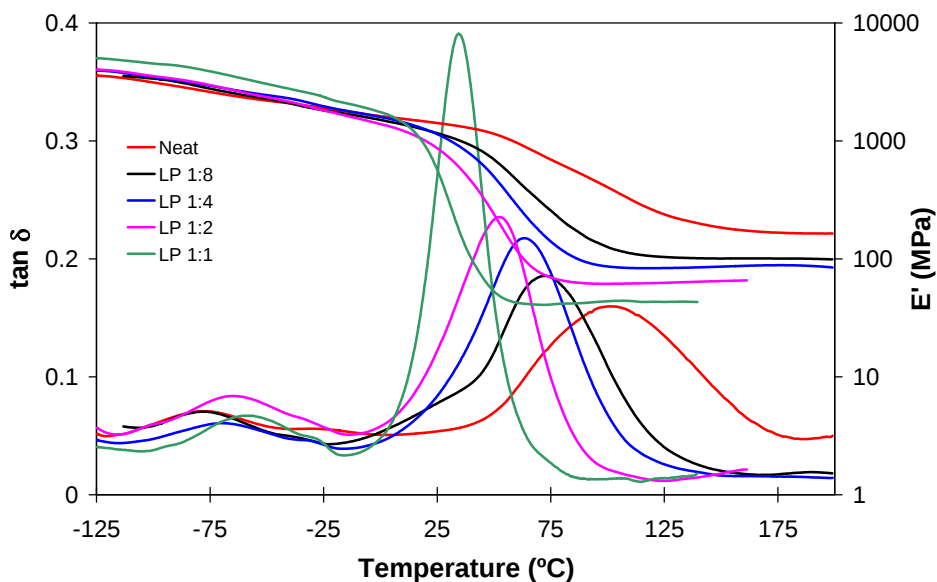
Figure 2. Storage moduli and \tan \delta curves against temperature of dual cured BGDA25/HDDA75 formulations with a 3wt.% of DMPA as photoinitiator and different molar ratio of LP/acrylate, indicated in the legend.
