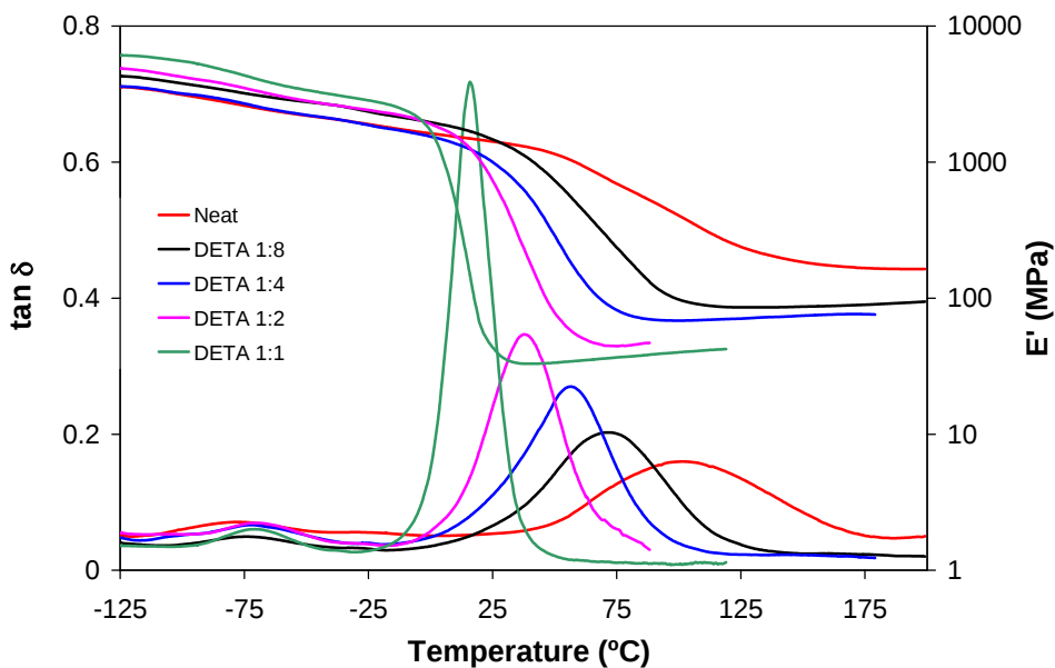
Figure 3. Storage moduli and \tan \delta curves against temperature of dual cured BGDA25/HDDA75 formulations with a 3wt.% of DMPA as photoinitiator and different molar ratio of DETA/acrylate, indicated in the legend.
