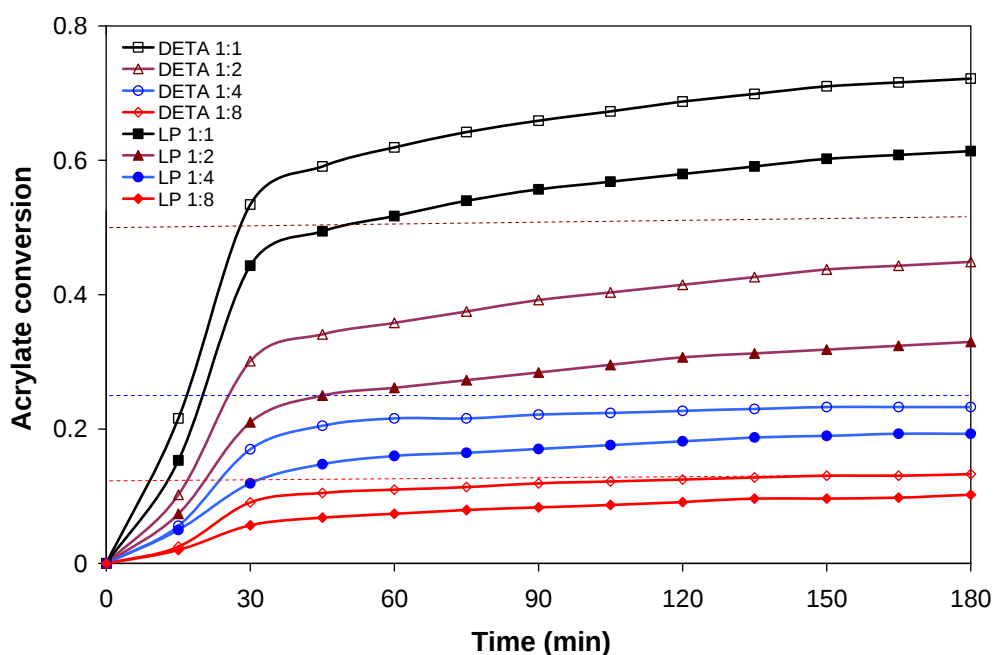
Figure 1. Acrylate conversion (from FTIR/ATR experiments) during aza-Michael addition (first curing stage) against time obtained by isothermal reaction at 35°C of BGDA25/HDDA75 formulations with a 3wt.% of DMPA as photoinitiator and different molar ratio of LP and DETA, indicated in the legend. Horizontal dashed lines indicate the maximum acrylate conversion if aza-Michael addition would be completed for 1:8, 1:4 and 1:2 formulations.
