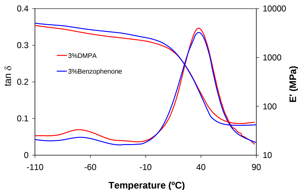
Figure 6. Storage moduli and \tan \delta curves against temperature of dual cured DETA/BGDA25/HDDA75 1:2 formulations with 3% of DMPA and 3% of benzophenone as photoinitiator.
