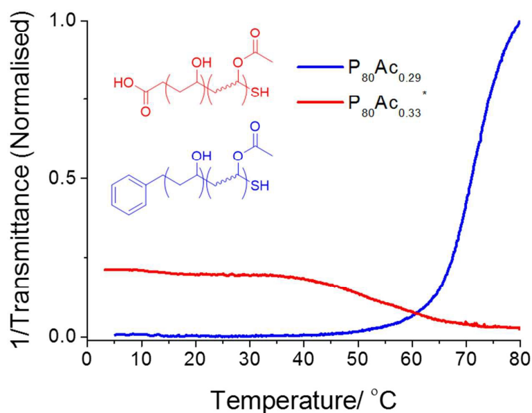
Figure 4. Turbidimetry curves showing the cloud point behaviour of P_{80}Ac_{0.29} and P_{80}Ac_{0.33}^* with hydrophobic and hydrophilic end groups at 10 \text{ mg.mL}^{-1} .
