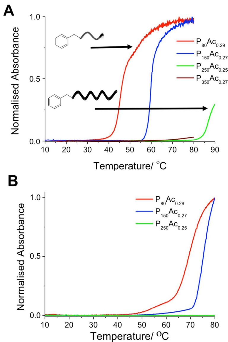
Figure 3. (A) Turbidimetry curves showing the molecular weight dependent cloud point behaviour of PVA(Ac) statistical copolymers with 30 mol% acetylation, at 30 mg.mL -1 . (B) Cloud point behaviour of PVA(Ac) statistical copolymers with 30 mol% acetylation, at 10 mg.mL -1 .
