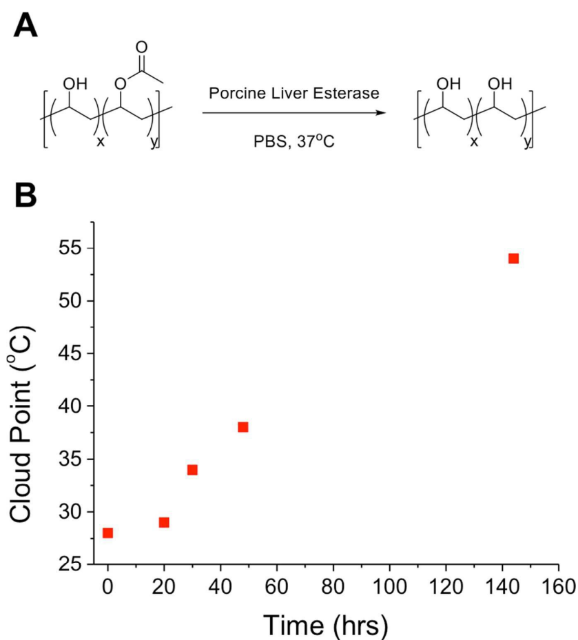
Figure 6. (A) Hydrolysis of acetate functionality of P_{350}Ac_{0.7} using Porcine Liver Esterase in PBS solution. (B) The cloud point behaviour of P_{350}Ac_{0.7} after addition of porcine liver esterase, showing increase in cloud point over time as acetate groups are enzymatically hydrolysed.
