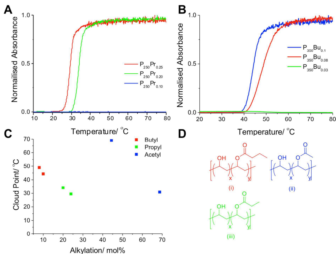
Figure 5. (A) Turbidimetry curves showing the cloud point behaviour of PVA.Propanoyl statistical copolymers at 10 \text{ mg.mL}^{-1} . (B) Turbidimetry curves showing the cloud point behaviour of PVA.Bu copolymers at 10 \text{ mg.mL}^{-1} (C) Comparison of cloud points (the temperature at 50% of normalised absorbance) of differently alkanoylated PVA copolymers. (D) Structures of statistical copolymers used in D (i) PVA.Butanoyl (ii) PVA.PVAc (iii) PVA.Propanoyl.
