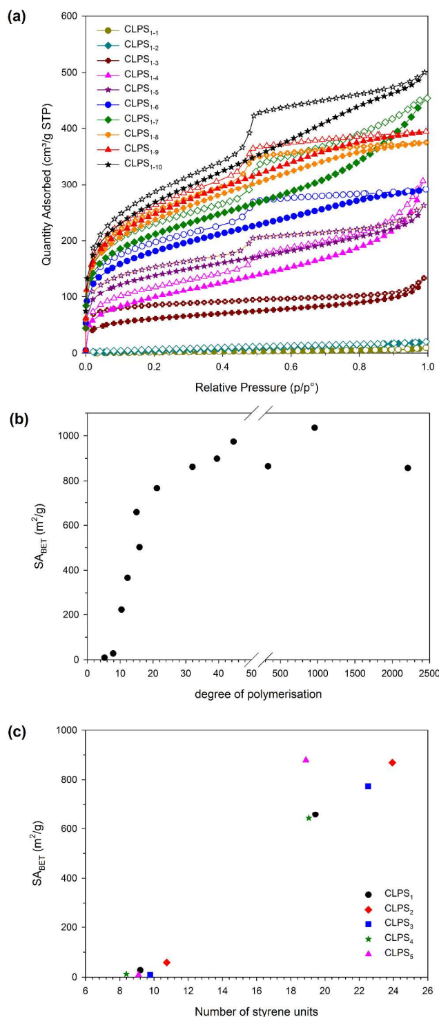
Figure 4. (a) Nitrogen isotherms of \text{CLPS}_{1-y} collected at 77 K. Adsorption (filled symbols), desorption (hollow symbols). (b) Plot of BET surface areas of \text{CLPS}_{1-y} against DP of the parent polystyrene. (c) Plot of BET surface areas of \text{CLPS}_{x-y} synthesised by different RAFT agent.
