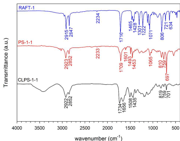
Figure 3. IR spectrum of \text{CLPS}_{1-1} , compared to that of \text{PS}_{1-1} and \text{RAFT-1} .
