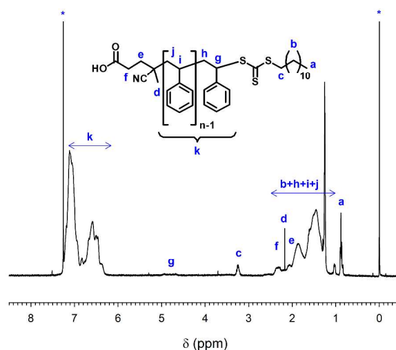
Figure 2. 1 H-NMR spectrum and assignment of PS 1-7 . Peaks marked with asterisks are due to CHCl 3 (7.27 ppm) and TMS (0.00 ppm).
