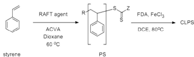
Scheme 1 Synthesis of hypercrosslinked polystyrene (CLPS)
