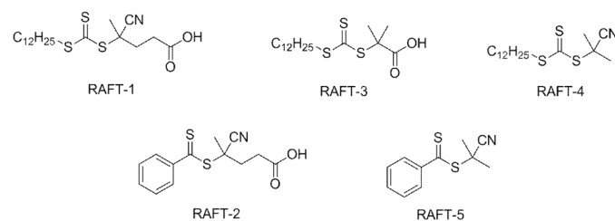
Figure 1. Structures of the RAFT agents used in this study.
