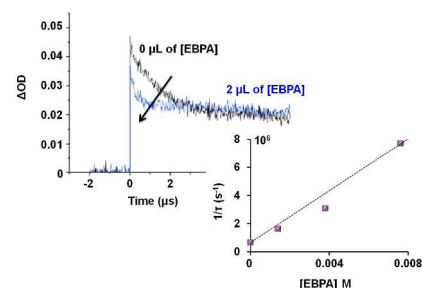
Figure 1 Laser flash photolysis. Decay of the [\text{1}]^{\text{II}*} signal at 390 nm in dichloromethane with increasing concentrations of 2 . The arrow shows that the \text{Au}_2^{\text{II}*} lifetime decreases as the concentration of 2 increases (from 0 to 7.6 \cdot 10^{-3} \text{ M} ). \Delta\text{OD} is the change in optical density associated with the light excitation ( \lambda = 355 \text{ nm} ).
