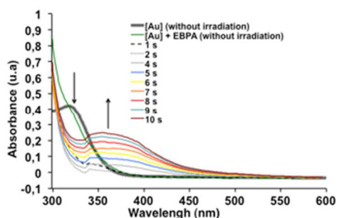
Figure 2 Steady state photolysis of 1 and 2 in dichloromethane upon exposure to the Xe-Hg under air at different irradiation times (from t = 0 to 10 s). 1/2 : 1/0.045. UV-vis spectra clearly demonstrate that one species disappears rapidly at very early stage and one appears.
