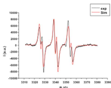
Figure 3. ESR spin trapping (PBN) spectrum. [\text{PBN}] = 7.90 \cdot 10^{-4} M, [\mathbf{1}] = 1.57 \cdot 10^{-4} M, [\mathbf{2}] = 1.91 \cdot 10^{-3} M in 1.5 mL of DCM/ tert -butylbenzene 1:2.
