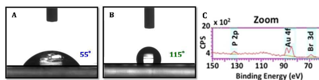
Figure 6 Contact angle experiments: Picture A) First layer: TPMTA/[Au 2 ]/EBPA: 1/0.0125/100 mol/mol after 3 minutes upon a blue LED bulb irradiation (405 nm). Picture B) Second layer after re-initiation with a fluoromonomer (HFBA 6 ) after 10 minutes upon a Xe-Hg lamp. Picture C) represents high resolution XPS spectra after re-initiation and formation of the fluorinated polymer.
