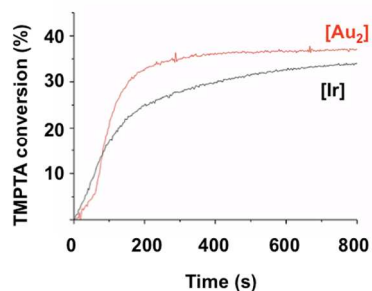
Figure 4 Compared polymerization profiles for TMPTA in laminate system for different catalysts upon a blue LED bulb irradiation (405 nm). Red curve: 2/5/1 (1/100/0.0125 mol/mol); black curve: 2/5/fac-Ir(ppy) 3 (1/100/0.0125 mol/mol).
