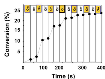
Figure 5 TMPTA conversion as a function of time for intermittent blue LED bulb irradiation. Polymerization was performed from 2/5/1 (1/100/0.0125 mol/mol) mixture.
