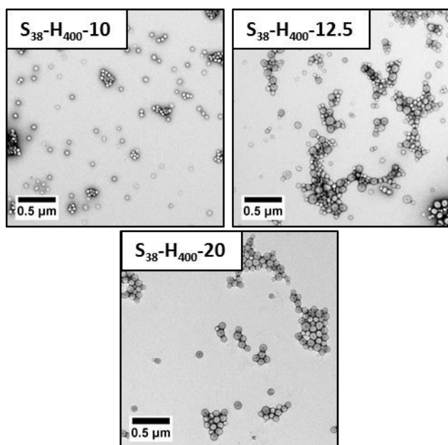
Figure 6. Representative TEM images obtained for \text{PSBMA}_{38}\text{-PPHMA}_{400} nanoparticles prepared at various solids contents. The copolymer morphology evolves from kinetically-trapped spheres (10 % w/w) to equilibrium vesicles (20 % w/w) via a spheres plus vesicles mixed phase (12.5 % w/w).
