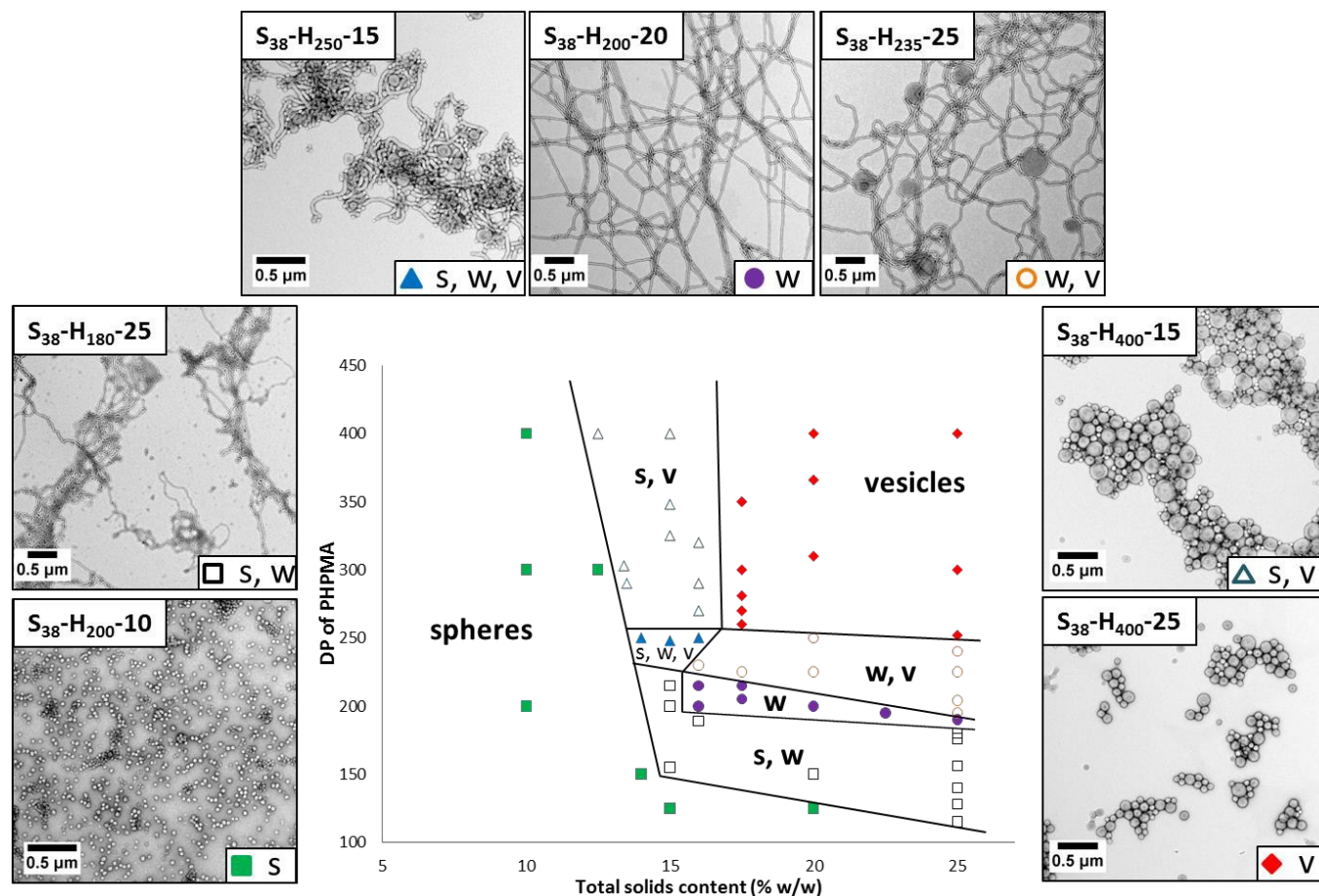
Figure 4. Detailed phase diagram constructed for the preparation of S_{38}\text{-H}_x\text{-Y} diblock copolymer nano-objects by RAFT aqueous dispersion polymerization of HPMA at 70 °C (for brevity, S denotes PSBMA and H denotes PHPMA). The target DP of the PHPMA block (x) and the total solids content (Y) were systematically varied and the diblock copolymer morphologies were assigned by post mortem TEM analysis of the final copolymer dispersions after appropriate dilution. Also shown are representative TEM images obtained for the various phases; S denotes spheres, W denotes worms and V denotes vesicles.
