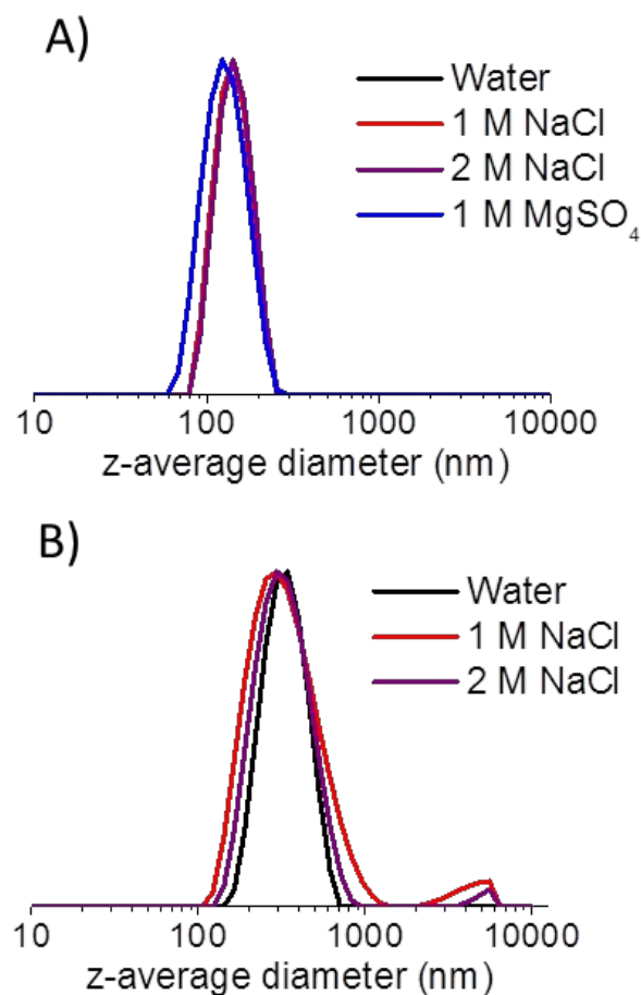
Figure 10. Intensity-average particle size distributions obtained by DLS for (a) S 38 -H 400 vesicles and (b) G 71 -H 400 vesicles after being aged in various aqueous salt solutions for one week.
