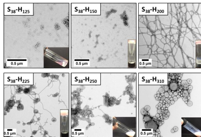
Figure 7. Representative TEM images obtained for \text{PSBMA}_{38}\text{-PPHMA}_x (denoted as S_{38}\text{-H}_x\text{-20} for brevity) nano-objects prepared by RAFT aqueous dispersion polymerization of HPMA at 70 °C at a total solids concentration of 20 % w/w. A digital photograph of the physical appearance of each copolymer dispersion is shown as an inset in each TEM image. The scale bar in each case is 0.5 μm. The tube inversion test confirms the formation of free-standing gels in three cases, whereas the other dispersions remained free-flowing.
