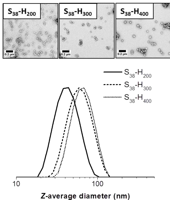
Figure 5. TEM images and corresponding DLS particle size distributions obtained for spherical S_{38}\text{-H}_x\text{-10} nanoparticles when x = 200, 300 or 400 .
