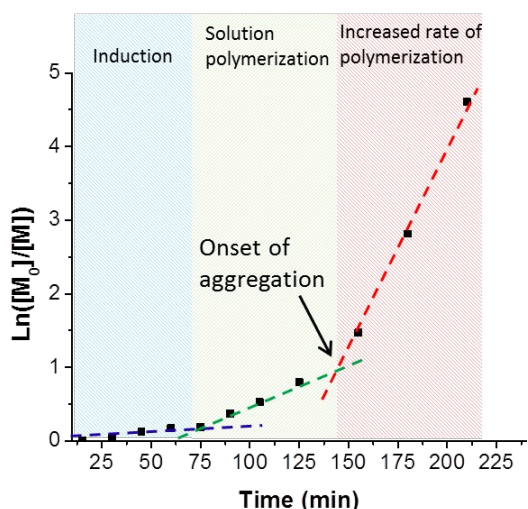
Figure 3. First-order kinetic plot for the RAFT aqueous dispersion polymerization of HPMA conducted using a PSBMA 38 macro-CTA in deionized water at 70 °C and 20 % w/w solids. Reaction conditions: [PSBMA 38 ]: [HPMA]: [ACVA] = 200: 1: 0.20. Three regimes can be identified: an induction period of approximately 75 min, a relatively slow rate of solution polymerization up to 145 min, and a relatively fast rate of dispersion polymerization after 145 min. The onset of micellization aggregation occurs at 150 min, which corresponds to a HPMA conversion of 67 % and equates to a PHPMA block length of 133.
