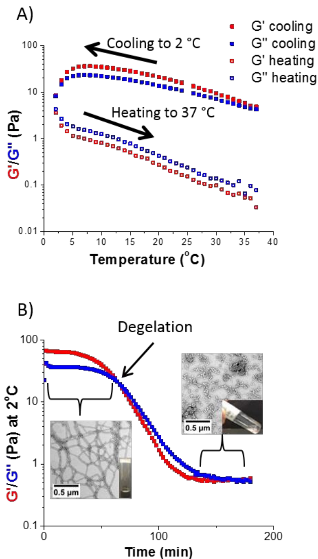
Figure 8. (A) Storage ( G' ) and loss ( G'' ) moduli recorded for a 10 % w/w S 38 -H 200 worm gel upon cooling from 37 °C to 2 °C followed by heating up to 37 °C. Irreversible degelation occurred at 2 °C. (B) Storage ( G' ) and loss ( G'' ) moduli recorded for a 10 % w/w S 38 -H 200 worm gel held at 2 °C for 200 min. Degelation occurred after 60 min at this temperature to produce a free-flowing liquid. TEM images recorded before cooling and 2 h after being held at 2 °C confirmed a worm-to-sphere transition. Both sets of measurements were conducted at 1.0 % applied strain using an angular frequency of 1.0 rad s -1 .
