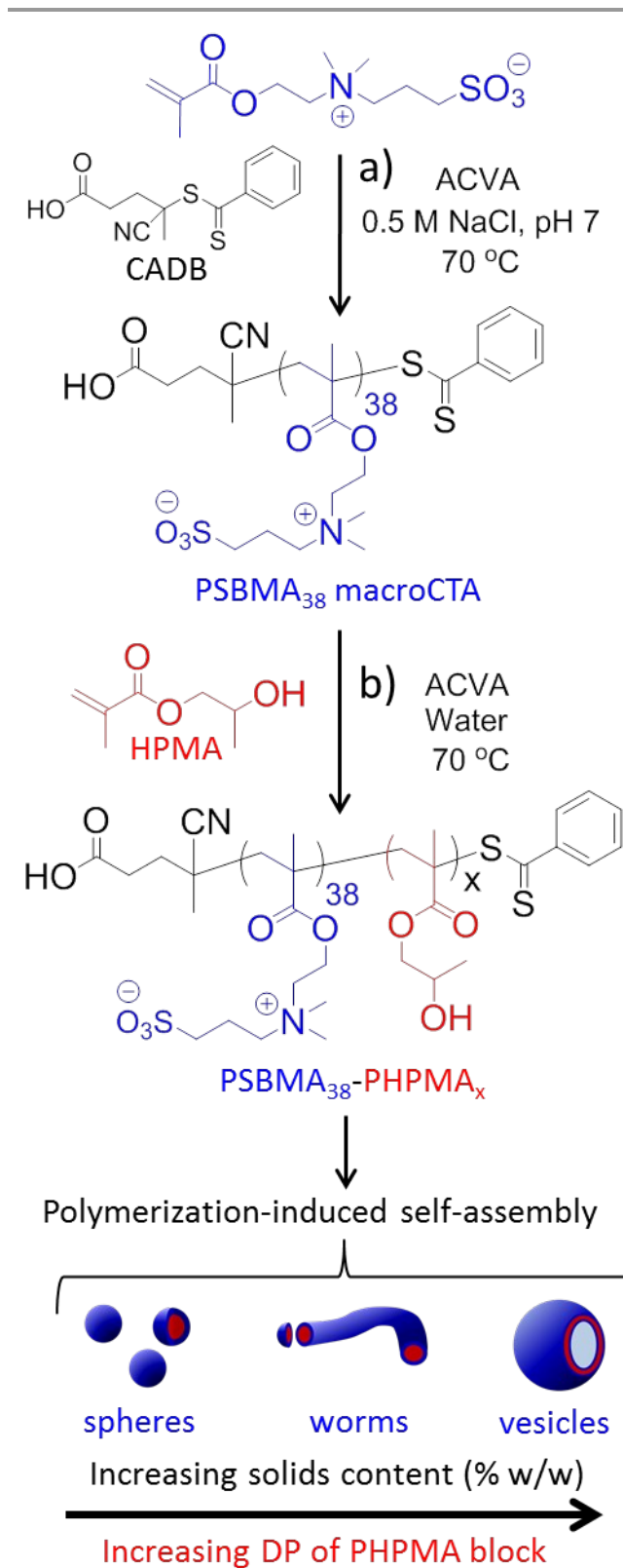
Figure 1. (a) Synthesis of the PSBMA 38 macro-CTA via RAFT aqueous solution polymerization of SBMA. (b) RAFT aqueous dispersion polymerization of HPMA using this PSBMA 38 macro-CTA at 70 °C to afford various PSBMA-HPMA diblock copolymer nano-objects via polymerization-induced self-assembly (PISA).
