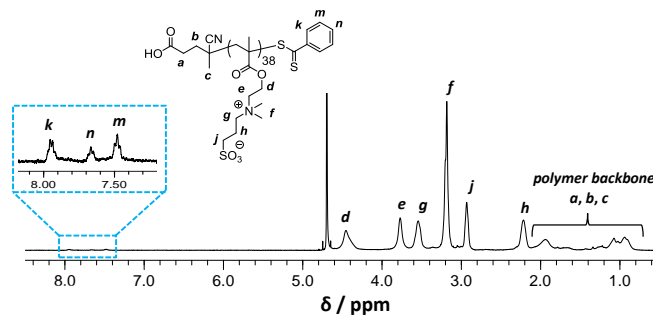
Figure 2. Assigned 1 H NMR spectrum recorded for PSBMA macro-CTA 1 in D 2 O.
