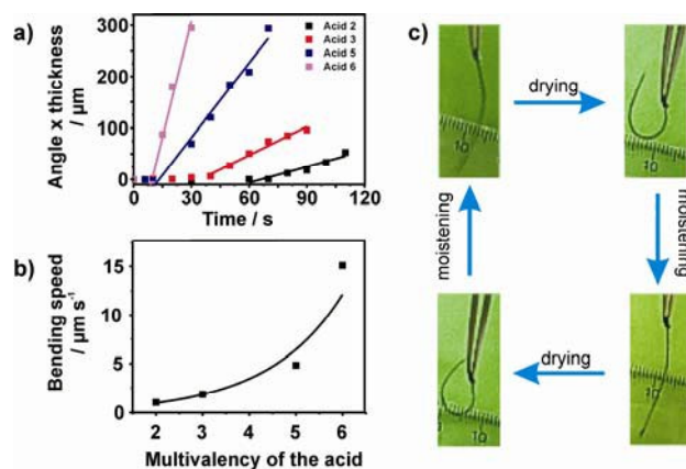
Figure 2: a) Plot of bending angle x membrane thickness vs. time for membrane actuators prepared from different acids. b) Bending speed derived from the slopes of b) vs. multivalency of the acid. c) On-off experiment, where a membrane from acid 6 was repeatedly dried and wetted.
