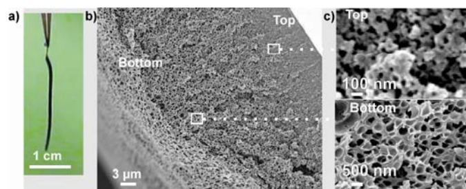
Figure 1: a) Photograph of a stripe-shaped membrane. b) Cross-section view of a porous PIL membrane prepared from PCMVPy-Tf 2 N with acid 3. c) An enlarged view of the same membrane on the top and at the bottom.
