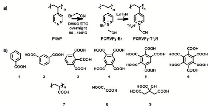
Scheme 1: a) Synthesis of polyvinylpyridinium-type PIL, PCMVPy-Tf 2 N by post-modification from poly(4-vinyl pyridine) (P4VP). b) Structures of the acids used for electrostatic complexation. ETG denotes ethylene glycol.
