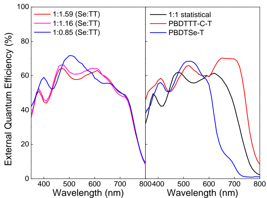
Figure 6 External quantum efficiency (EQE) spectra of devices of blocky (left), statistical and parent (right) polymers.
