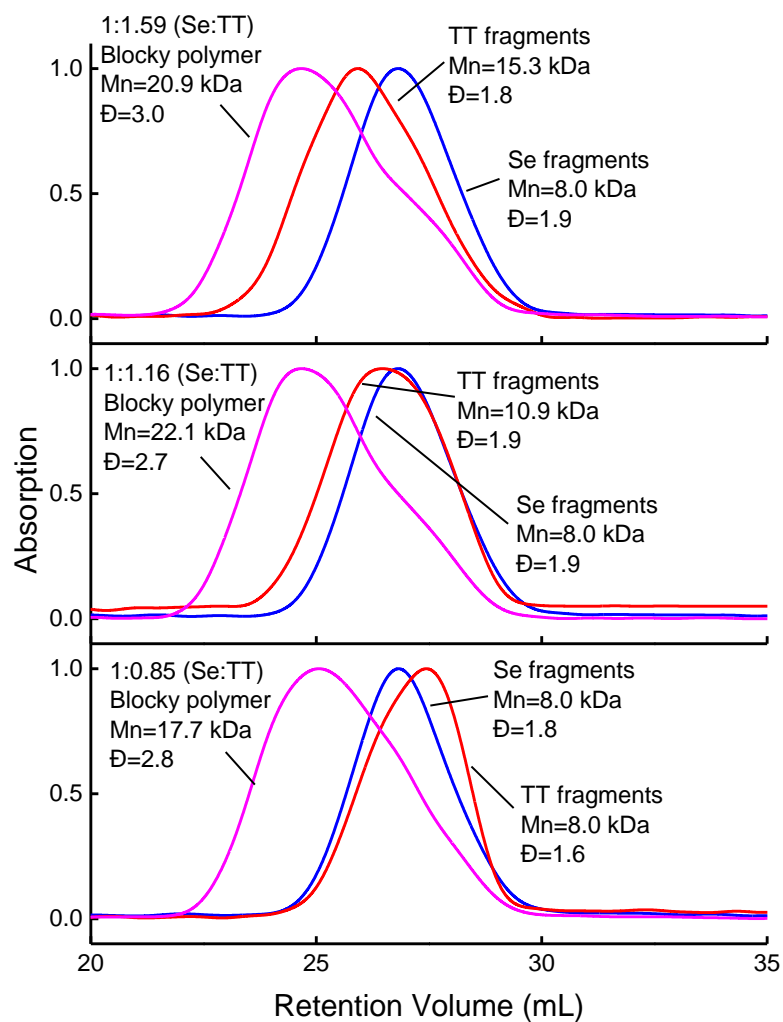
Figure 1 GPC elution profiles of blocky copolymers (magenta) and their PBDTSe-T (blue) and PBDTTT-C-T fragment reactants (red).
