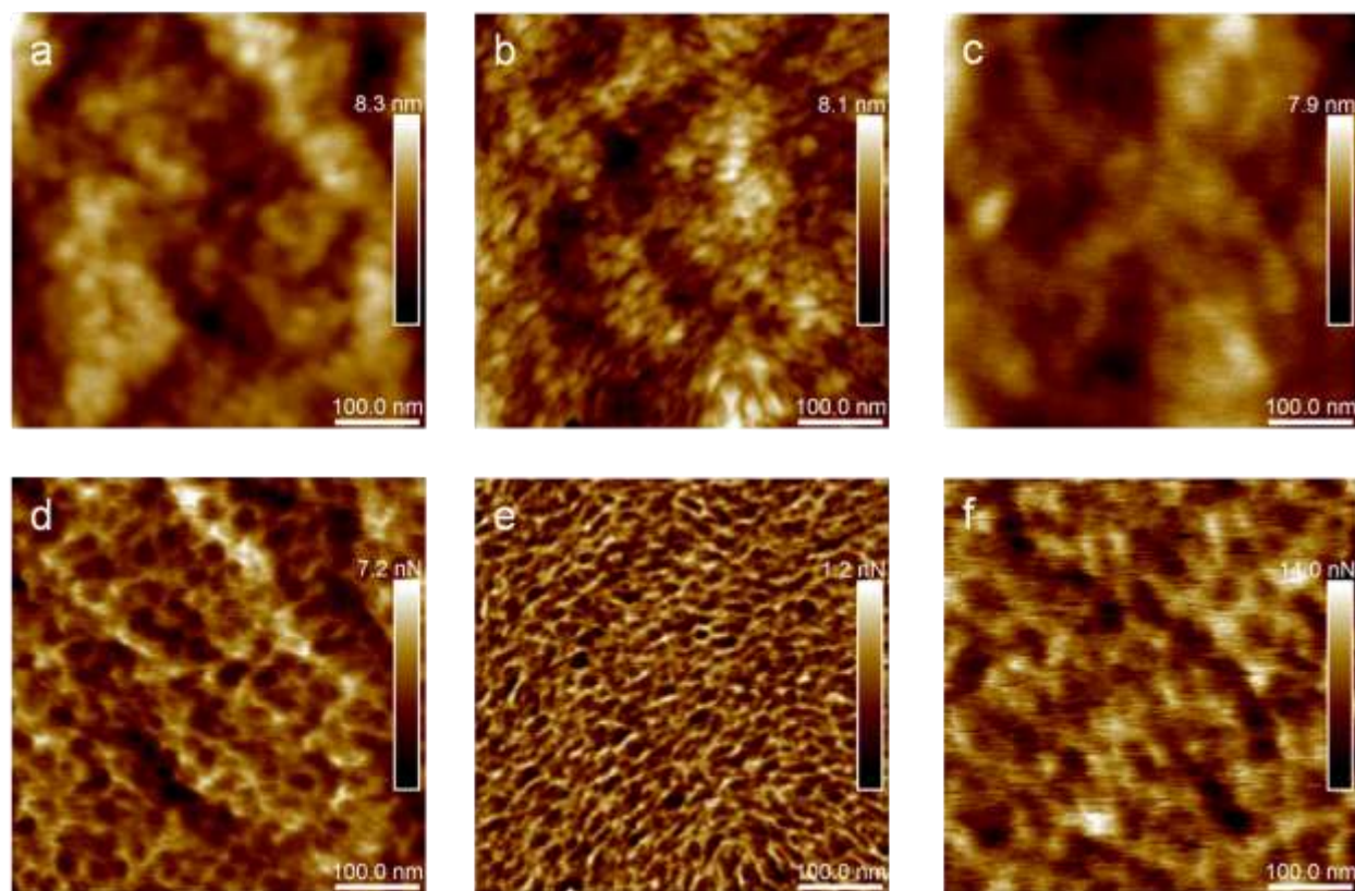
Figure 5 AFM height (above) and adhesion (below) images of 1:1.59 blocky (a,d), 1:1.16 blocky (b,e) and 1:0.85 blocky(c, f) polymer:PC 71 BM blend films.
