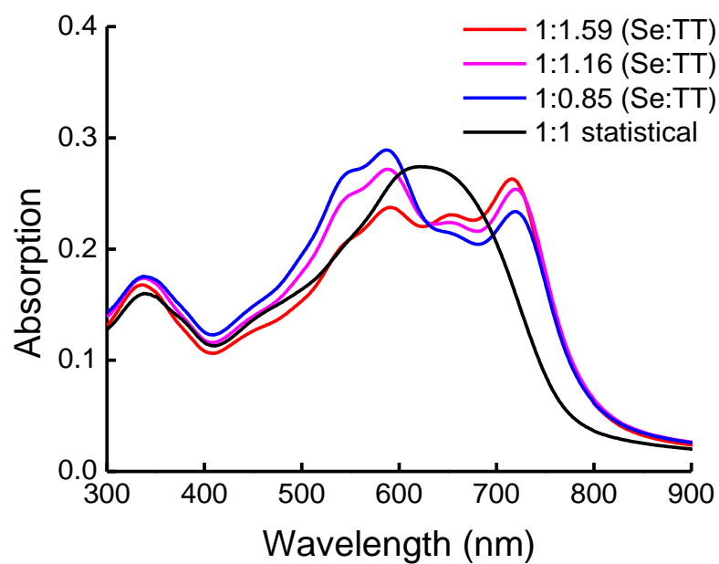
Figure 3 Absorption spectra of blocky and statistical polymer films spin-coated from chloroform solutions.
