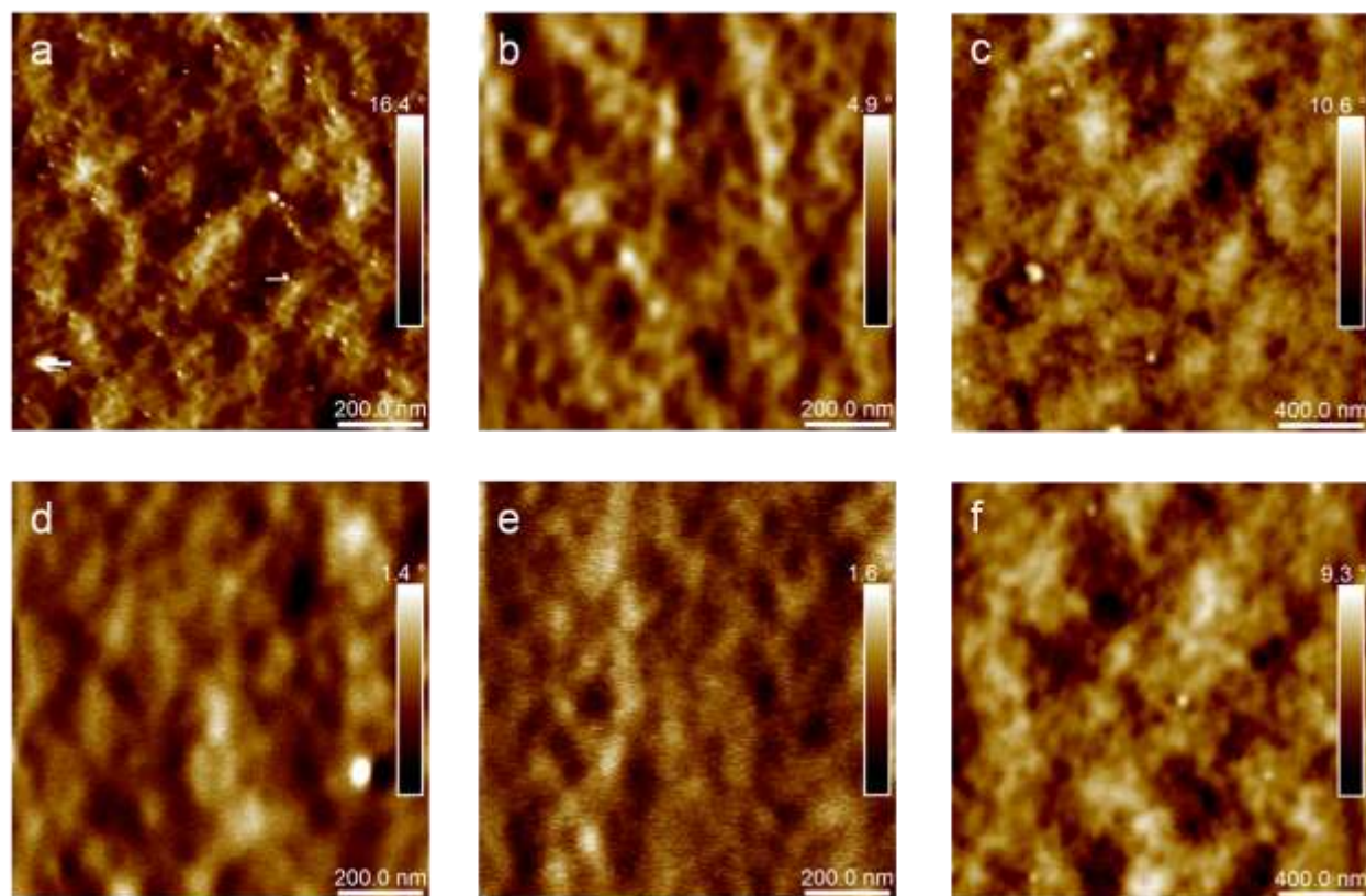
Figure 4 AFM phase images of 1:1.59 blocky (a), 1:1.16 blocky (b), 1:0.85 blocky (c), 1:1.59 physical mixture (d), 1:1.16 physical mixture (e) and 1:0.85 physical mixture (f) polymer:PC 71 BM blend films.
