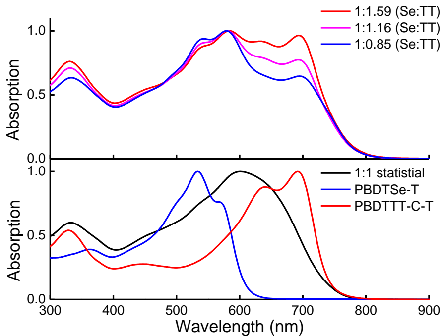
Figure 2 Normalized absorption spectra of blocky (above), statistical and parent (below) copolymers in chloroform.
