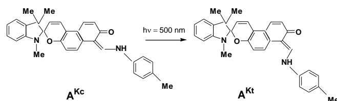
Scheme 9 Photochromic process in hydroxyazomethine fragment of BPC ( 1 ).
