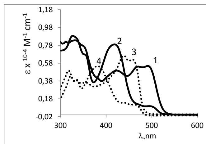
Fig.1 UV-vis absorption spectra of PBC (1) (curves 1, 2) and model (3) (curves 3, 4) in toluene (curves 2, 4) and methanol (curves 1, 3) solutions.
