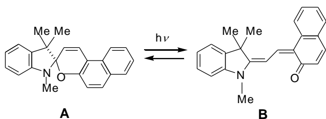
Scheme 7 Photochromic process in spironaphthopyran (4).
