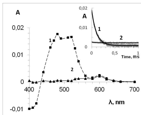
Fig.3. Visible absorption spectra of the intermediates produced by the 500 nm laser flash photolysis of BPC ( 1 ) in methanol solution in 0.05 \mu s (spectrum 1) and 1 ms (spectrum 2) after the laser pulse. Insert - decay kinetics of the intermediates, observed at 480 nm (1) and 600 nm (2) under flash photolysis of ( 1 ) with 500 nm light in MeOH.
