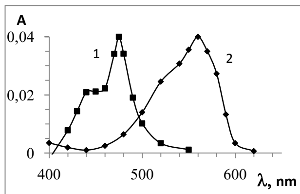
Fig.2 Visible absorption spectra of the intermediates produced by the 337 nm laser flash photolysis of (3) - (spectrum 1) and (4) - (spectrum 2) in methanol solution in 0.05 \mu s after the laser pulse.
