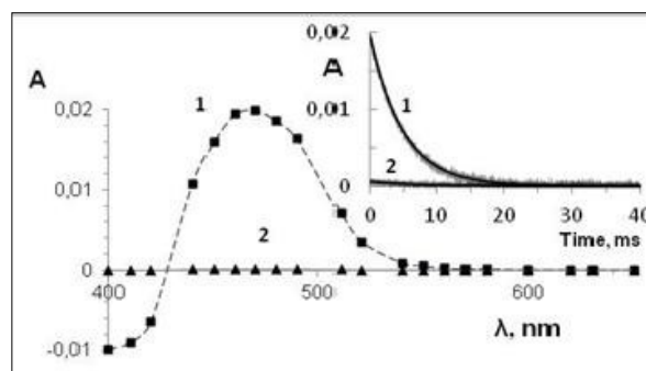
Fig. 4. Visible absorption spectra of the intermediates produced by the 500 nm laser flash photolysis of BPC (1) in toluene solution in 0.05 \mu\text{s} (1), and 30 ms after the laser pulse (2). Insert - decay kinetics of the intermediates, observed at 480 nm (1) and 600 nm (2) under laser flash photolysis of BPC (1) with 500 nm light in toluene
