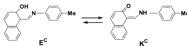
Scheme 5 Tautomeric forms of N-naphthylsalicylideneimine molecules
